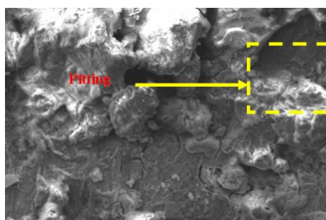
Figure 4. Pitting corrosion on tin surface
