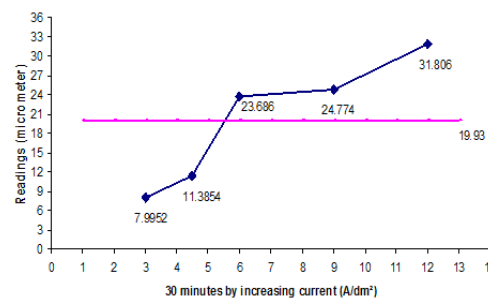
Figure 3. Graph for variables current density with 30 minutes coating
