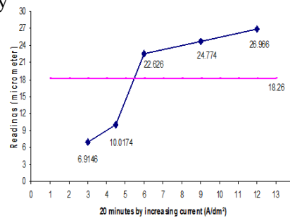
Figure 2. Graph for variables current density with 20 minutes coating
