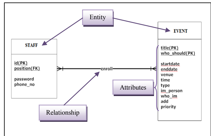
Figure 6. UTeM-EAS Entity Relationship Diagram
