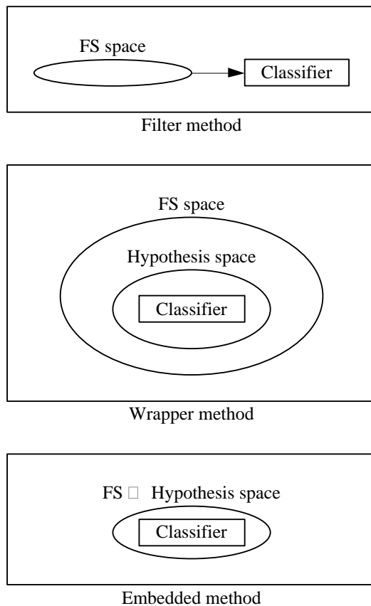
Figure 1. The model of feature selection methods
