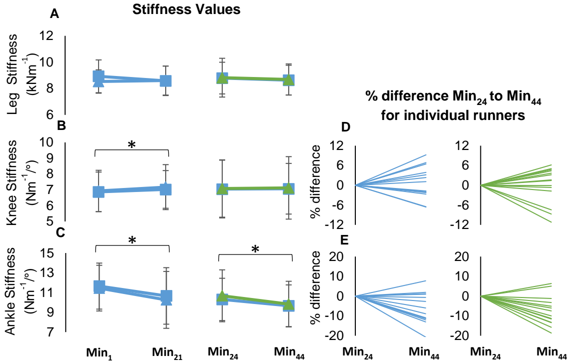
Figure 2: Leg, knee and ankle stiffness (A-C) throughout the PTR and individual % difference in knee and ankle stiffness from the start-end of the intervention run (D-E) in the neutral shoe (blue) and stability shoe (green) for sessions A (squares) and B (triangles). *Indicates main effect for time ( p < 0.05 ).
