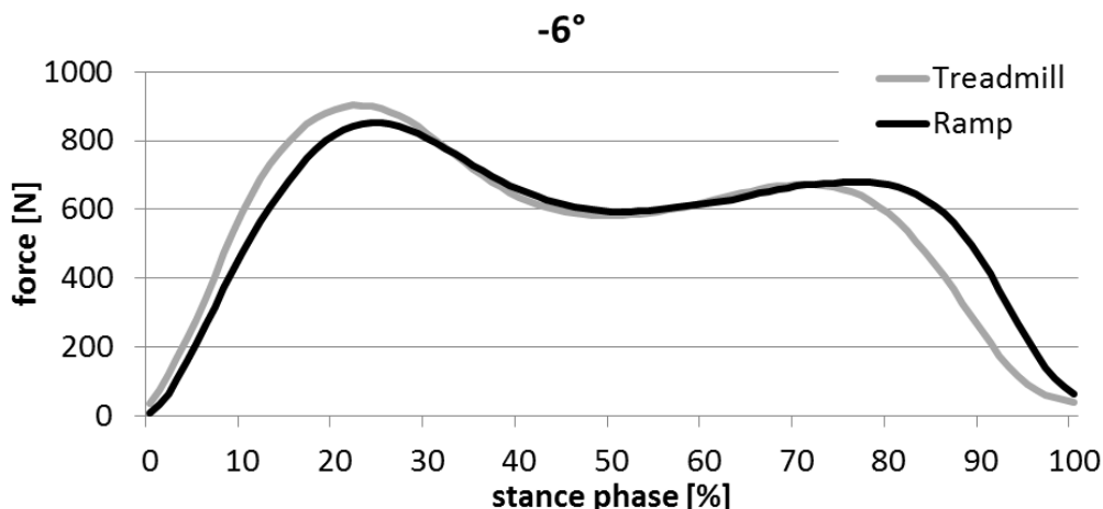
Figure 1: Loadsol forces during stance phase in 6° downhill walking on a treadmill and ramp construction during stance phase.
