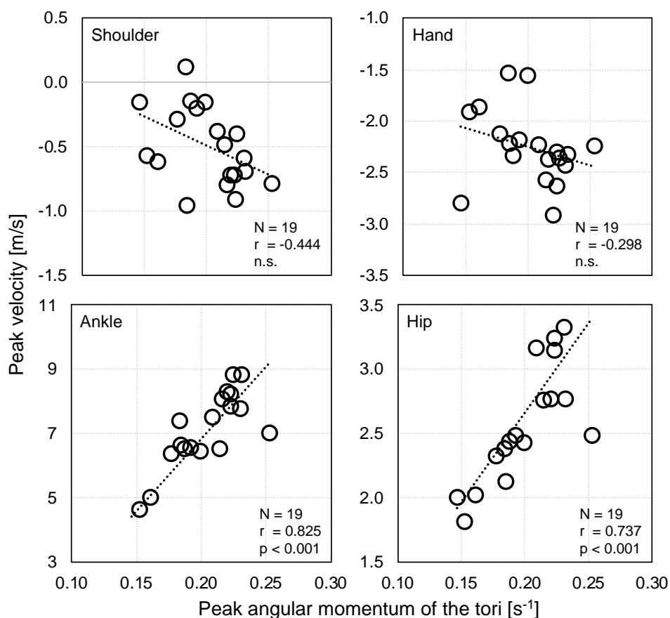
Figure 2: Relationship between normalized angular momentum of the tori and the peak velocity of the ankle, hip, shoulder and hand in the turning phase.
