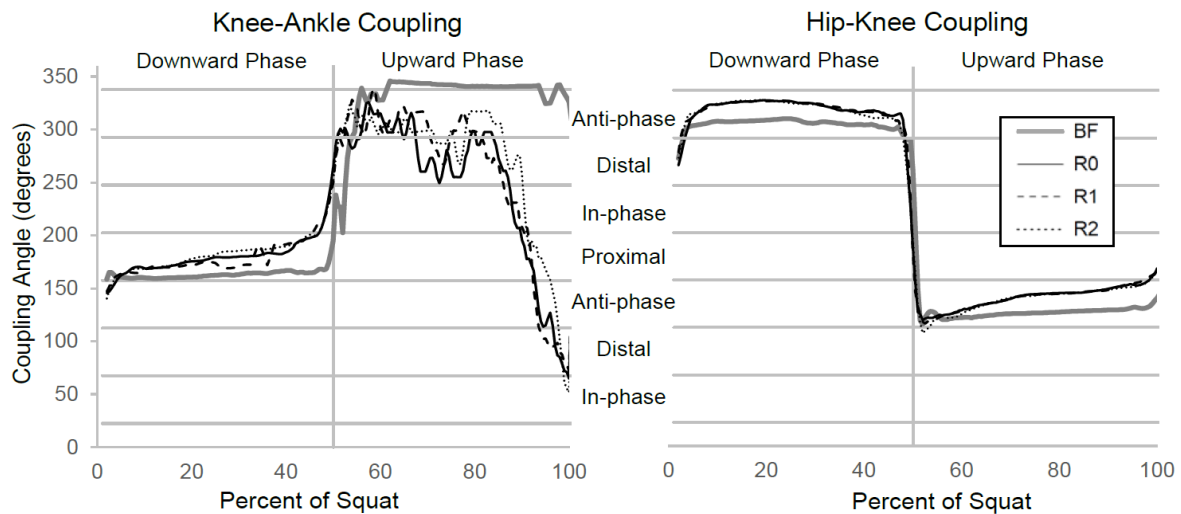
Figure 1. Average coupling angles of knee-ankle and hip-knee coordination during one squat are displayed for the non-dominant leg. The coupling pattern (movement driven by the distal joint, proximal joint, or in-phase/anti-phase joint contribution) is labelled for each angle range for which it is associated. Squat downward phase = 0 – 50%; upward phase = 51-100%. BF = barefoot; R0, R1, R2 = binding angles of 0°, 1°, and 2°, respectively.
