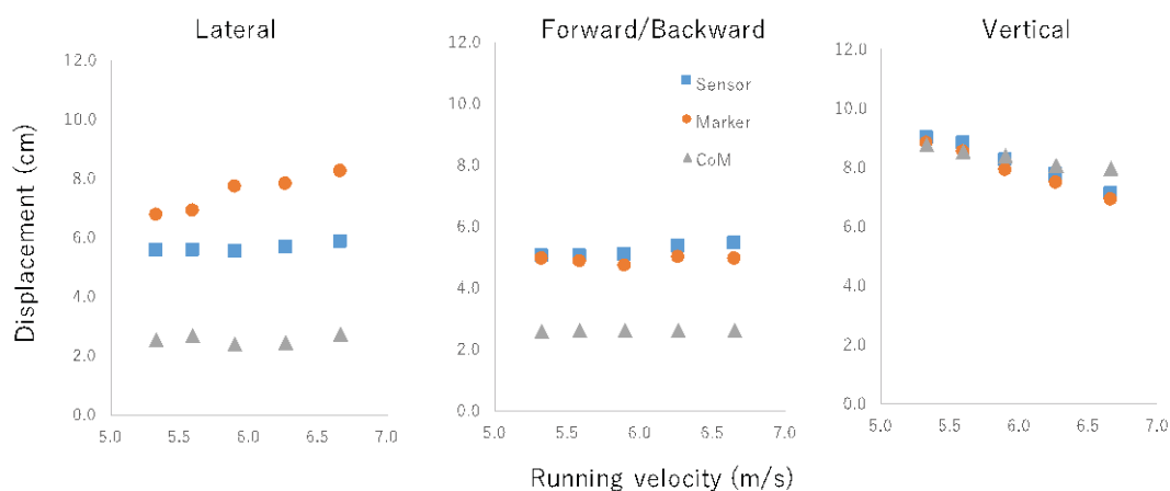
Figure 2 Lateral, forward/backward, and vertical displacement of Sensor, Marker, and CoM
