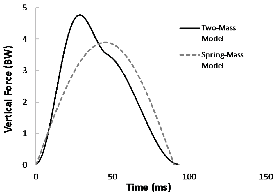
Figure 1: Kinematic-averaged sprint running ground reaction force-time waveforms generated by the two-mass and spring-mass models from 24 footfalls (n = 6 per athlete) at a mean running velocity of 11.7 meters per second.
