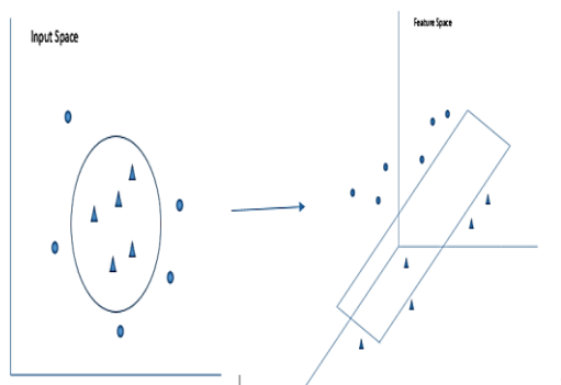
Gambar 2. Model Non-Linear Support Vector Machine
