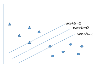
Gambar 1. Model Linier Support Vector Machine
