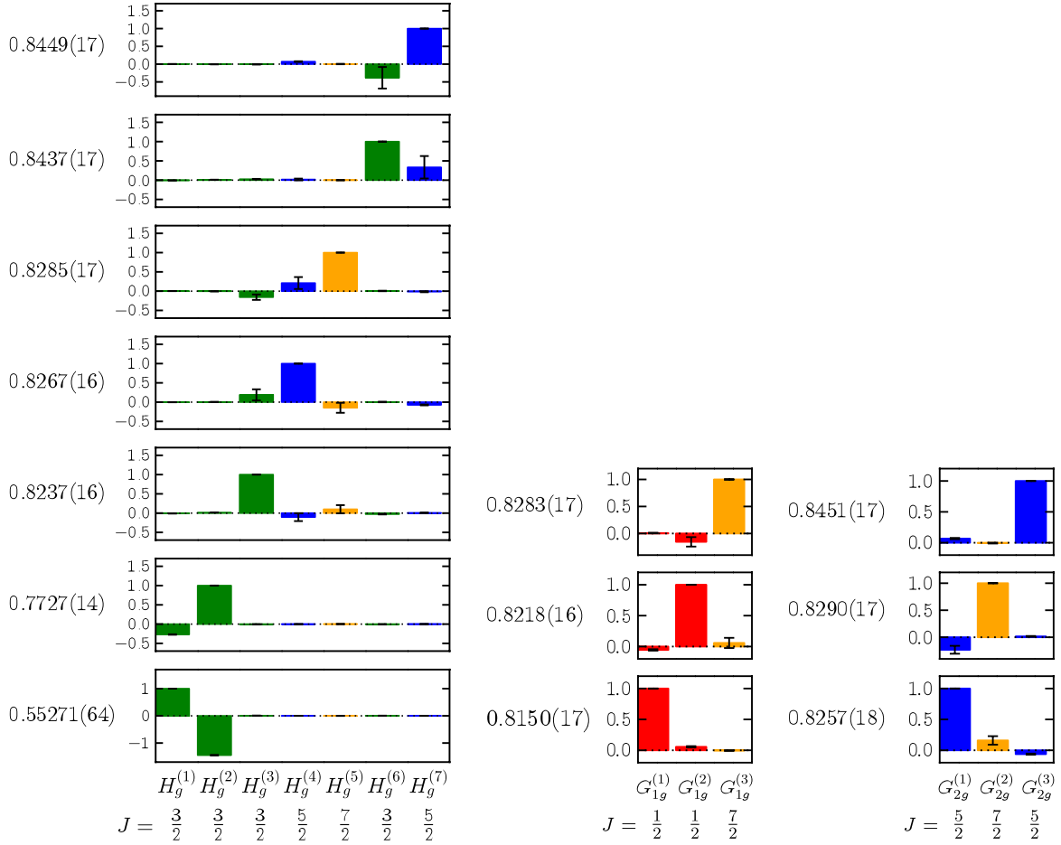
FIG. 4 (color online). Fitted energies E_n^{(\Lambda)} (in lattice units; from bottom to top: n = 1, \dots, N ), together with histograms of the corresponding relative overlap factors A_{n,i}^{(\Lambda)}/A_i^{(\Lambda)} [see Eqs. (29) and (30)]. The fits for the three different irreps were performed independently. For each i , the continuum angular momentum J from which the operator \Lambda^{(i)} was subduced is given at the bottom. These values of J are also indicated by the colors in the histograms (red: J = \frac{1}{2} ; green: J = \frac{3}{2} ; blue: J = \frac{5}{2} ; orange: J = \frac{7}{2} ). The data shown here are from the ensemble with a \approx 0.08 fm and am_{u,d} = 0.004 ; the fits have t_{\min}/a = 6 .
