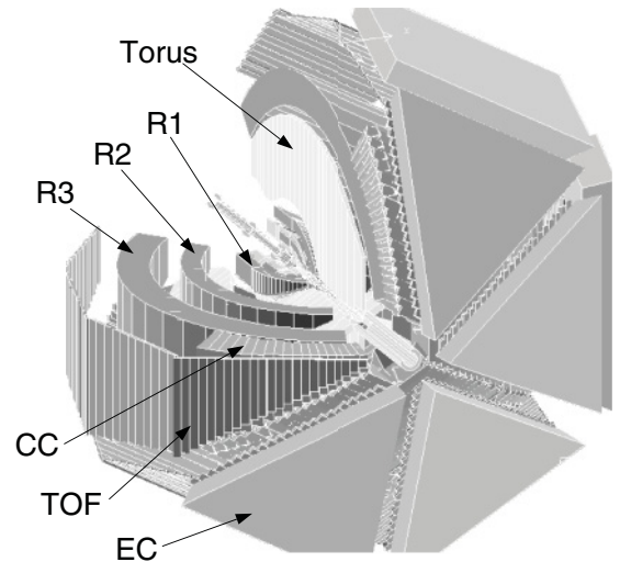
FIG. 1. Three-dimensional view of the CLAS, showing the three regions of drift chambers (R1–R3), Čerenkov counters (CC), the time-of-flight system (TOF), and the electromagnetic calorimeter (EC) (see text for details). In this picture, the photon beam travels from the upper-left corner to the lower-right corner.
