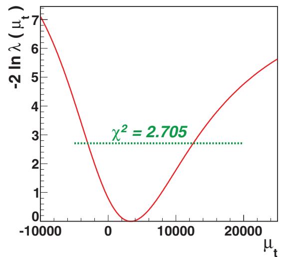
FIG. 10. (Color online) Illustration of determining the upper and lower limits for CL = 90%. The x axis is the expectation value for the measured quantity \mu . The red solid curve is the logarithm of the profile likelihood \mathcal{L} versus \mu_t , and the green dashed line is \chi^2 = 2.705 , corresponding to CL = 90%.
