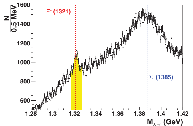
FIG. 4. (Color online) Invariant mass of the \Lambda\pi^- pairs. The red dashed and blue dotted lines mark the positions of the nominal mass for \Xi^-(1321) and \Sigma^-(1385) , respectively [4]. The shaded area shows the mass range used in this analysis.
