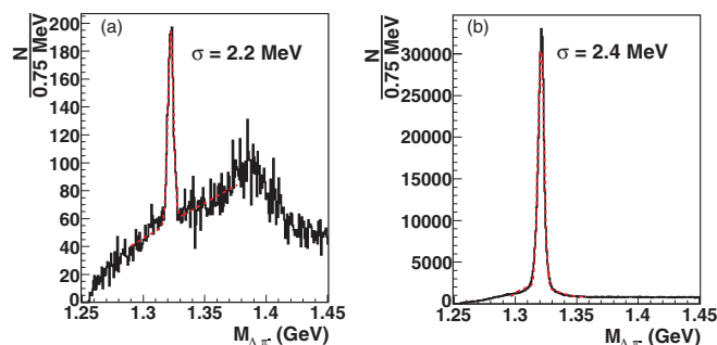
FIG. 7. (Color online) (a) Mass spectrum of \Lambda\pi^- from data using restrictive cuts (see text for details) and (b) \Lambda\pi^- mass from the GEANT-based simulations.
