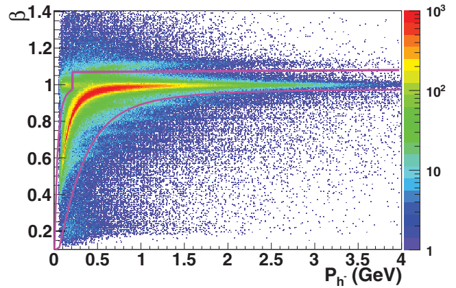
FIG. 3. (Color online) \beta versus momentum of the negative hadrons. The pions from decays of the \Lambda candidates are not included in this plot. The magenta lines indicate the \pi^- -identification cuts applied in this analysis.
