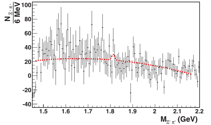
FIG. 6. (Color online) Number of \Xi^- \pi^- events per 6-MeV mass bin. The error bars indicate the statistical uncertainties. The dashed curve shows the fit to a Gaussian peak above a polynomial background. The center of the Gaussian in this plot is fixed at the center of the bin at 1.813 GeV.
