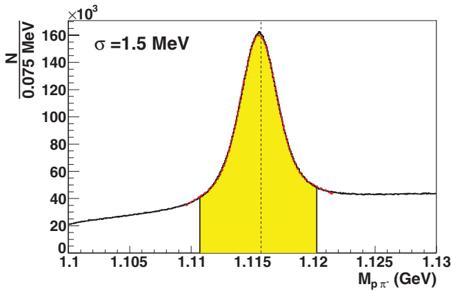
FIG. 2. (Color online) Mass spectrum of the p\pi^- system. The yellow (gray) shaded area indicates the mass range used in this analysis. The red curve is the fit to a Gaussian peak with a polynomial background. The dashed vertical line shows the PDG [4] value for the mass of \Lambda(1116) .
