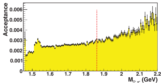
FIG. 8. (Color online) Acceptance of CLAS versus the invariant mass of the \Xi^-\pi^- system, determined from the \gamma d \rightarrow K^+K^+\Xi^-\pi^-p_s phase-space simulation using a GEANT-based detector simulation package GSIM. The red vertical line indicates the position of the peak seen by the NA49 collaboration.
