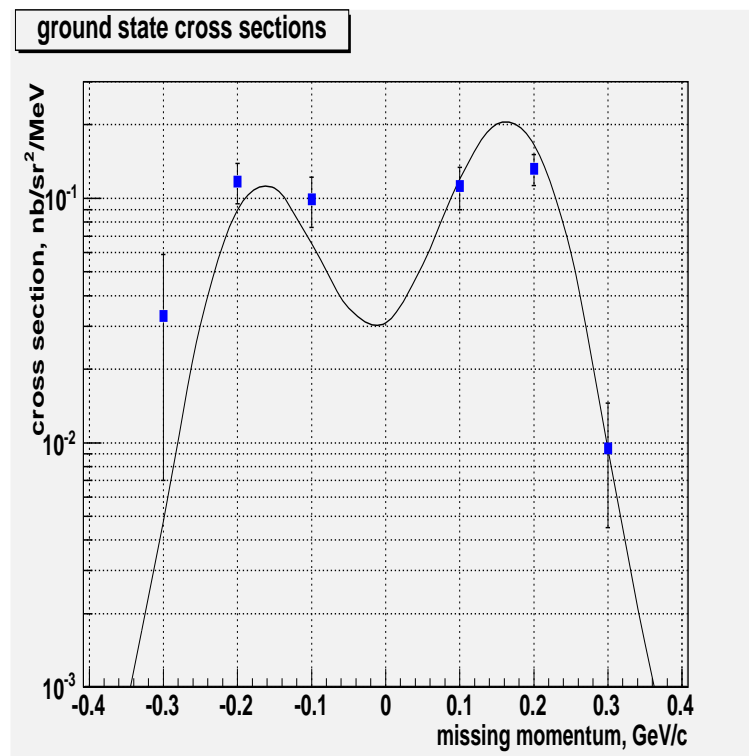
Figure 2. Absolute comparison of RDWIA theoretical prediction (solid line) vs data (squares) for the ground state cross section of the ^{209}\text{Bi}(e, e'p)^{208}\text{Pb} reaction. Theory assumes there is one proton in the 1h9/2 state in ^{209}\text{Bi} .
