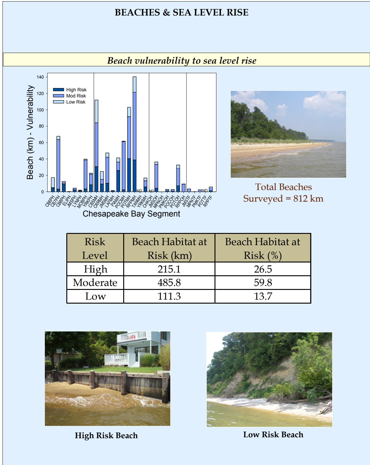
Figure 20. Estuarine beach vulnerability to sea level rise. There are approximately 812 km of beach habitat within 7134 km of surveyed shoreline in tidal Virginia. The highest abundance of beaches occurs within mesohaline reaches, and more than 85% of existing beaches are at high-moderate risk to sea level rise.
