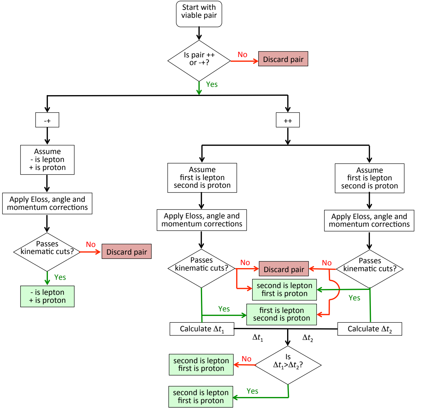
FIG. 11. (Color online) Flow chart showing the decision process in selecting elastic events. The green filled boxes correspond to identified elastic events.
