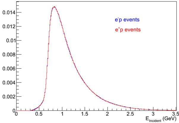
FIG. 13. (Color online) Reconstructed incident beam energy distributions of all elastic scattering events using scattering angles. The positron (red) and electron (blue) distributions have been scaled by the total number of counts in the distributions and show almost imperceptible differences. This figure differs from Fig. 7 in that it shows the incident energy distribution for elastic scattering events rather than the overall beam energy distribution.
