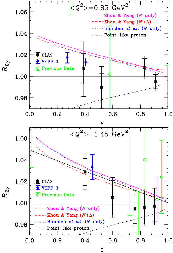
FIG. 20. (Color online) R_{2\gamma} as a function of \epsilon at Q^2 \approx 0.85 \text{GeV}^2 (top) and 1.45 \text{GeV}^2 (bottom) extracted from the measured ratio of e^+p/e^-p cross sections corrected for both \delta_{brem} and \delta_{even} . The filled black squares show the results of this measurement. The inner error bars are the statistical uncertainties and the outer error bars are the statistical, systematic and radiative-correction uncertainties added in quadrature. The line at R_{2\gamma} = 1 is the limit of no TPE. The magenta solid and red dashed curves show the calculation by Zhou and Yang [31] including N only and N + \Delta intermediate states, respectively. The blue dotted curve shows the calculation by Blunden et al. [21]. The black dot-dashed line shows the calculation of TPE effects on a structureless point proton [20]. The open green circles show the previous world data at 0.7 \leq Q^2 \leq 1.0 \text{GeV}^2 and 1.2 \leq Q^2 \leq 1.53 \text{GeV}^2 in the top and bottom plots, respectively [32]. The filled blue diamonds are from VEPP-3 [55] showing the combined statistical and systematic uncertainty. The solid black line in the lower figure is a linear fit to the all of the data shown and was constrained to go to R_{2\gamma} = 1 at \epsilon = 1 .
