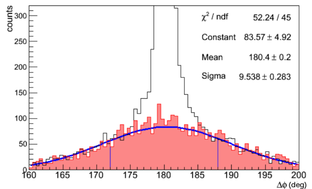
FIG. 17. (Color online) Black histogram is the \Delta\phi distribution for e^-p elastic events at \langle\epsilon\rangle = 0.40 and \langle Q^2\rangle = 1.44 \text{GeV}^2 , the bin with the largest background. The other three kinematic cuts have been applied. Tails of the distribution to the left of 172^\circ and to the right of 188^\circ (shown by vertical lines) were fit with a Gaussian function shown in blue. The filled red histogram is a scaled background sample from Fig. 18.
