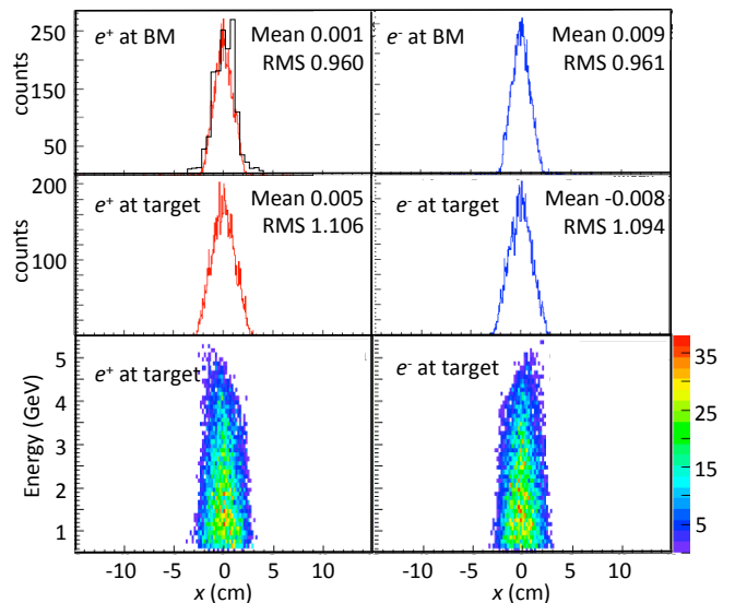
FIG. 9. (Color online) Results of Monte Carlo simulations of the horizontal ( x ) beam distribution at the sparse-fiber beam monitor (top) and the at the upstream face of the target (middle) and the beam-energy versus x distributions at the upstream face of the target for both positrons (left) and electrons (right) for a single chicane polarity. The upper left panel also has a measured spatial distribution for a combined positron/electron beam taken during the run overlaid on the simulation results. The spike in the histogram to the right of the peak is due to improperly gain matched fiber.
