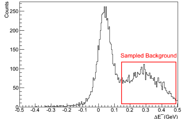
FIG. 18. \Delta E^- distribution for e^-p events at \langle\epsilon\rangle = 0.40 and \langle Q^2\rangle = 1.44 \text{GeV}^2 , the bin with the largest background. The other three kinematic cuts have been applied. The box shows the region of the distribution that was sampled for background.
