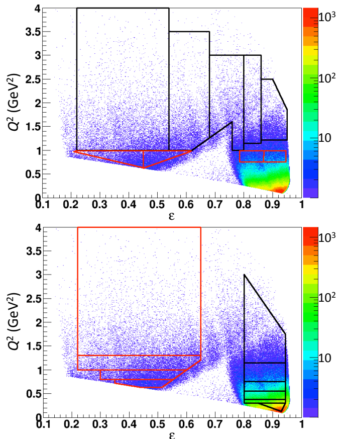
FIG. 15. (Color online) Data binning in Q^2 and \varepsilon overlaid on positive torus e^+p events. The upper plot shows the two sets of bins for the \varepsilon dependence (red and black boxes for \langle Q^2 \rangle = 0.85 and 1.45 \text{GeV}^2 , respectively), while the lower plot shows the two binning choices for the Q^2 dependence (red and black boxes for \langle \varepsilon \rangle = 0.45 and 0.85 , respectively.)
