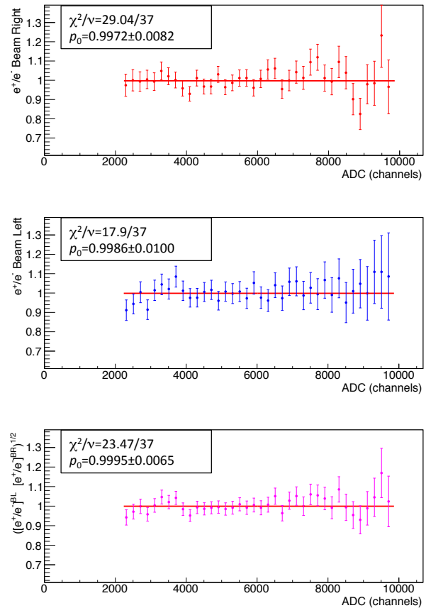
FIG. 8. (Color online) The ratio of the incident positron energy distribution to the incident electron energy distribution versus incident energy (measured in channels where channel 1000 corresponds approximately to 370 MeV) for leptons passing on the right side of the chicane (top panel) and for leptons passing on the left side of the chicane (middle panel), and the square root of the product of the two ratios (bottom panel). The distributions are normalized to unity. The statistics boxes show the results of one-parameter (constant) fits to the ratios.
