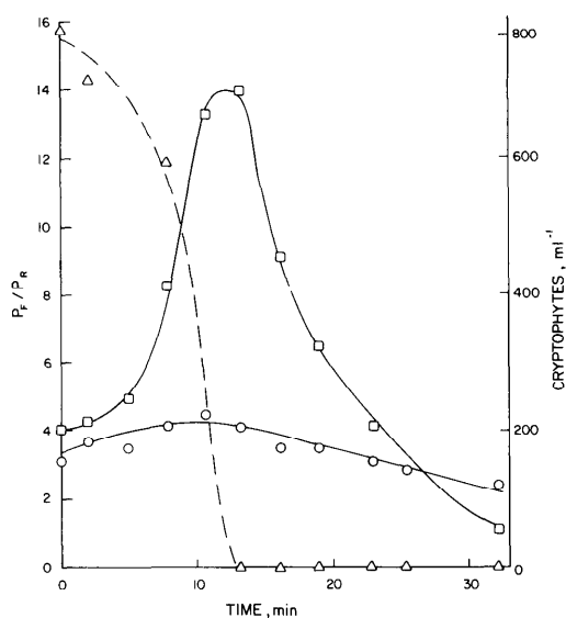
Fig. 3. Time histories of the (normalized) phycoerythrin (□) and Chl a (○) fluorescence intensities for a York River sample. The cell count for cryptophytes (△), obtained using epifluorescence microscopy, is also shown.
