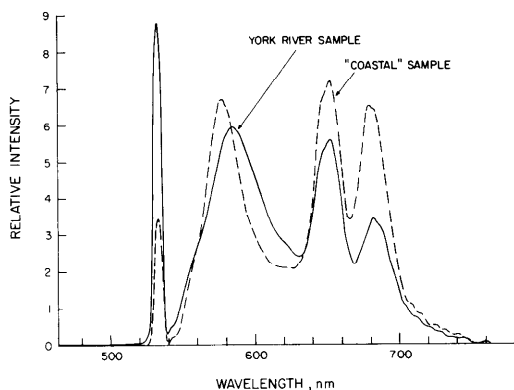
Fig. 1. Spectra obtained from a York River sample and a coastal sample illustrating different spectral characteristics for the phycoerythrin peak.
