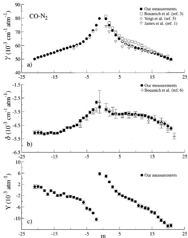
FIG. 3. (a) A comparison of experimental \text{N}_2 -broadening coefficients, \gamma , for the first overtone of CO. (b) A comparison of the \text{N}_2 -shifting coefficients, \delta , of the first overtone spectrum of CO. (c) \text{N}_2 weak mixing coefficients, Y , for the first overtone of CO.
