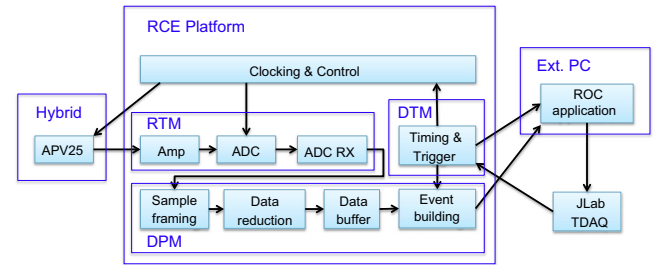
Fig. 10. Block diagram overview of the SVT DAQ.
