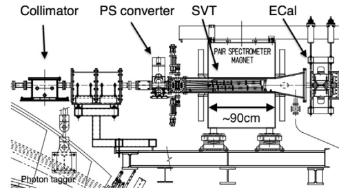
Fig. 2. Layout of the HPS parasitic run.
