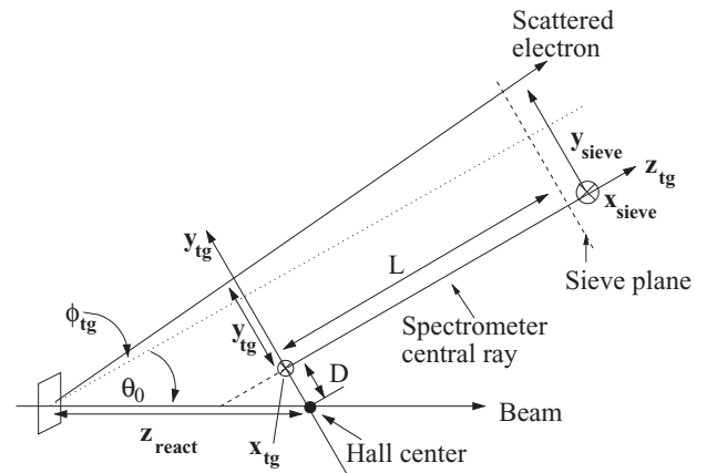
FIG. 12. Top view of the TCS (x_{tg}, y_{tg}, z_{tg}) and the sieve plane coordinate system (x_{sieve}, y_{sieve}) . The z_{tg} axis is along the HRS central ray, the y_{tg} axis is pointing to the left, the x_{tg} axis is pointing vertically down, and the origin of the TCS is the point along the HRS central ray that is the closest to the Hall center. The \phi_{tg} is the tangent of the in-plane angle and \theta_{tg} is the tangent of the out-of-plane angle (not shown) with respect to the spectrometer central ray. The sieve plane is located at a drift distance L = 1.12 m from the TCS origin, with the y_{sieve} axis pointing to the left of the spectrometer entrance and the x_{sieve} axis pointing vertically down. The pointing of the spectrometer, D , describes how much the HRS central ray misses the Hall center, and \theta_0 is the angle of the HRS central ray with respect to the beamline. Figure reproduced from Refs. [54,70].
