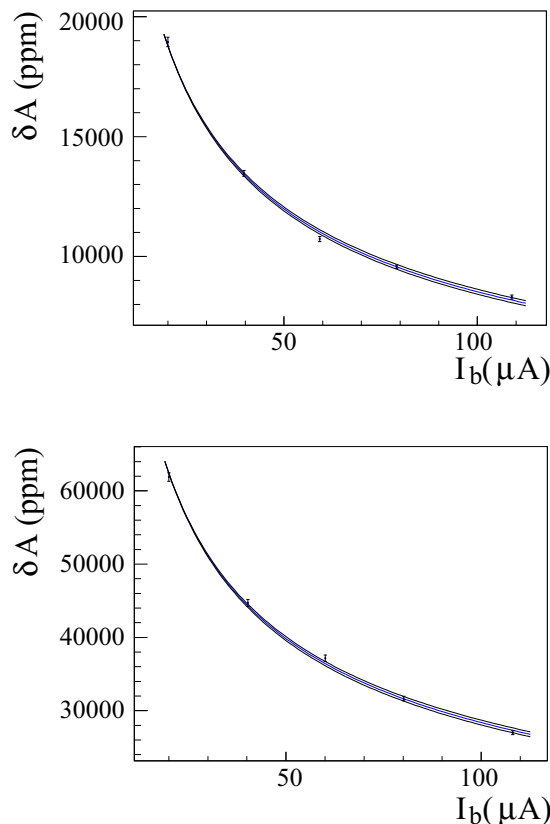
FIG. 8. (Color online) Measured standard deviation of the pairwise asymmetries at various beam currents for DIS#1 (top) and DIS#2 (bottom), with a 4 \times 4 \text{ mm}^2 square raster. The curves show the results of the fit \delta A \propto I^{p_3} and its error band. The fit results are p_3 = 0.4900 \pm 0.0076 and p_3 = 0.4897 \pm 0.0072 for DIS#1 and DIS#2, respectively. These results are in good agreement with pure counting statistics ( \delta A \propto \sqrt{I} ).
