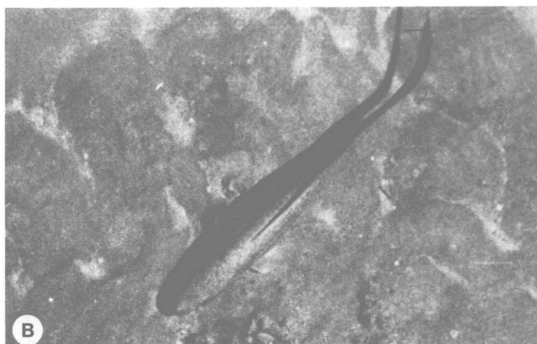
Figure 1. A, Monomitopus magnus with a small rattail in close attendance. Blake Plateau, 30°51'N, 78°8'W–30°50'N, 78°3'W, 920–970 m; B, dorsal view of M. magnus swimming over bottom in region of Blake Plateau. A from Hersey (1967).
