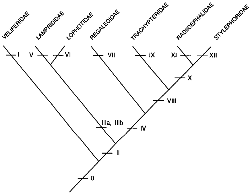
Figure 3. Hypothesis of relationships of lampridiform families proposed by Oelschläger, 1983 and redrawn from his fig. 109. Numbers refer to the following synapomorphies: (0) strongly protractile jaw apparatus for small animal feeding; (I) scaly sheath on dorsal- and anal-fin bases; (II) horizontal pectoral fins; (IIIa) strong separation of coracoid and distal cleithrum; (IIIb) pectoral-fin radials with clearly marked ovoid condyles; (IV) friction reducing skin; (V) shoulder girdle as a secondary swimming apparatus; (VI) frontal-occipital crest with a rostral horn; (VII) pelvic fins with chemical receptive organs; (VIII) symmetric insertion of pectoral erector muscle; (IX) dorsal lobe of caudal fin bears lateral line; (X) ventral lobe of caudal fin bears lateral line; (XI) pelvic fins abdominal; (XII) protractile jaw like a pipette.
