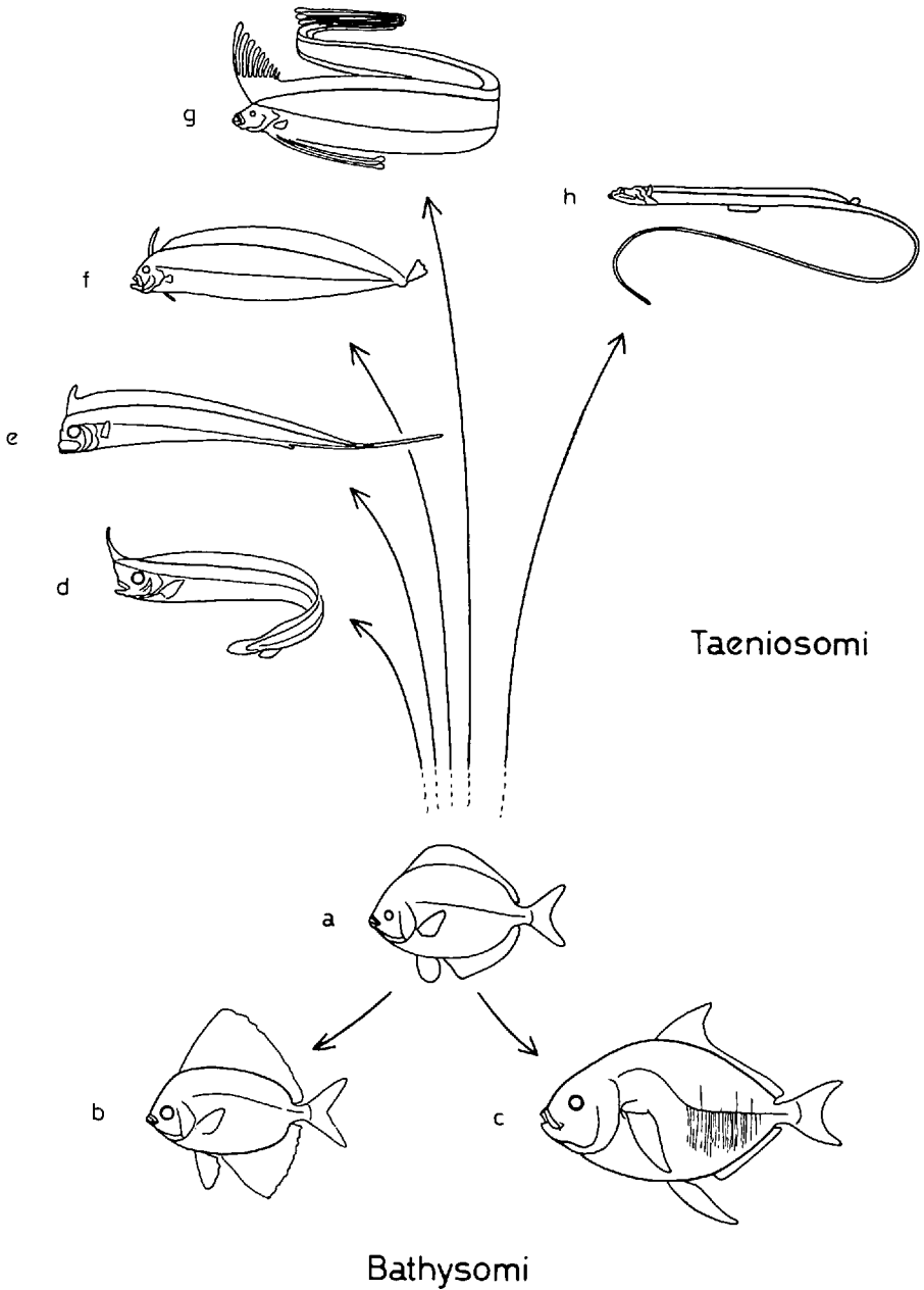
Figure 2. Morphological radiation of Lampridiform (=Allotriognath) families (from Oelschläger, 1976): a) an hypothesized ancestral lampridiform; b) Veliferidae; c) Lamprididae; d) Lophotidae; e) Radiicephalidae; f) Trachipteridae; g) Regalecidae; h) Stylephoridae.
