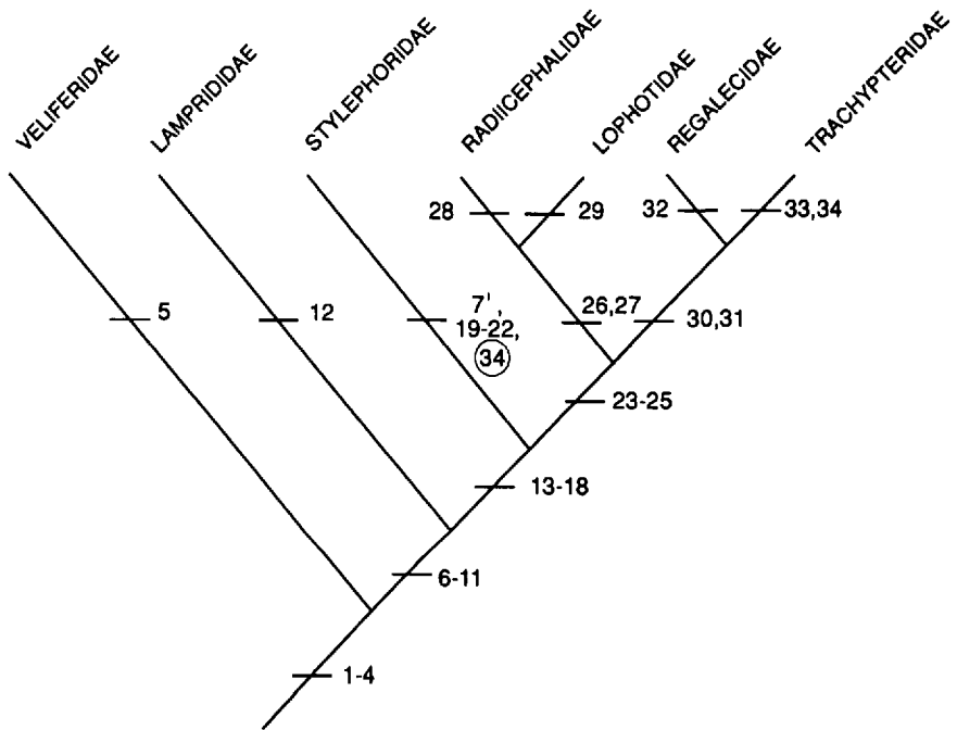
Figure 12. Cladogram depicting hypothesized relationships of lampridiform families. Numbers refer to the following synapomorphies: (1) absence of the anterior palatine process and the anterior palatomaxillary ligament; (2) mesethmoid posterior to lateral ethmoids; (3) elongate ascending processes of premaxillae and large rostral cartilage insert into frontal vault or cradle; (4) first dorsal-fin pterygiophore inserts anterior to first neural spine; (5) dorsal- and anal-fin bases with scaly sheaths; (6) large, pelagic eggs with red-brown chorion; (7) first pectoral-fin radial fused to the scapula, remaining three radials autogenous; (8) absence of uncinat process on first epibranchial; (9) absence of autogenous pelvic-fin radials; (10) more than 40 total vertebrae; (11) second, third and fourth pharyngobranchials columnar, obliquely oriented and with small, posteroventral toothplates; (12) foramen magnum enclosed in cranial condyle; (13) absence of supraneurals; (14) absence of supraoccipital crest; (15) first two dorsal-fin pterygiophores greatly enlarged and inclined sharply forward over the cranium; (16) first neural spine directed anteriorly, usually curving over posterior surface of the cranium; (17) fewer than 20 total caudal-fin rays, some of which are enlarged; (18) first vertebral centrum reduced in length; (19) second neural spine absent, neural arch m-shaped; (20) loss of rostral cartilage; (21) palatine reduced to small, straight rod; (22) posterior shift in first dorsal-fin pterygiophore position; (23) dorsal-fin rays bear lateral spinules; (24) one or two fang-like teeth on the vomer; (25) more than 60 total vertebrae; (26) anteriorly projecting supraoccipital process; (27) ink gland present; (28) elongate haemal spines on PU4–PU6; (29) supraoccipital spine enlarged and supporting first dorsal-fin pterygiophore; (30) absence of anal fin; (31) caudal- and pelvic-fin rays bear lateral spinules; (32) pelvic-fin rays reduced in number to one stout, elongate ray and one small splint-like element; (33) lateral line scales bear spines; (34) absence of pleural ribs. Character 7' is a reversal, and the circled number indicates independent origin.
