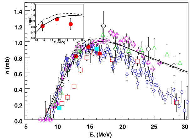
Fig. 3. (Color online.) All currently available total cross section data for the {}^3\text{He}(\gamma, n)pp reaction up to 30 MeV: Ref. [7] and datum at 16.5 MeV presented for first time in this letter (filled circles), Ref. [39] (open circles), Ref. [40] (open squares), Ref. [41] (diamonds), Ref. [42] (open upward triangles), Ref. [43] (open crosses), Ref. [44] (filled squares), Ref. [33] (filled upward triangles), Ref. [45] (filled downward triangle) in comparison to the calculations from Ref. [19] (solid curve) and Ref. [20] (dashed curve). In the insert, the data by our collaboration are shown and compared with the theories. The older measurements [39–41,43] are presented with the statistical uncertainties while the newer data points [7,44,33,45] include both the statistical and systematic errors added in quadrature.
