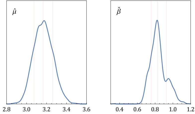
FIG. 12: Results for the energy shifts of a spin-up (lower points) and a spin-down (upper points) proton in a uniform background magnetic field. The details of the figure are as in Fig. 9. The lower panel shows the PDFs for the fit parameters \hat{\mu} and \hat{\beta} .
