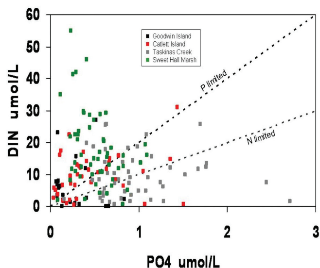
Figure 15. Water column DIN:PO 4 ratios for Reserve components. Dashed lines depict ratios of 10 and 20; ratios <10 indicate N limitation and >20 indicates P limitation (BOYNTON et al. , 1982). Data source: NOAA/NERRS SWMP monthly sampling program for the period 2002-2006; samples below detection limits were not included in analysis.
