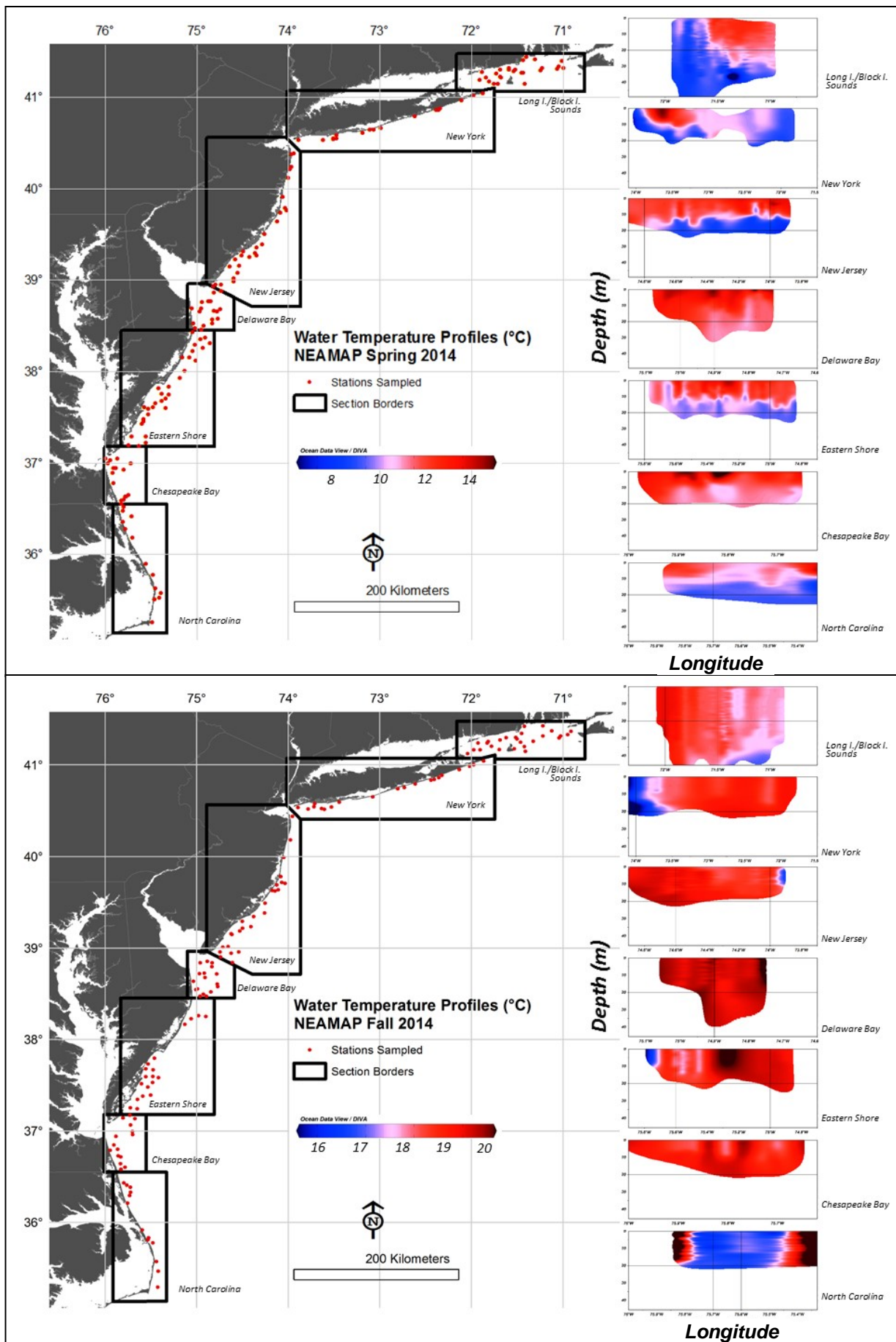
Figure 4. Water column temperature profiles integrated within defined 'section' boundaries for spring (A) and fall (B) 2014.
