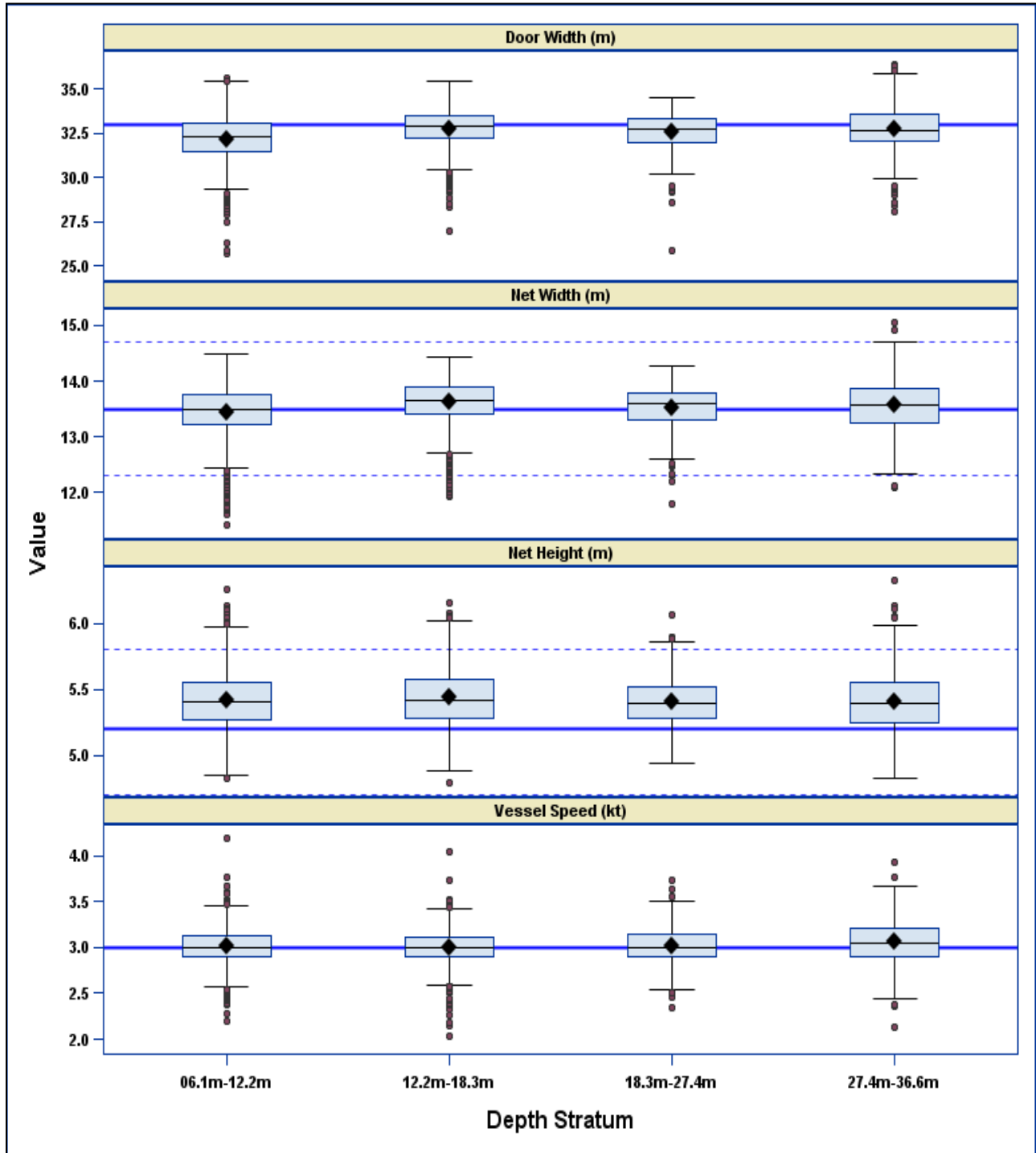
Figure 5B. Performance of the NEAMAP sampling gear for all tows during each research cruise, by depth stratum*.
