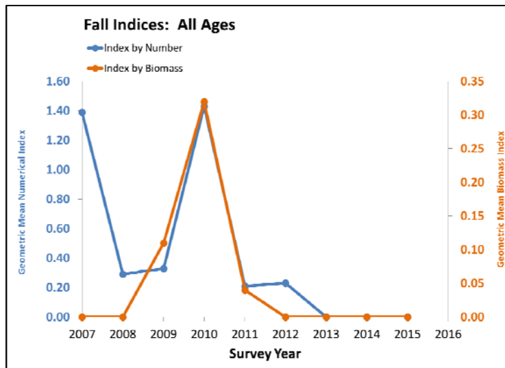
Figure 159. Spanish Mackerel geometric mean indices of abundance, by number and biomass, for fall NEAMAP surveys, for all specimens captured.
