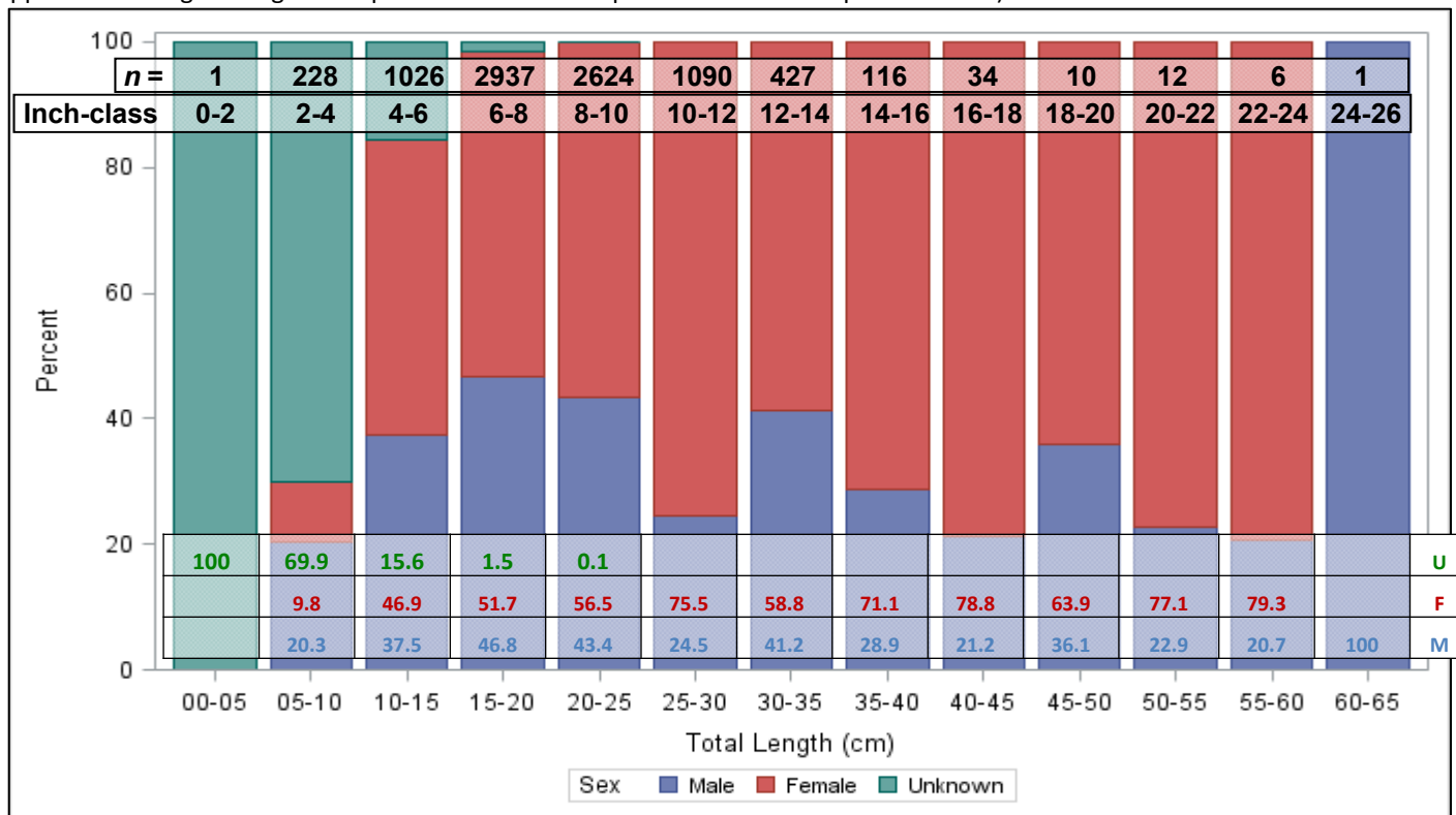
Figure 212. Weakfish maturity at length, by sex for all cruises pooled, 2007-2015.
