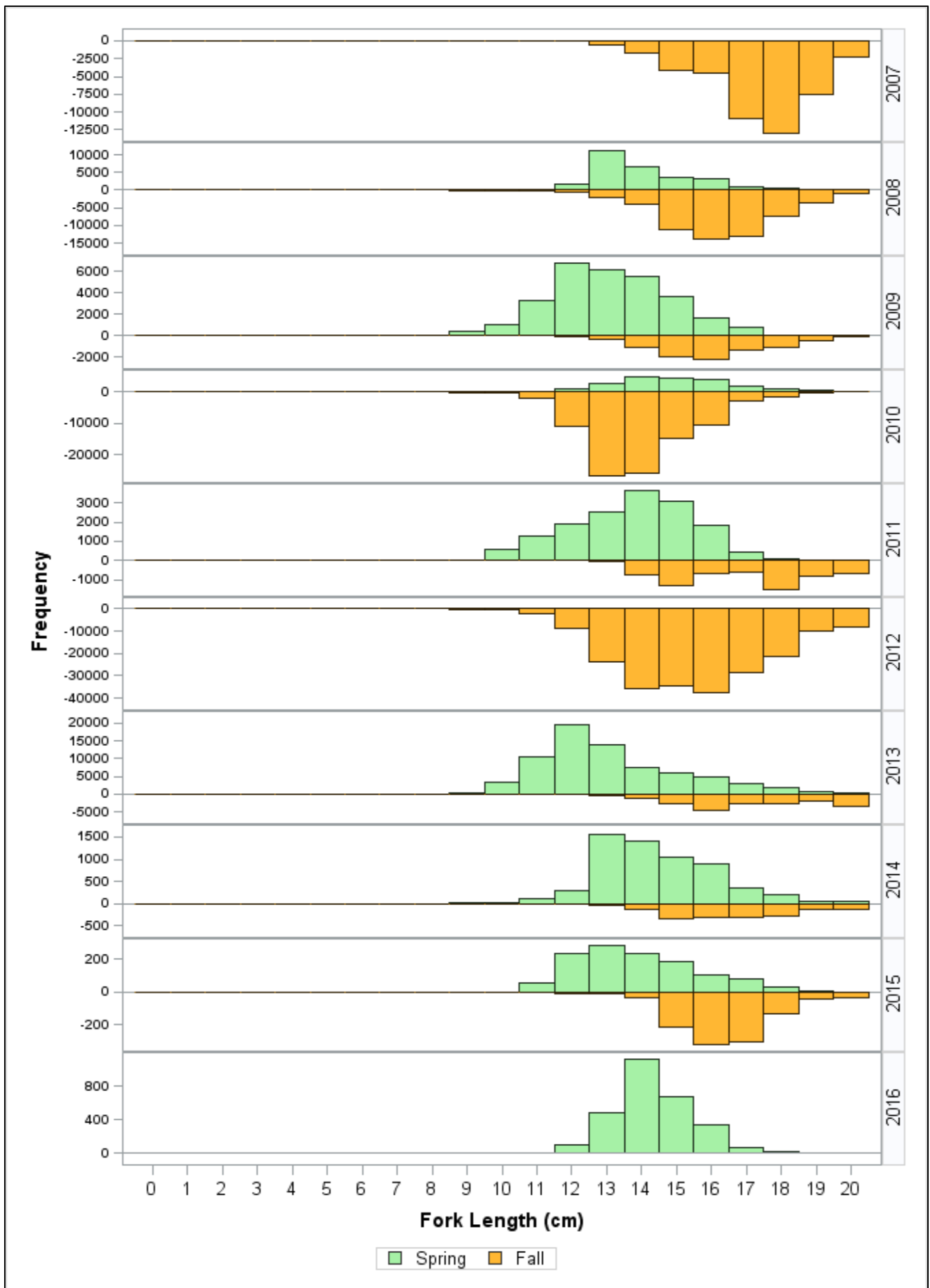
Figure 176. Spot length-frequency distributions, by cruise.
