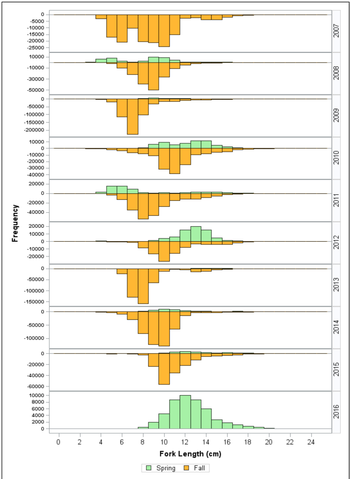
Figure 88. Butterfish length-frequency distributions, by cruise.
