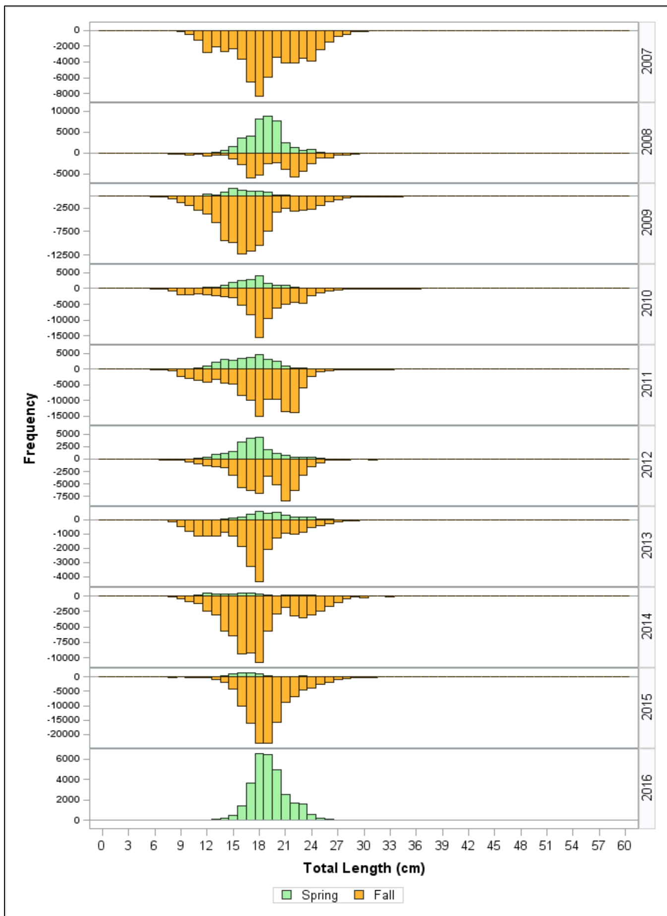
Figure 207. Weakfish length-frequency distributions, by cruise.
