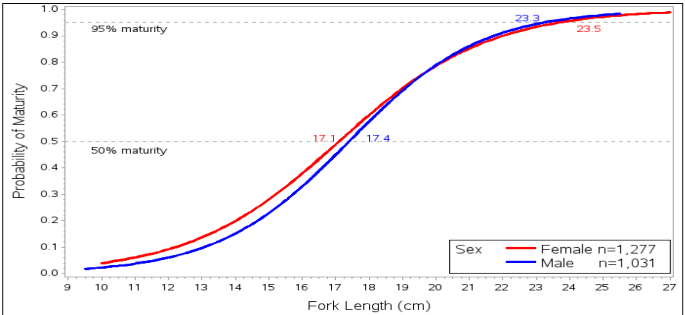
Figure 178. Spot maturity at length, by sex for all cruises pooled, 2007-2015.
