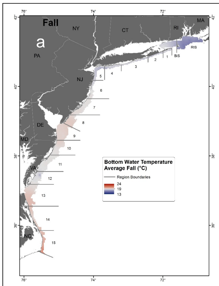
Figure 3P. Bottom temperatures as measured by NEAMAP for fall 2014. (Map 'a' represents measured values averaged over all fall cruises between 2007 and 2014, 'b' gives actual values for fall 2014, and 'c' represents the difference.)
