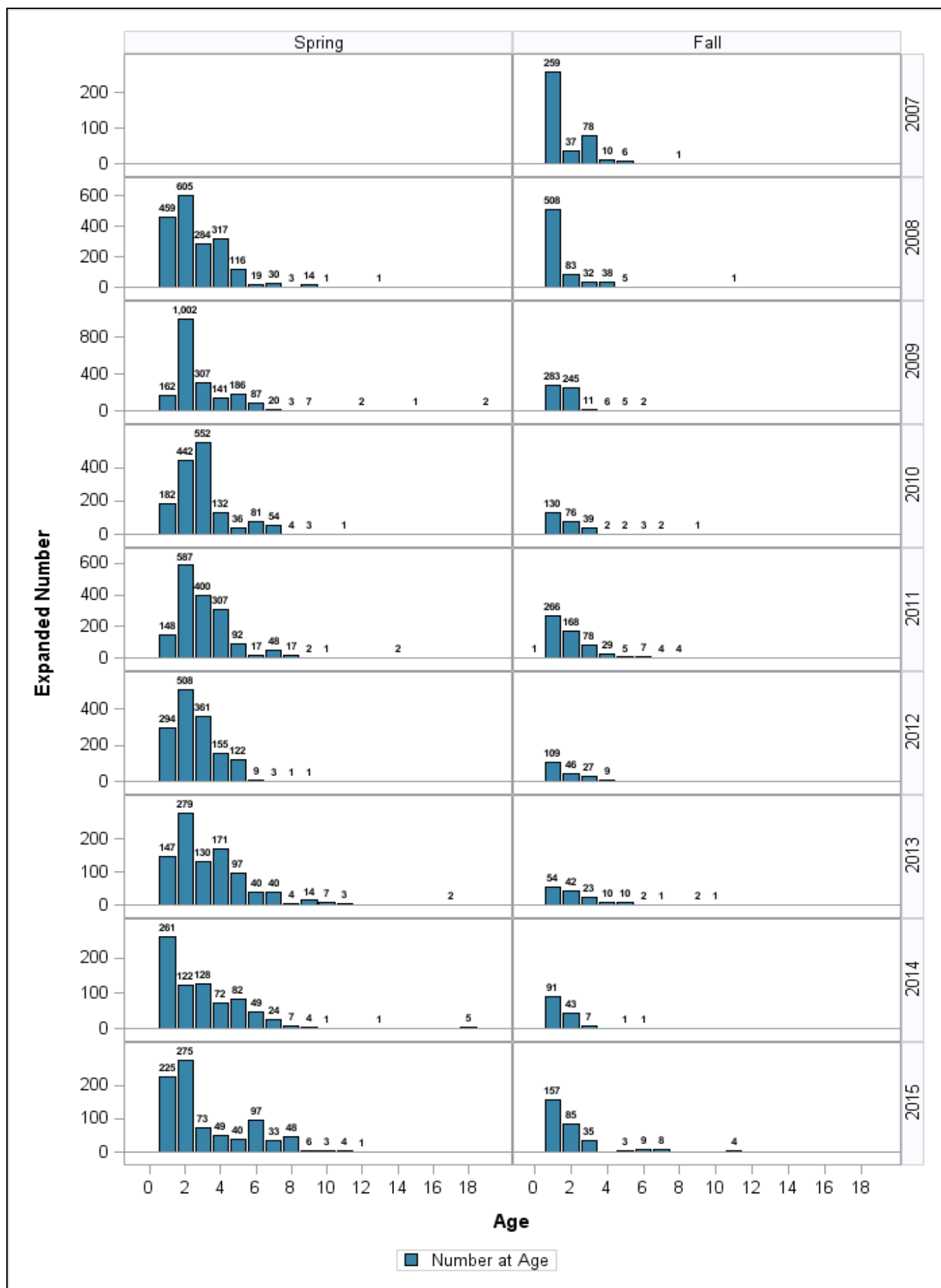
Figure 229. Winter Flounder age-frequency distribution, by cruise. The estimated total number collected at a given age is provided above each corresponding bar. (Values in red were generated by application of age-length keys.)
