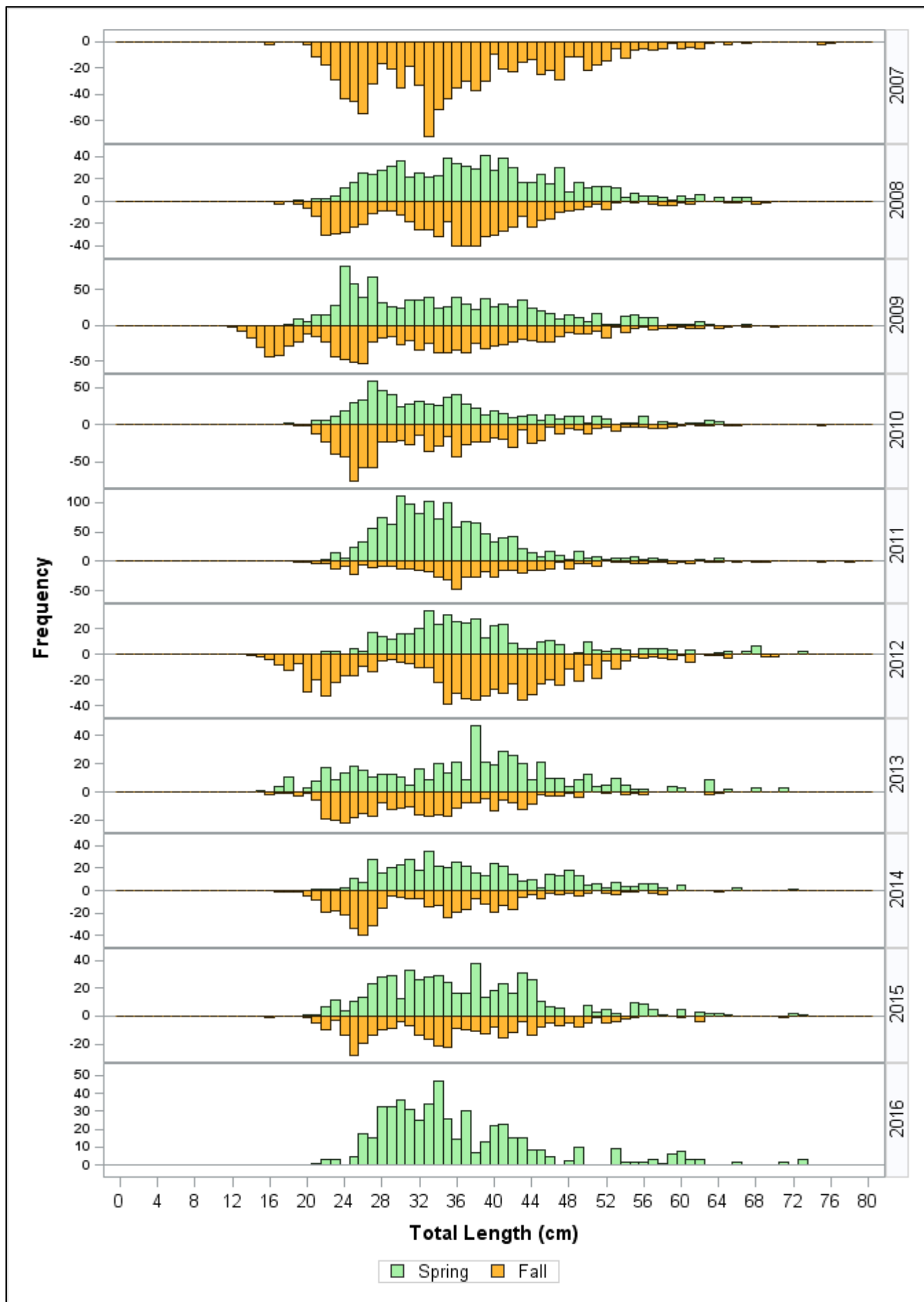
Figure 192. Summer Flounder length-frequency distributions, by cruise.
