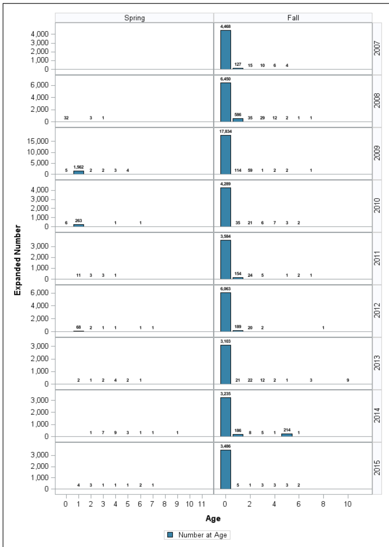
Figure 77. Bluefish age-frequency distribution, by cruise. The estimated total number collected at a given age is provided above each corresponding bar.
