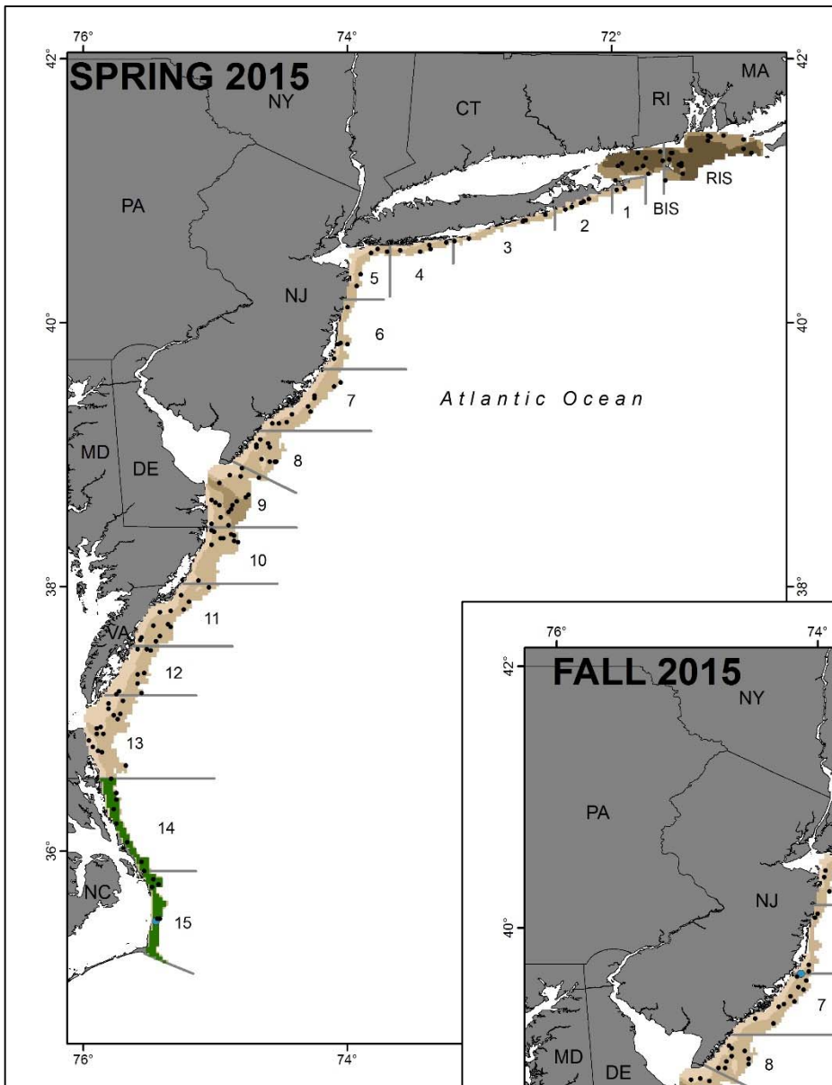
Figure 215. White Shrimp biomass (kg) at each sampling site for 2015 NEAMAP cruises and strata used for calculation of abundance indices.
