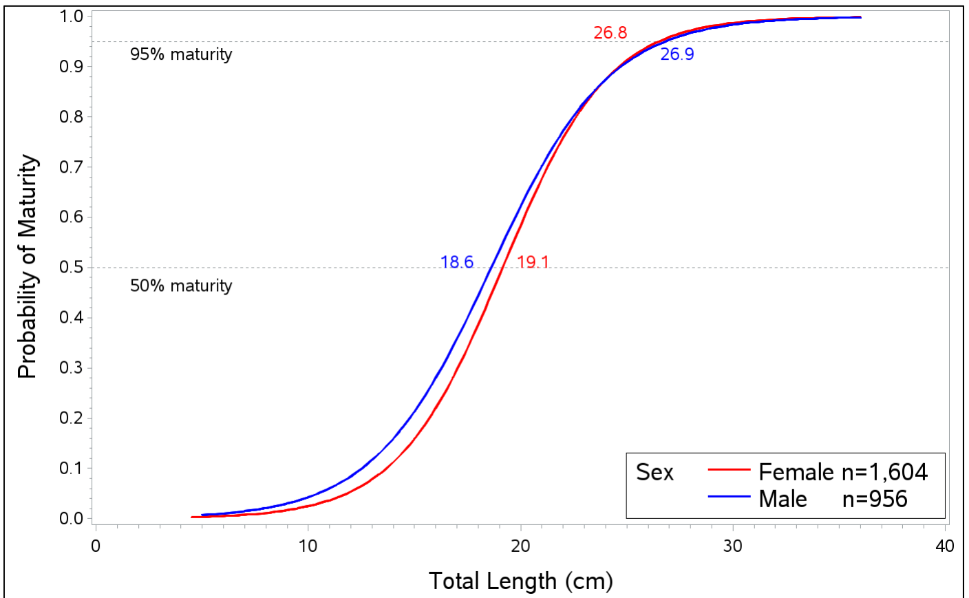
Figure 223. Windowpane Flounder maturity at length, by sex for all cruises pooled, 2012-2015.
