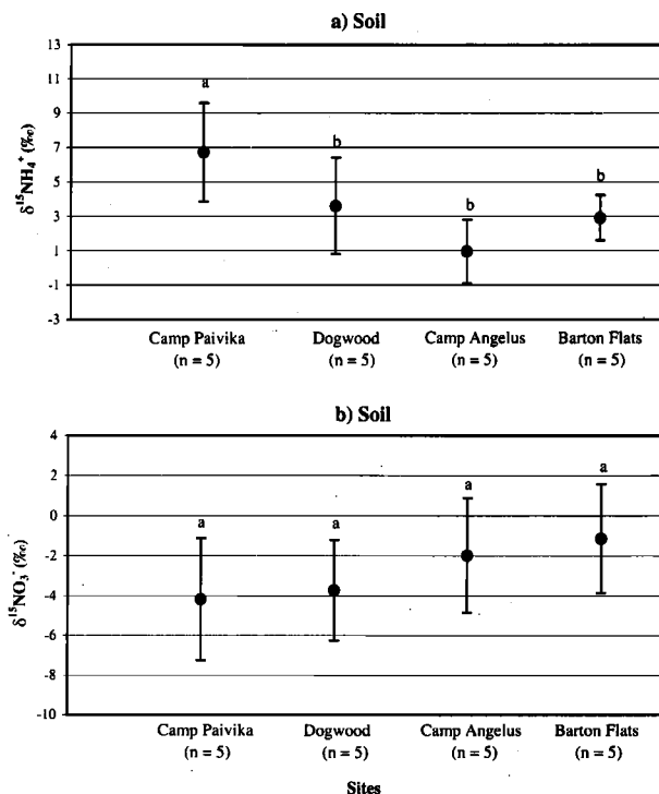
Figure 5. Soil \delta^{15}\text{NH}_4^+ and \delta^{15}\text{NO}_3^- values across the west to east air pollution gradient. Means followed by the same letter are not statistically different (mean \pm \sigma ).
