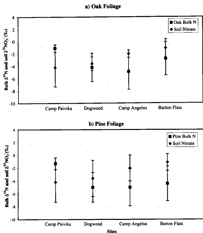
Figure 6. Vegetation bulk \delta^{15}\text{N} and soil \delta^{15}\text{NO}_3^- .
