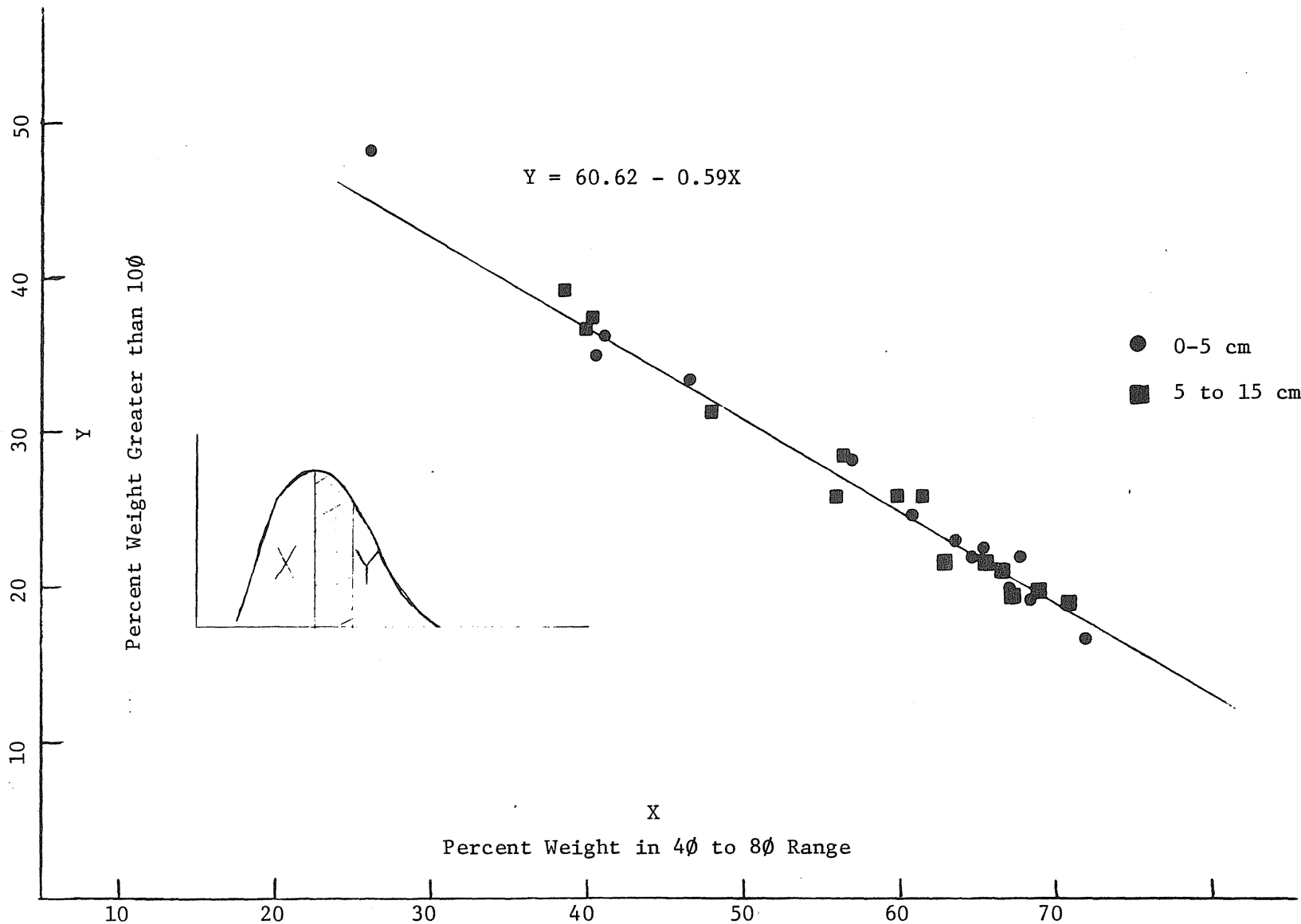
Figure III-5. Regression of percent weight in 4φ to 8φ size range versus percent weight finer than 10φ.
