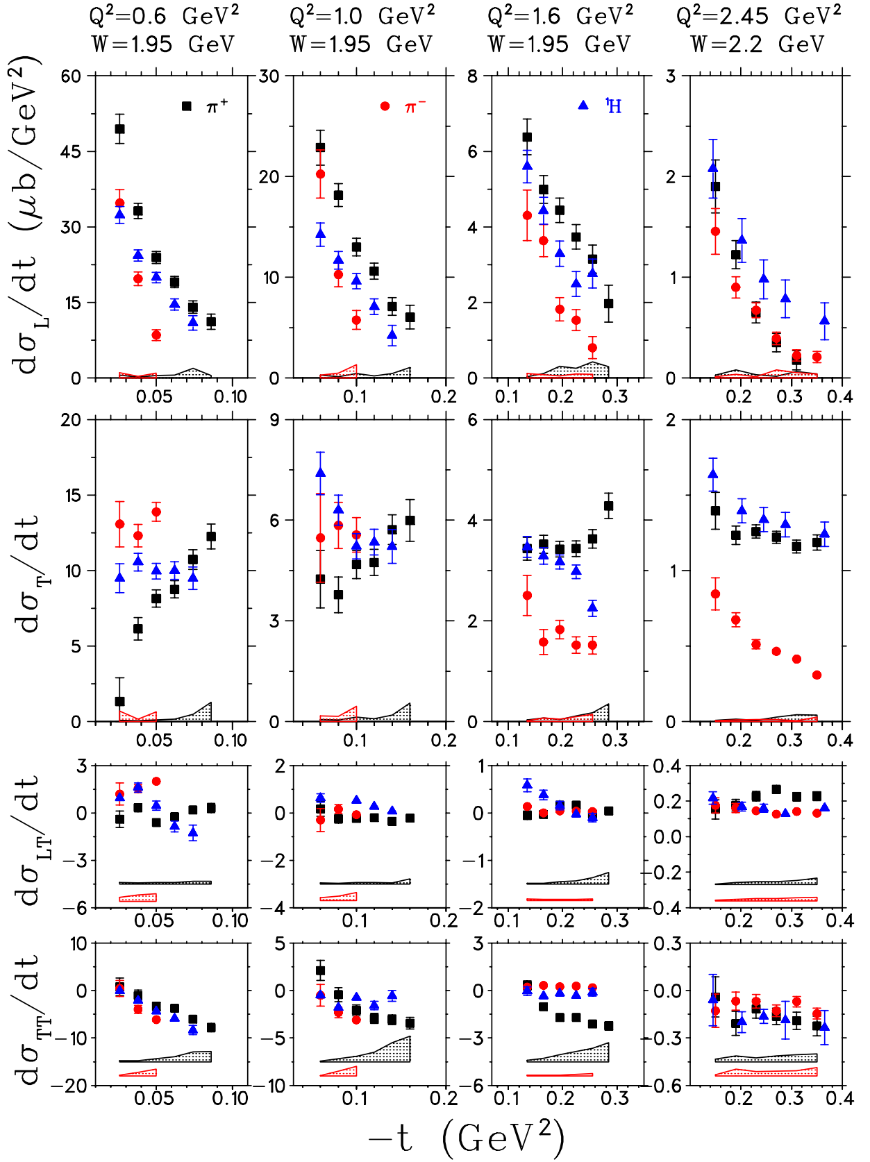
FIG. 10. (Color online) Separated cross sections as a function of -t . \pi^- from {}^2\text{H} : [red circles], \pi^+ from {}^2\text{H} : [black squares], \pi^+ from {}^1\text{H} : [blue triangles]. The error bars include both statistical and uncorrelated systematic uncertainties. The “model-dependences” of the L , T , LT , TT cross sections are indicated by the shaded bands, by which all data points move collectively. The {}^1\text{H} data have not been scaled to the mean Q^2 , \bar{W} values for each -t bin of {}^2\text{H} data. In addition, please keep in mind the issues relating to {}^2\text{H} off-shell effects before directly comparing the {}^1\text{H} and {}^2\text{H} data.
