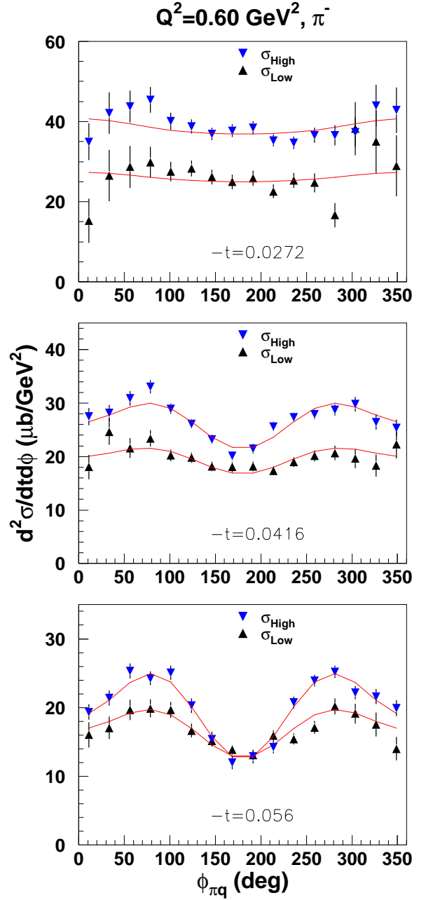
FIG. 9. (Color online) Unseparated experimental \pi^- cross sections as a function of azimuthal angle \phi at Q^2=0.60 \text{ GeV}^2 , low \epsilon (black triangles) and high \epsilon (blue inverted triangles). The curves shown represent the fit of the measured values of the cross section to Eqn. 6. In this fit, all four parameters \sigma_{L,T,LT,TT} are extracted simultaneously, separate for each -t bin.
