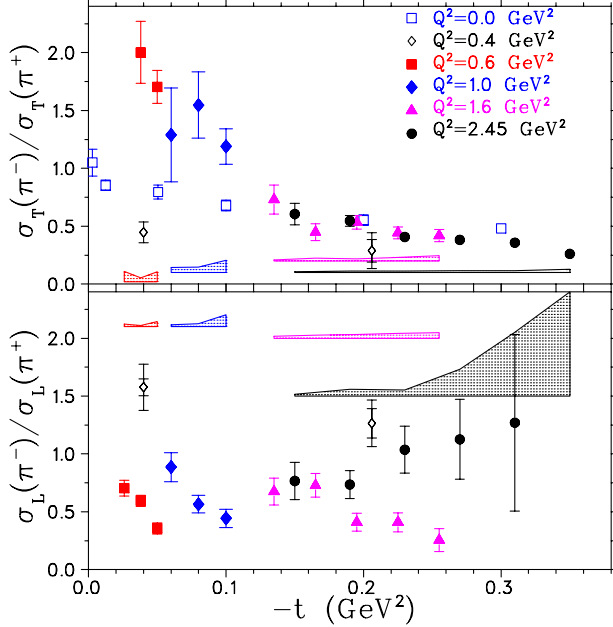
FIG. 12. (Color online) The ratios R_L and R_T versus -t for four Q^2 settings from this work. The model-dependences of the ratios are indicated by the shaded bands, and the error bars include statistical and uncorrelated systematic uncertainties. Also shown are the ratios at Q^2=0.4 GeV ^2 in the resonance region from Refs. [24, 30], and R_T from the E_\gamma=3.4 GeV photoproduction data of Ref. [31].
