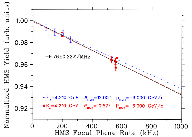
FIG. 2. (Color online) Normalized yields (no PID cut) from the carbon target versus HMS singles rate. As the tracking efficiency calculation uses a data sample where multiple track events are rejected, the HMS tracking efficiencies are overestimated at high rates, leading to an effective drop in normalized yield versus rate. The HMS tracking efficiencies for both of the F _{\pi-1} and F _{\pi-2} data sets are corrected with the linear rate dependent function shown here, leading to a normalized yield that is independent of rate.
