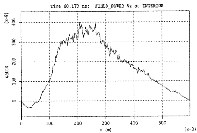
Figure 5.12: The energy flux distribution in the bulb
