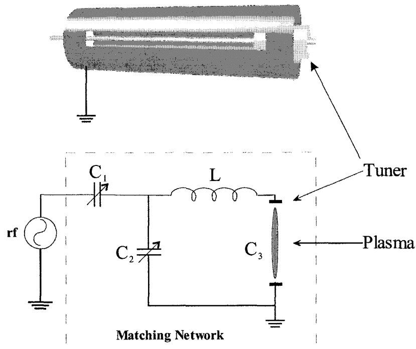
Figure 3.2: Matching network
