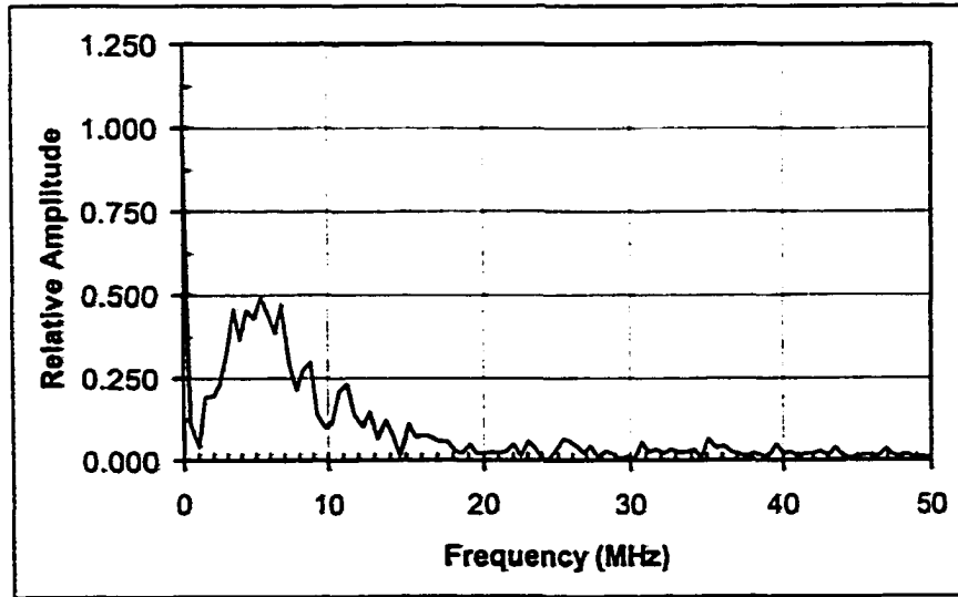
Figure 5.39: Epicentral displacement in woven GR/Epoxy generated by the EO Q-switched Nd:YAG (1.064 \mu\text{m} ).
