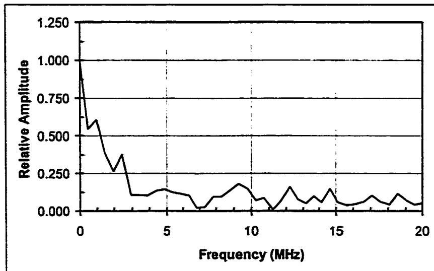
Figure 5.55: Epical displacement in epoxy generated by the AO Q-switched Nd:YAG (1.064 \mu\text{m} ) laser.
