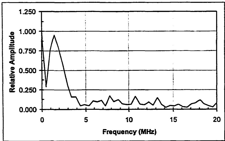
Figure 5.67: Epicentral displacement in stitched woven GR/Epoxy generated by the AO Q-switched Alexandrite laser.
