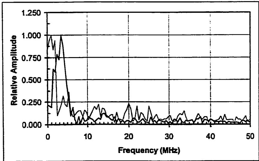
Figure 5.29: Epicentral displacement in aluminum generated by the RM Q-switched CTH:YAG ( 2.10 \mu\text{m} ) laser with a constraining layer of vacuum grease.
