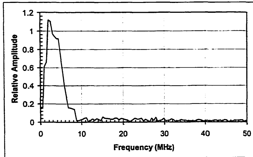
Figure 5.63: 10 MHz transducer response and frequency spectrum of the first wave arrival in the stitched woven GR/Epoxy sample.
