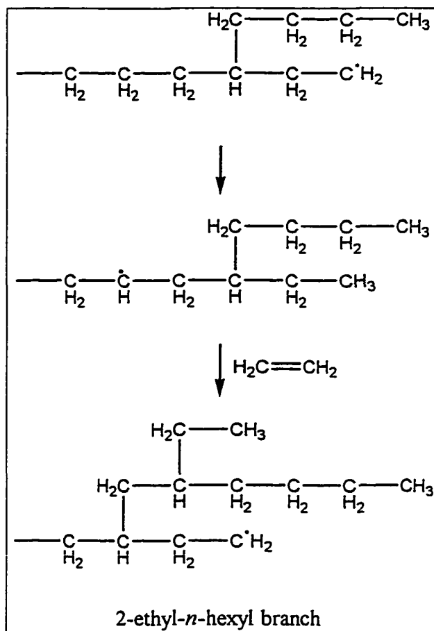
Scheme 2.21: Formation of 2-ethyl- n -hexyl branch caused by double backbiting mechanism
