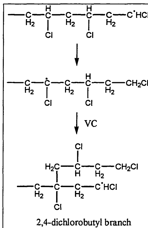
Scheme 2.19: Formation of 2,4-dichlorobutyl branch caused by backbiting mechanism
