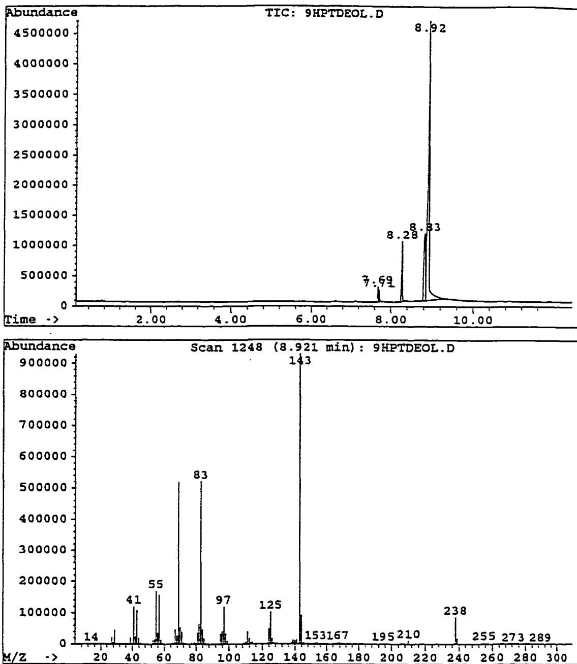
Fig. 3.24: Mass spectrum and gas chromatogram of 9-heptadecanol
