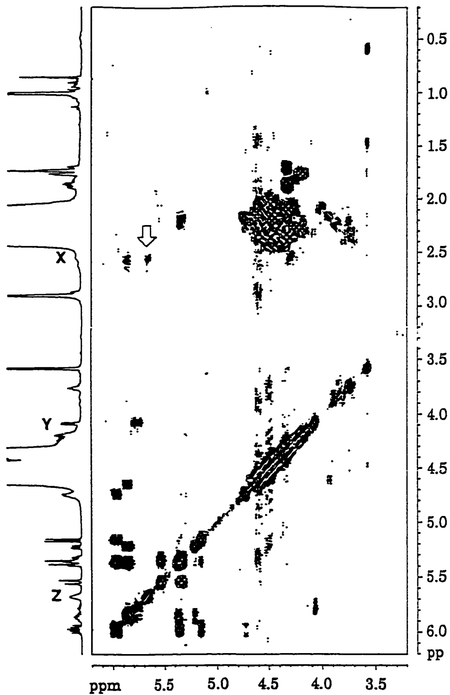
Fig. 4.2: Phase-sensitive DQF-COSY 2D ^1\text{H} NMR partial spectrum (500.14 MHz, \text{THF-}d_8 , 23 ^\circ\text{C} ) of (t\text{-Bu})_2\text{Mg} -initiated PVC
