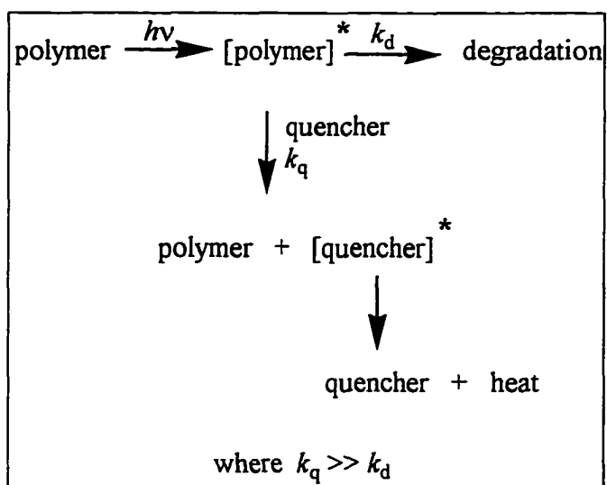
Scheme 2.13: Photostabilization of PVC by excited-state quenchers
