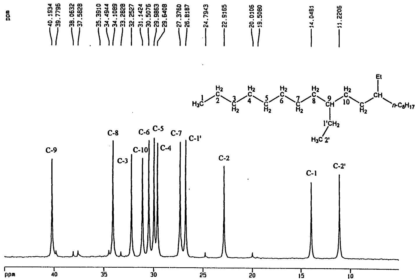
Fig. 3.40: 13 C NMR spectrum (125.77 MHz) of 9,12-diethyleicosane prepared by homocoupling
