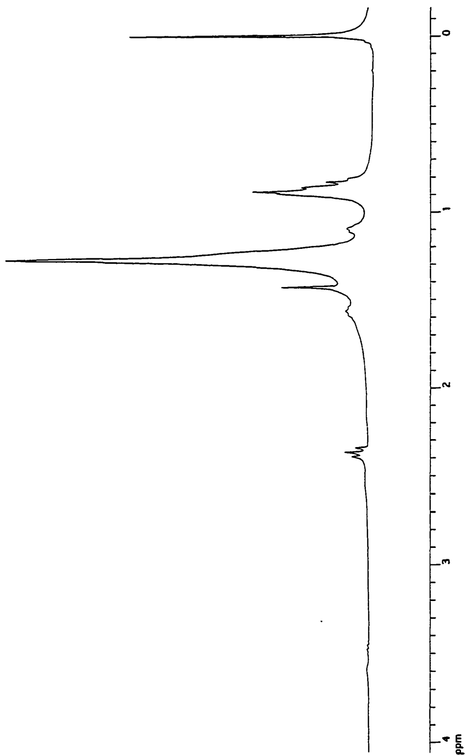
Fig. 3.21: ^1\text{H} NMR spectrum (300.592 MHz) of 9-(2-ethyl-1-hexyl)heptadecane
