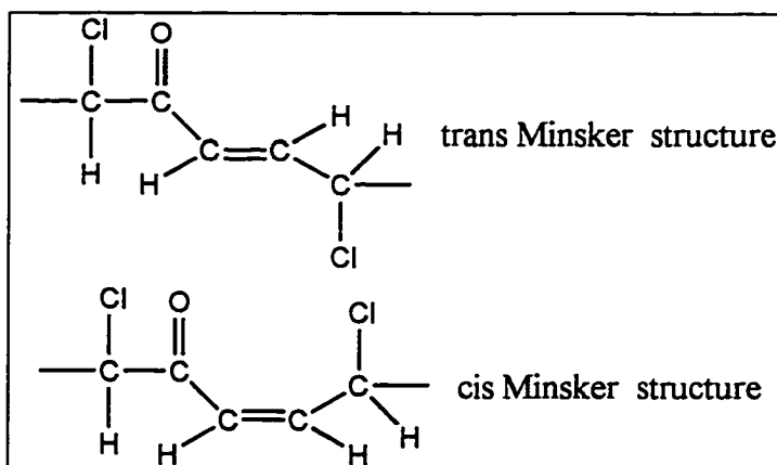
Scheme 2.18: Minsker structures
