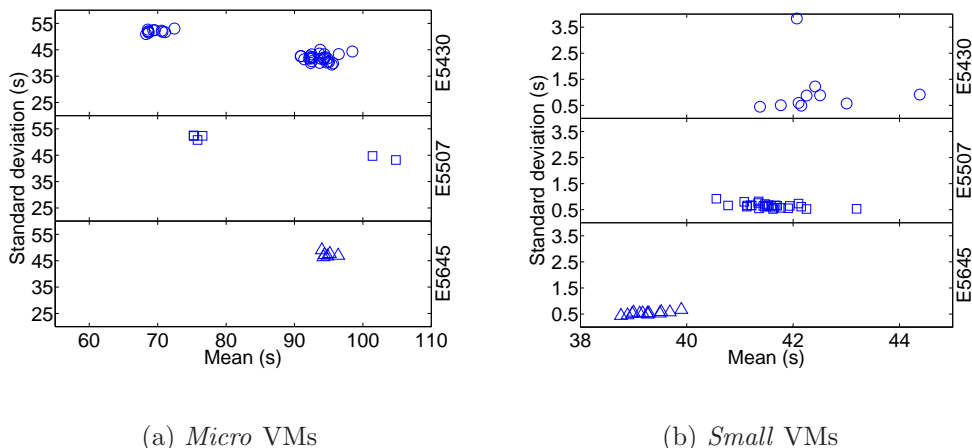
Figure 4.1: Performance results of 50 spot instances avrora on different hardware.
