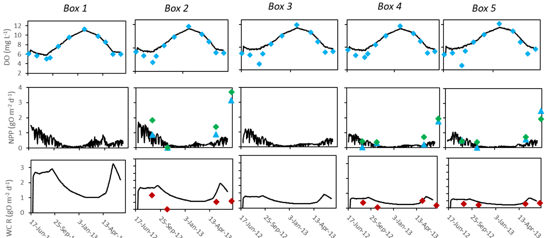
Figure 10: Measured (diamonds) and modeled (black lines) Dissolved Oxygen concentration, Water Column NPP rates, and Water column R rates. Data for calibration of water column NPP are water column GPP (diamonds) along with water column NCP (triangles)
