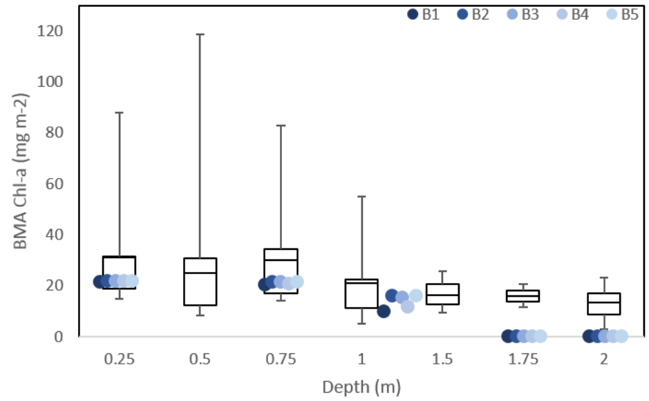
Figure 13: Benthic Microalgae Chlorophyll- a concentrations in the top 3 mm from the May 9, 2014 system survey (box and whiskers) and the model simulation (points) averaged for May 2013. (Points between 1 and 1.5m represent modeled values at 1.25m.)
