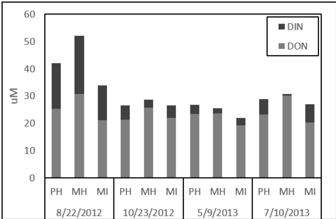
Figure 17: Water Column TDN (DIN and DON) concentrations from seasonal sampling dates at sites PH, MH, and MI.
