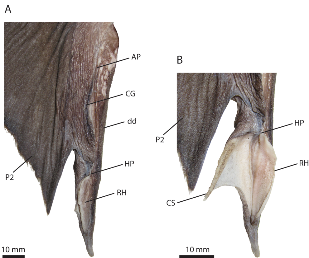
FIGURE 9. Clasper (left) of Centrophorus granulosus (CSIRO H 5343–07, adult male 1176 mm TL). A, Glans not dilated; B, Glans spread. Abbreviations: AP, apophyle; CG, clasper groove; CS, clasper spine; dd, dermal denticles; HP, hypophyle; P2, pelvic fin; RH, rhipidion.
