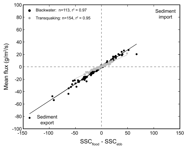
Figure 3. Mean sediment flux per unit channel area from Ganju et al. [2013] versus flood-ebb SSC differential. Fluxes and SSC from sites BWR and FB1 were averaged over 12 h windows; SSC measurements were time weighted to account for any differences in flood/ebb duration.
