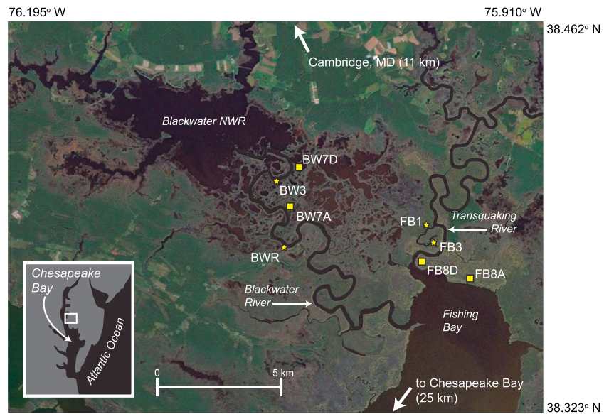
Figure 1. Study area, on the eastern side of Chesapeake Bay, USA. Sites with boxes are accretion measurement locations, sites with stars are SSC measurement locations.
