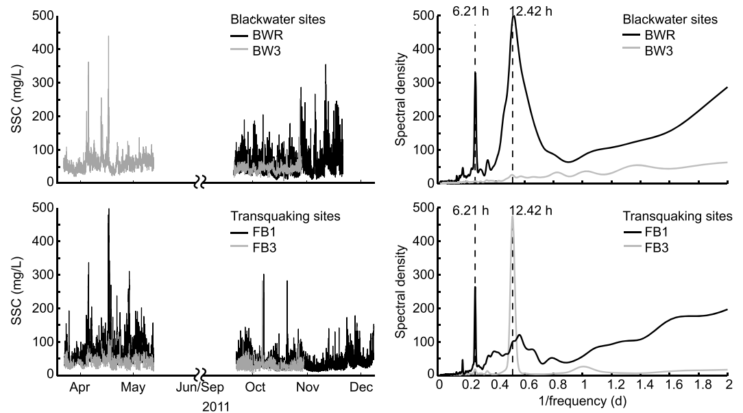
Figure 2. (left column) SSC time series and (right column) spectral density from (top row) Blackwater River sites and (bottom row) Transquaking River sites. Coherence at 6.21 h corresponds to flood and ebb tidal advection, coherence at 12.42 h indicates correspondence with either flood or ebb tidal advection. In this case, the large 12.42 h peak at BWR corresponds with ebb tide advection, while the large 12.42 h peak at FB3 corresponds to flood tide advection.
