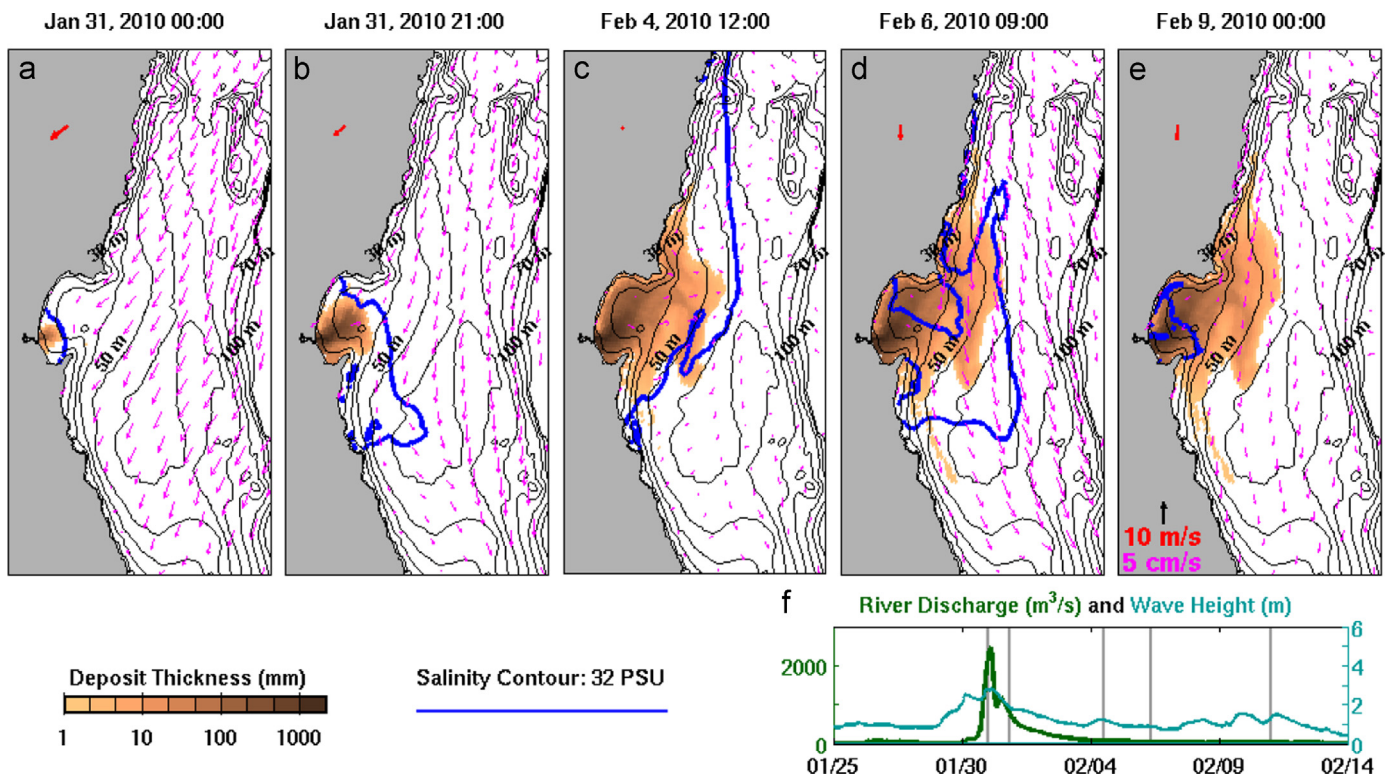
Fig. 4. January, 2010 flood ‘snapshots’ showing salinity contour (32 PSU) for surface waters (blue contours on maps), depth averaged currents (pink arrows), spatially-averaged wind (red arrow), and deposit thickness (brown shading on maps). Panels represent (a) early flood, (b) mid flood, during a time of onshore winds, (c) flood plume during a period of weak winds, (d) flood plume during a period of variable winds, and (e) post-flood. The gray lines on the time series of river discharge (dark blue) and wave height (turquoise) in panel (f) indicate the timing of the snapshots in (a)–(e) (For interpretation of the references to color in this figure legend, the reader is referred to the web version of this article).
