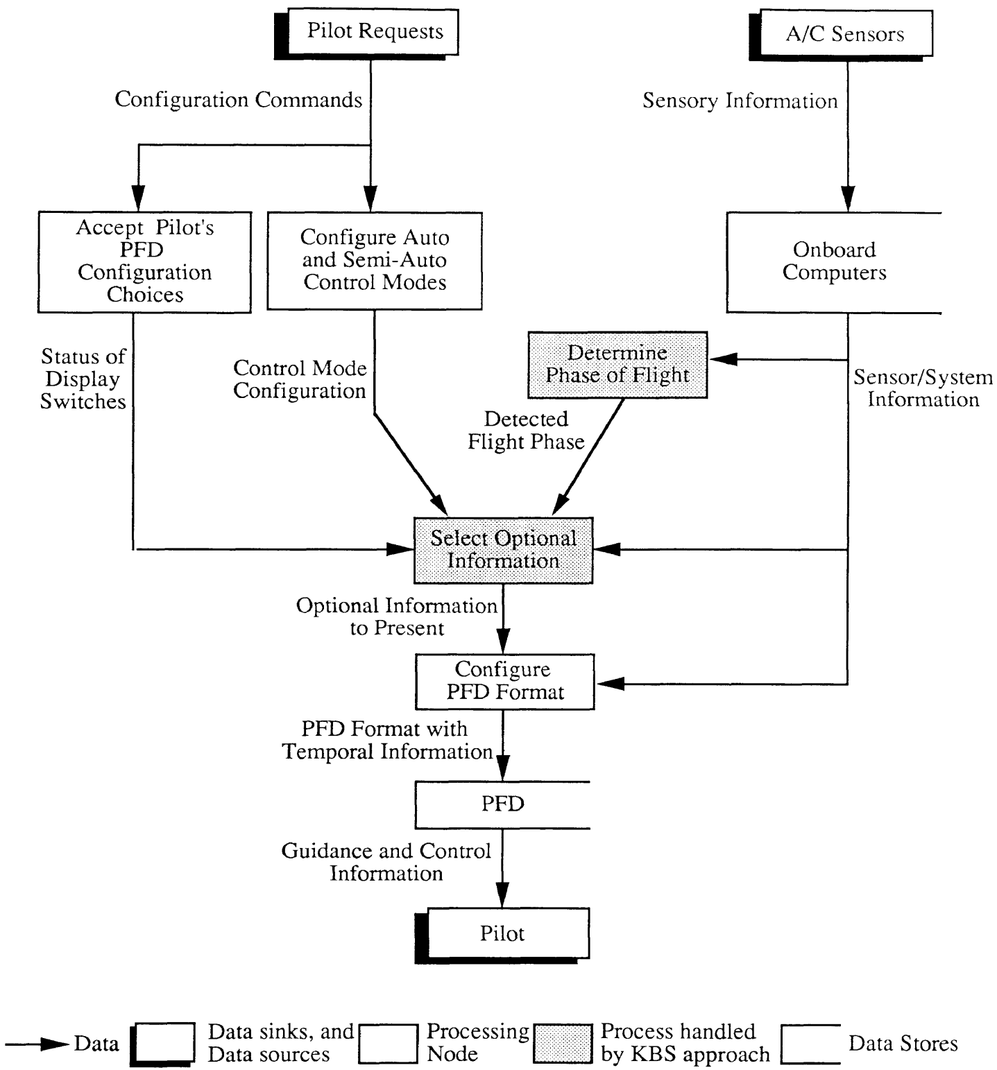
Figure 2-2 - Data-Flow Diagram of System With Automatic Flight Phase Detection
