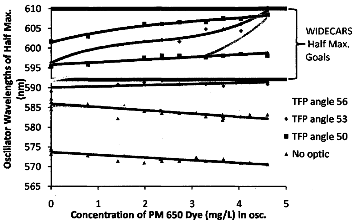
Figure 5.7: The half-maximum wavelengths versus concentrations of PM 650 added to a ~50mg/L solution of PM 597 in ethanol at different angles of incidence of the spectral selective optic, TFP. Fitted curves are added to show the general trends of the half-maximum. The shaded regions are the wavelengths of the spectra that are above the half-maximum. Wavelengths of the WIDECARS half-maximum goals are shown as thick lines.
