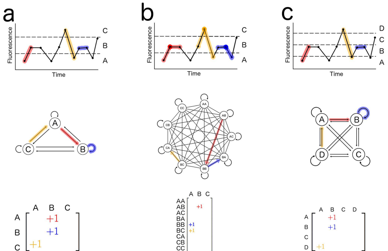
Fig 2. Illustrations of the Markov Processes which represent the observed calcium activity time series. Processes are defined with (a) n=3 and k=1 , (b) n=3 and k=2 , and (c) n=4 and k=1 . Colored transitions in the observed schematic time series are correspondingly colored as state transitions in the Markov Process below the time series, and also designated in the state transition matrices. Note that the time series are identical between (a), (b), and (c). For clarity, each line between states in the central state-transition graph of (b) is condensed to represent both a forward and a reverse state transition.
