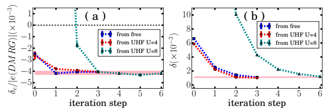
FIG. 2: Convergence of CPMC results in the self-consistent procedure. Three initial trial wave-functions are tested: free-electron and UHF solutions at U = 4t and 8t . The system is the same as in Fig. 1. In each panel, the pink band represents the converged result and error bar. In (a), the relative error in the computed ground-state energy relative to DMRG is shown vs. self-consistency iteration. The horizontal dotted line at zero is to aid the eye. Plotted in (b) are the mean square error [following the definition in Eq. (3)] in the local density computed by CPMC from the reference DMRG results.
