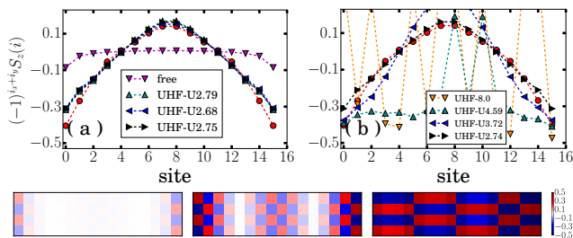
FIG. 3: Finding the optimal U_{\text{eff}} for the IP calculations during the iterations. The staggered spin density from a UHF calculation with U_{\text{eff}} is shown during each iteration of the self-consistent procedure with CPMC. The self-consistency procedure begins with the free-electron |\Psi_T\rangle in panel (a) and with the U = 8t UHF solution in (b). In the lower panel, the left, middle and right depict the spin density of the free electron wave function, the correct ground state from the converged CPMC result, and the UHF solution with U = 8t , respectively. The system is the same as in Fig. 1.
