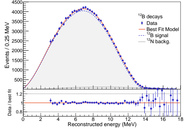
FIG. 14. (color online). Comparison of the electron energy spectrum from ^{12}\text{B} decay with simulation, including the estimated nonlinearity of the scintillator and electronics.
