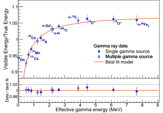
FIG. 13. (color online). Ratio of observed energy to true energy for \gamma -ray reference data relative to the estimated model of the nonlinear scintillation and Cherenkov light emission. For sources which consist of multiple \gamma -rays, the mean energy is used as an 'effective' energy for the purposes of modeling the scintillator nonlinearity. The best fit for a model of the scintillator nonlinearity is also shown (red solid line). For clarity, the estimated nonlinearity contributed by the electronics has been removed from both the data and the model.
