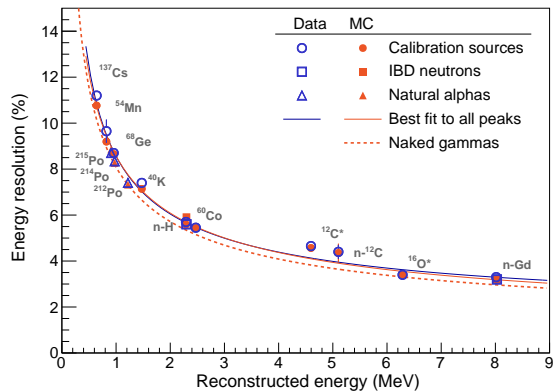
FIG. 12. (color online). Energy resolutions measured for calibration sources, neutron captures following inverse beta decay, and natural \alpha radioactivity within the scintillator (open blue markers). The detector resolution was limited by the statistical uncertainty of photoelectron counting, as modeled using Eq. 14 (blue solid line). The resolutions were consistent with Monte-Carlo simulation (solid orange markers). The simulation predicted that the intrinsic detector resolution (dashed orange line) was slightly better than that estimated for the calibration sources (solid orange line), since the latter suffered from optical shadowing by the source encapsulation. The energy resolutions for \alpha particles emitted by natural radioactivity (open blue triangles) confirmed the intrinsic energy resolution.
