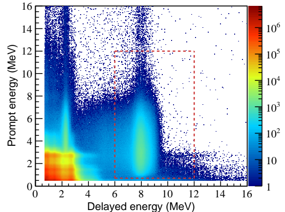
FIG. 19. (color online). The distribution of prompt versus delayed energy for signal pairs which satisfied the \bar{\nu}_e inverse beta decay selection criteria. Interactions with prompt energy of 0.7 \text{ MeV} < E_p < 12 \text{ MeV} and delayed energy of 6 \text{ MeV} < E_d < 12 \text{ MeV} were used for the neutrino oscillation analysis discussed here (red dashed box). A few-percent contamination from accidental backgrounds (symmetric under interchange of prompt and delayed energy) and ^9\text{Li} decay and fast neutron backgrounds (high prompt and \sim 8 MeV delayed energy) are visible within the selected region. Inverse beta decay interactions where the neutron was captured on ^1\text{H} provided an additional signal region with E_d \sim 2.2 MeV, albeit with much higher background.
