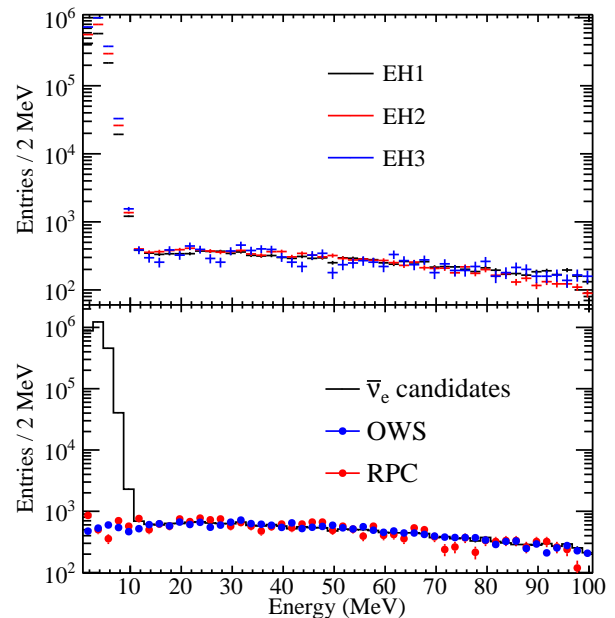
FIG. 25. (color online). ( Top ) An expanded selection of \bar{\nu}_e candidate signals with prompt energies from 0.7 MeV to 100 MeV revealed a broad continuum of background, attributed to energetic, or fast , neutrons. Actual \bar{\nu}_e signals were visible as the dominant signals below \sim 12 MeV. The energy spectra of the fast neutron background above 12 MeV were similar in all three experimental halls (EH1: black, EH2: red, EH3: blue). ( Bottom ) The sum of the \bar{\nu}_e candidate spectra from all three halls (black line) was compared to a high-purity fast neutron sample obtained by selecting those \bar{\nu}_e candidate signals which had been vetoed in the 200 \mu\text{s} after an OWS or an RPC, but not an IWS, muon signal (OWS: blue, RPC: red). The energy spectra of the vetoed samples were consistent with the background observed above 12 MeV in the \bar{\nu}_e candidate sample. The normalization of the vetoed samples were adjusted to match the \bar{\nu}_e candidates above 12 MeV. The fast neutron contamination in the \bar{\nu}_e candidate sample below 12 MeV was estimated using the vetoed sample.
