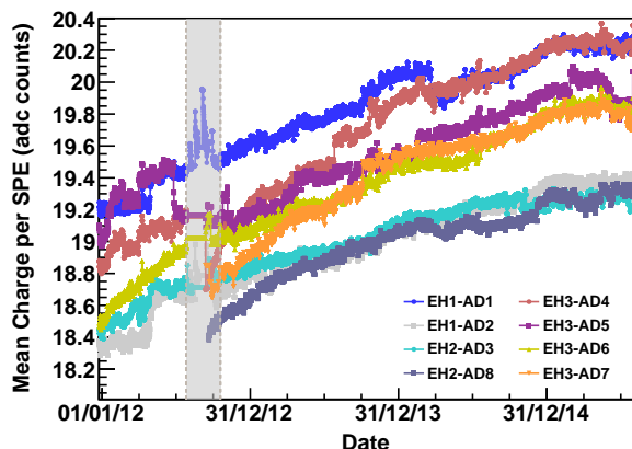
FIG. 5. (color online). Average number of ADC counts per single photoelectron, averaged over all PMT channels within each AD versus time. The shaded vertical band delineates the Summer 2012 shutdown period, during which the high-voltage mainframes were frequently power-cycled and data-taking was partially interrupted for installation activities.
