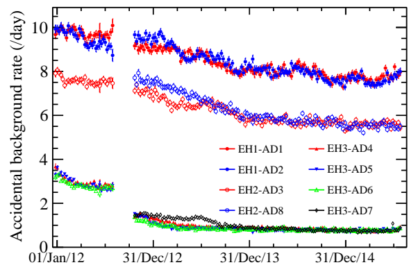
FIG. 23. (color online). The accidental background rate for selection A as a function of time for each antineutrino detector, as calculated from measurements of the rates of uncorrelated signals which satisfy the prompt \bar{\nu}_e signal selection, R_p , and delayed \bar{\nu}_e signal selection, R_d . The accidental rate primarily depended on experimental hall depth due to the relative rate of unstable isotope production by muons. The decline of the accidental background versus time was due to combination of a decrease in the natural radioactivity following detector installation and a reduction of the neutron emission by the ^{241}\text{Am} - ^{13}\text{C} calibration sources. R_p was sensitive to small changes in electrical noise, which resulted in the observed instability in the accidental background rate. Installation of the final two detectors in the summer of 2012 is evident as a gap during this time. Removal of two of the three ^{241}\text{Am} - ^{13}\text{C} sources in each far detector during the installation period reduced the accidental background rate by \sim 50\% .
