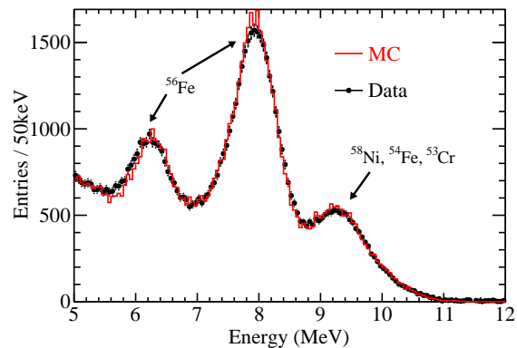
FIG. 28. (color online). Uncorrelated individual signals with E_{\text{rec}} > 5 MeV generated by a \sim 59 Hz ^{241}\text{Am} - ^{13}\text{C} neutron source temporarily installed on the lid of EH3-AD5 (black points). Peaks in the spectra are attributable to neutron capture on Fe, Cr, or Ni nuclei present in stainless steel of the lid, where an energetic capture \gamma -ray subsequently penetrates to the scintillating region of the detector. The measurement was used to benchmark a Monte-Carlo simulation of the uncorrelated and correlated background induced by this source (red solid line), and thereby estimate the correlated background induced by the regular weak \sim 0.7 Hz ^{241}\text{Am} - ^{13}\text{C} sources present in the automated calibration units (ACUs), also on the detector lid.
