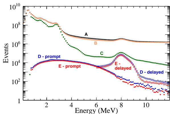
FIG. 16. (color online). Reconstructed energy spectra of all signals in EH1-AD1 as successive cuts from selection A were applied: (A) all signals, (B) rejection of signals from PMT light emission, (C) Water Shield muon veto, (D) IBD signal pair selection: prompt energy, delayed energy, prompt-delayed time separation, and multiplicity veto, and (E) AD muon and shower vetos. The spectra E are the final prompt and delayed energy spectra of the \bar{\nu}_e candidates for EH1-AD1.
