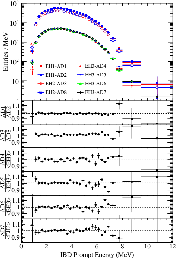
FIG. 34. (color online). (Top) Distributions of the reconstructed prompt energy for the selected \bar{\nu}_e candidates in each of the eight detectors. (Bottom) The ratio of the distributions for detectors within the same experimental hall showed no significant deviations between detectors.
