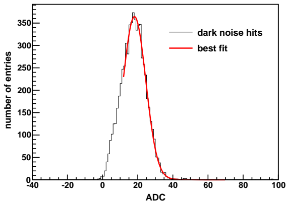
FIG. 4. (color online). Example of the baseline-subtracted ADC charge distribution of uncorrelated PMT signals modeled using Eq. 6.
