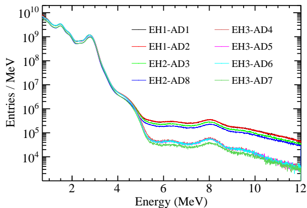
FIG. 22. (color online). The reconstructed energy spectra of isolated uncorrelated signals for all eight detectors. The prompt-like signal rate was dominated by natural radioactivity with energies below 3 MeV. The delayed-like signal rate was dominated by beta decay of muon-induced unstable isotopes, mainly ^{12}\text{B} , and \gamma -rays from capture of ^{241}\text{Am} - ^{13}\text{C} calibration source neutrons on materials at the top of each detector. The energy spectrum of the accidental background prompt signals in each AD were equivalent to these distributions.
