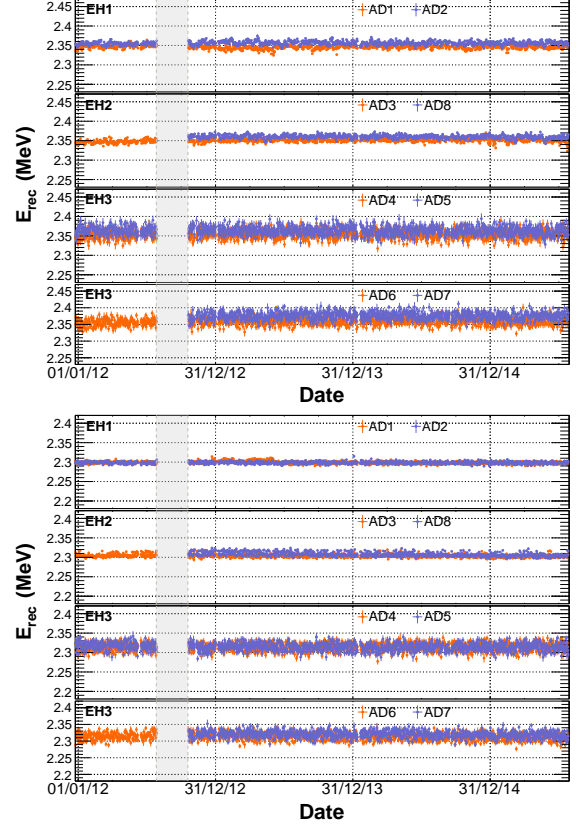
FIG. 10. (color online). Top : Stability of the mean reconstructed energy of signals from spallation neutron capture on H versus time, obtained from calibration using a ^{60}\text{Co} source located at the detector center (reconstruction A). Bottom : The same, but for the calibration method which relies on spallation neutrons (reconstruction B). Each point corresponds to one day. The shaded vertical band represents the 2012 shutdown period.
