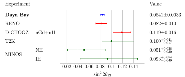
FIG. 42. (color online). Comparison of measurements of \sin^2 2\theta_{13} : this measurement (blue point); RENO [73] and Double Chooz [74] (red points); T2K [75] and MINOS [76] (green points). The T2K and MINOS values were deduced from 2\sin^2 \theta_{23} \sin^2 \theta_{13} , and are presented for the two cases of the normal (upper) and inverted (lower) mass hierarchy. The MINOS measurement assumed \sin^2 \theta_{23} = 0.5 , \delta_{CP} = 0 , while the T2K measurement marginalized over these unknown parameters.
