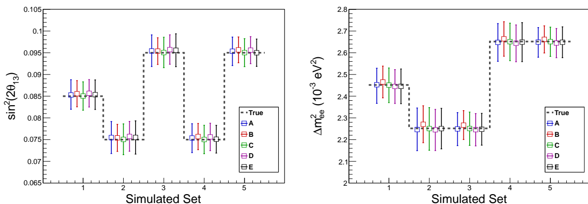
FIG. 36. (color online). Results of a validation study of the independent statistical methods (A through E) used to compare observation with the three-flavor model of neutrino oscillation. An independent program was used to generate fake observations under the assumption of a range of true values for the oscillation parameters \theta_{13} and |\Delta m_{ee}^2| (grey dashed lines). All methods demonstrated a consistent unbiased estimation of the true input parameters (colored points) for \theta_{13} (left panel) and |\Delta m_{ee}^2| (right panel). The final estimated total uncertainties, given by the error bars on each point, were also consistent between methods.
