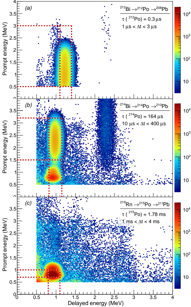
FIG. 30. (color online). The distributions of low-energy prompt versus delayed reconstructed energy for the time intervals (a) 1 \mu\text{s} to 3 \mu\text{s} , (b) 10 \mu\text{s} to 400 \mu\text{s} , and (c) 1 \text{ms} to 4 \text{ms} for all detectors combined. The distributions revealed time-correlated signal pairs from actinide contamination in the GdLS regions of each detector. While these interactions were not a background for \bar{\nu}_e detection, the resulting estimates of actinide \alpha -particle activity constrained potential background from subsequent ^{13}\text{C}(\alpha, n)^{16}\text{O} interactions.
