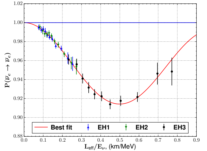
FIG. 40. (color online). Measured reactor \bar{\nu}_e spectral distortion, displayed as the oscillation survival probability versus L_{\text{eff}}/E_\nu . The effective propagation distance L_{\text{eff}} was estimated for each hall based on the distribution of reactors contributing to the signal (see Eq. 56). The average true \bar{\nu}_e energy \langle E_\nu \rangle was determined for each bin in the prompt positron spectrum based on the model of the detector response. The \bar{\nu}_e survival probability was given by the observed signal in each bin divided by the prediction assuming no oscillation. The measurement sampled \bar{\nu}_e survival over almost one full cycle, demonstrating distinct evidence in support of neutrino flavor oscillation.
