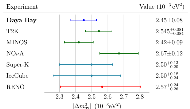
FIG. 43. (color online). Comparison of measurements of \Delta m_{32}^2 : this measurement (blue point); RENO [73] (red point); T2K [75], MINOS [77], and NO \nu A [78] (green points); Super-Kamiokande [79] and IceCube [80] (cyan points). All values are given for the case of the normal mass hierarchy; the comparison for the inverted ordering was qualitatively similar.
