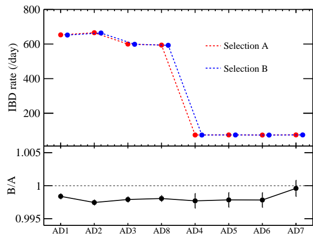
FIG. 32. (color online). (Top) The rates of \bar{\nu}_e inverse beta decay observed in each antineutrino detector, for both selection A and selection B. (Bottom) The rates obtained by selection B were \sim 0.2\% lower than those of selection A, demonstrating a difference in absolute selection efficiency within expectations. The ratio of the far versus near detector rates are consistent for the two selections, considering the statistical uncertainty from candidate signals uncommon between the two samples.
