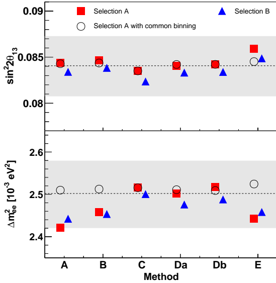
FIG. 39. (color online). A comparison of the estimated values of \sin^2 2\theta_{13} (top) and \Delta m_{ee}^2 (bottom) obtained using various combinations of the two selected \bar{\nu}_e samples, statistical methods, and reactor \bar{\nu}_e flux models. The horizontal dashed lines show the best estimate of each parameter, while the gray regions show the \pm 1\sigma confidence interval from the reference results (selection A, method D, and the Huber-Mueller reactor flux model). The \lesssim 1\sigma offsets for methods A, B, and E were due to their choice of binning of the prompt energy spectrum, particularly below 1.3 MeV. When all methods used the same binning as method C, consistent results were obtained (open circles). See the text for details.
