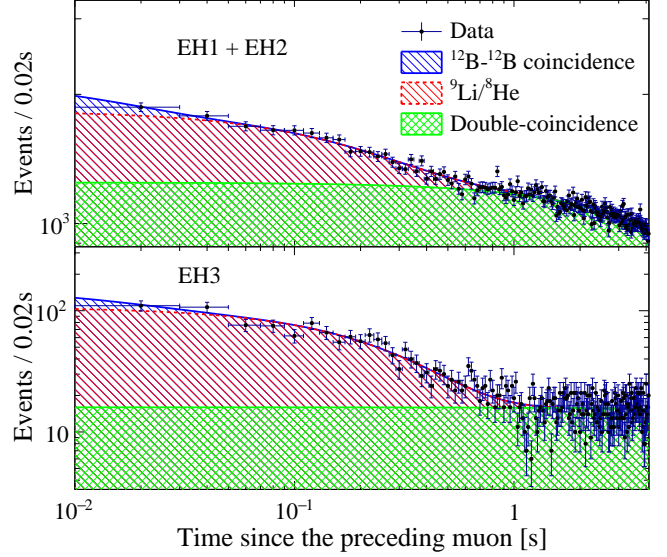
FIG. 26. (color online). The distribution of \bar{\nu}_e inverse beta decay candidates versus time since the most recent muon-induced particle shower ( E_{\text{rec}} > 2.5 \text{ GeV} ) in the same detector (blue points). A fit to this distribution statistically distinguishes the muon-uncorrelated \bar{\nu}_e and accidentals (green hatched region), from the muon-correlated background from \beta -n decay (red lined region). A minor contribution from accidental background, where the delayed signal was from ^{12}\text{B} \beta decay, is barely visible in the first bin (blue lined region). A more restrictive \bar{\nu}_e selection of 3.5 \text{ MeV} < E_p < 12 \text{ MeV} , and 1 \mu\text{s} < \Delta t < 100 \mu\text{s} suppressed the accidental contribution, providing a more precise estimate of the \beta -n background.
