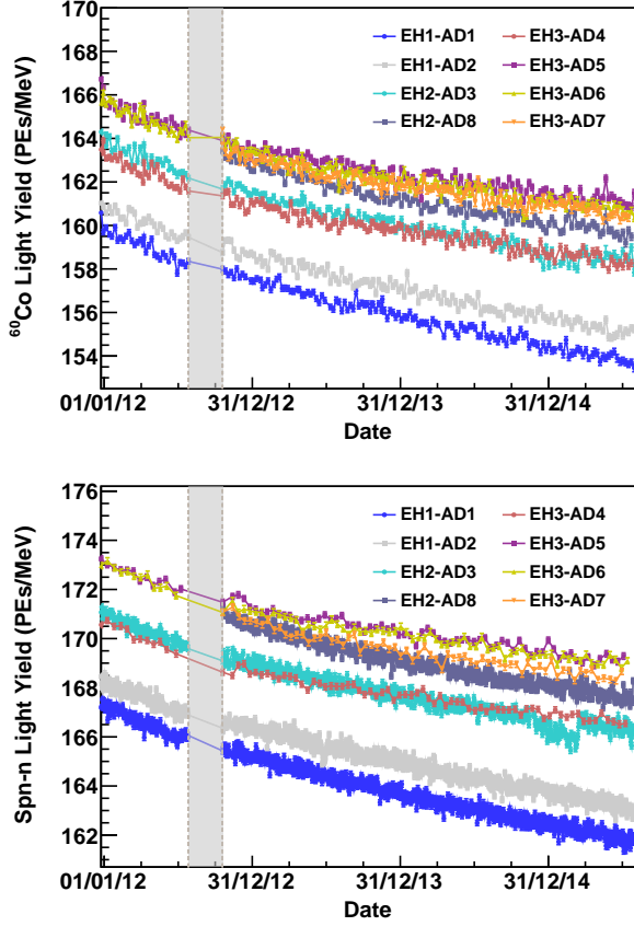
FIG. 6. (color online). Top : Observed light yield versus time, in units of observed photoelectrons (PEs) per MeV, as obtained using weekly deployments of a ^{60}\text{Co} source at the center of each detector. Bottom : Observed light yield obtained using spallation neutron capture on Gd distributed throughout the target volume. A consistent \sim 1\% per year decline in the light yield was observed for all detectors. The offset in light yield between these two calibration references was due to the nonlinear response of the detectors. The vertical shaded band indicates the summer 2012 shutdown period, during which data-taking was partially interrupted for installation of the final two detectors.
