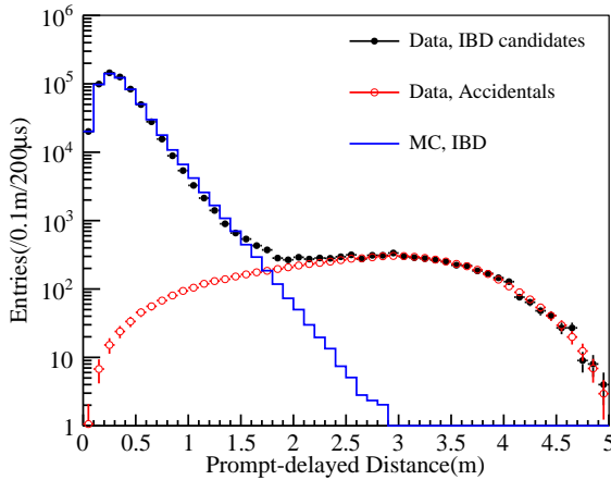
FIG. 24. (color online). Distribution of distances between the reconstructed positions of the prompt and delayed signals of the antineutrino inverse beta decay candidate signals from all detectors (black points). The positions were highly correlated for true \bar{\nu}_e interactions, as demonstrated by Monte-Carlo simulation (blue line). Repeating the selection of \bar{\nu}_e interactions, but with the time window for selection of the delayed signals offset by 1 ms to 20 ms, enhanced the uncorrelated accidental background (red points) and suppressed correlated signals. The consistency of the distributions confirmed the estimate of contamination by accidental backgrounds, which varied from 1% to 2% depending on detector.
