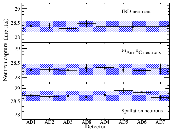
FIG. 18. (color online). Comparison of the capture time of neutrons on Gd measured in each detector, for neutrons from IBD, ^{241}\text{Am} - ^{13}\text{C} , and muon spallation. The IBD neutron data is combined for the four detectors in EH3 (AD4–AD7) in order to reduce the statistical uncertainty. The observed capture times vary by less than \pm 0.2\mu\text{s} between detectors (blue band). The spatial distributions of neutrons emitted by these sources differed, introducing slight offsets in their absolute capture times.
