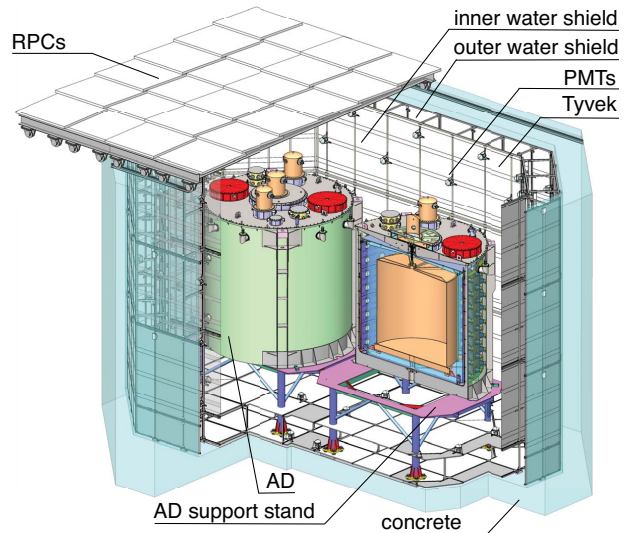
FIG. 3. (color online). Diagram of a near site detector system. Two ADs were immersed in a water Cherenkov muon detector which functioned as both a passive radiation shield and an active muon tag. Tyvek sheets divided the pool into two optically separate detectors, the inner and outer water shields. An RPC system covered the pool, providing additional muon identification.
