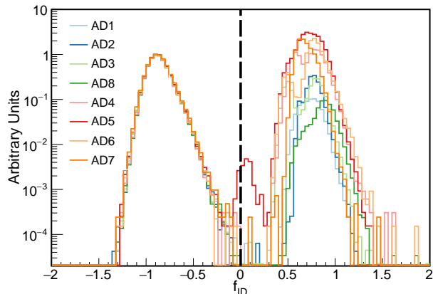
FIG. 21. (color online). Distributions of the discriminator f_{\text{ID}} for all inverse beta decay delayed signal candidates from the eight detectors. The distributions are normalized to the number of antineutrino candidates for each AD. This demonstrates the consistency of these distributions among the ADs for genuine antineutrino candidates ( f_{\text{ID}} < 0 ). This normalization artificially enhances the magnitude of the light-emission background distributions ( f_{\text{ID}} \geq 0 ) for the far (AD4–AD7) relative to the near ADs. These background distributions differed between detectors depending on the characteristics of the light-emitting PMTs in each AD.
