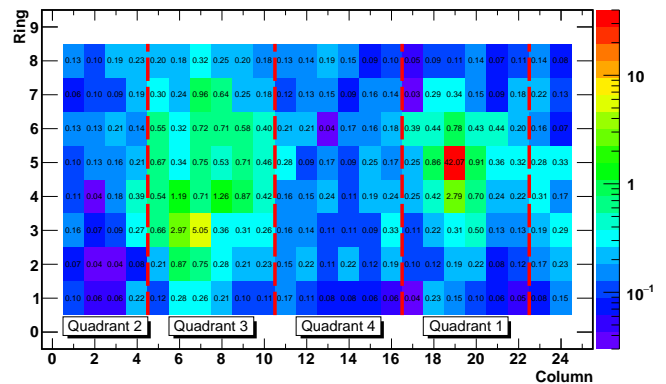
FIG. 20. (color online). Typical charge distribution from PMT light emission. The 8 ring by 24 column cylindrical PMT array has been projected onto a plane. The logarithmic color scale, as well as numbers, provides the percentage of the total signal charge observed by each PMT. In this example, light was emitted by the PMT at column 19 in ring 5. The discharging PMT and those PMTs directly opposite in Quadrant 3 observed a significant fraction of the total charge. The distinct charge pattern allowed efficient rejection of this instrumental background.
