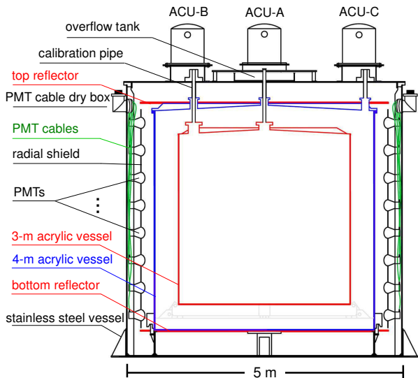
FIG. 2. (color online). Cross-sectional diagram of an antineutrino detector (AD). Scintillation light was produced when a reactor \bar{\nu}_e interacted within the central 20-ton GdLS target, which was contained in a transparent acrylic vessel. The target was nested within an additional 20-tons of pure LS to increase efficiency for detection of gamma rays produced within the target. Scintillation light was detected by 192 photomultipliers mounted on the inner circumference of a 5 m by 5 m stainless steel vessel, which was filled with mineral oil (MO).
