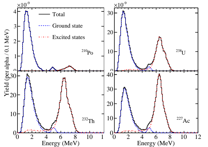
FIG. 31. (color online). Simulation of energy spectra of the prompt signals for the ^{13}\text{C}(\alpha, n)^{16}\text{O} background, for each of the primary sources of natural \alpha activity in the detectors. Energetic neutrons produced a broad peak from proton recoils below 4 MeV, and a small peak near 5 MeV from inelastic scattering on ^{12}\text{C} . Higher-energy \alpha -particles increasingly populated the excited states of ^{16}\text{O} , resulting in a broad peak from 5 MeV to 8 MeV from ^{16}\text{O}^* de-excitation.
