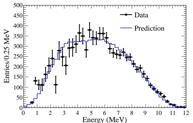
FIG. 27. (color online). A comparison of the observed (black points) and predicted (blue line) prompt reconstructed energy spectrum from {}^9\text{Li} \beta -n decay. The observed spectrum was obtained from those \bar{\nu}_e candidate interactions which followed muon-induced particle showers, with the expected background from \bar{\nu}_e and accidentals subtracted. The prediction was estimated considering the known \beta -n decay branches and contribution from the nuclear break-up to a neutron and two \alpha 's.
