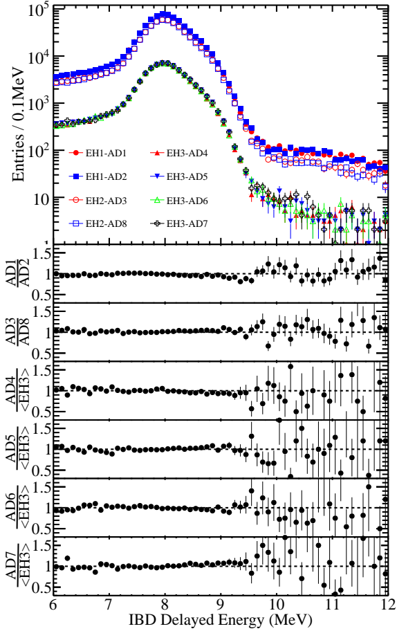
FIG. 35. (color online). (Top) Distributions of the reconstructed delayed energy for the selected \bar{\nu}_e candidates in each of the eight detectors. (Bottom) The ratio of the distributions for detectors within the same experimental hall showed no significant deviations between detectors; the slight slopes in the ratios are consistent with the \lesssim 0.2\% relative differences in the energy scale among the detectors.
