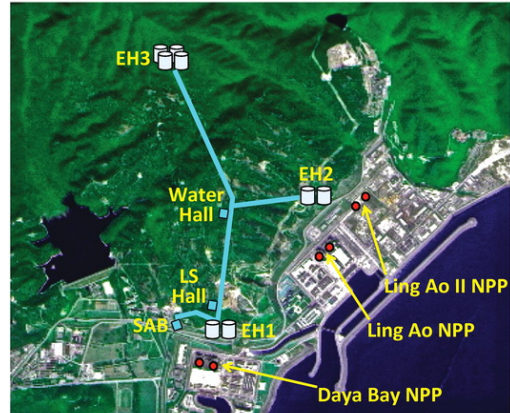
FIG. 1. (color online). Layout of the Daya Bay experiment. The Daya Bay and Ling Ao nuclear power plant (NPP) reactors (red circles) were situated on a narrow coastal shelf between the Daya Bay coastline and inland mountains. Two antineutrino detectors installed in each underground experimental hall near to the reactors (EH1 and EH2) measured the \bar{\nu}_e flux emitted by the reactors, while four detectors in the far experimental hall (EH3) measured a deficit in the \bar{\nu}_e flux due to oscillation. The detectors were built and initially tested in a surface assembly building (SAB), transported to a liquid scintillator hall (LS Hall) for filling, and then installed in an experimental hall.
