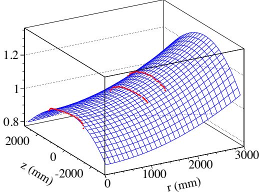
FIG. 7. (color online). Variation in light yield versus vertical ( z ) and radial ( r ) position of an interaction within EH1-AD1 for reconstruction A (blue surface). The functional form of the variation f_b(z,r) was motivated by simulation, and constrained using the relative light yield of ^{60}\text{Co} calibration data from ACU A ( r=0 mm), ACU B ( r=1350 mm) and ACU C ( r=1772.5 mm) (red points). While the modeled correction was between -6\% to 17\% over the volume of a detector, only slight differences ( <3.2\% ) were observed between the eight detectors.
