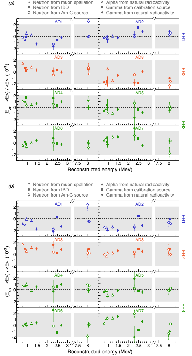
FIG. 11. (color online). Comparison of the mean reconstructed energy between antineutrino detectors for a variety of calibration references using (a) calibration with ^{60}\text{Co} sources (reconstruction A) and (b) calibration with spallation neutrons (reconstruction B). E_{\text{AD}} is the reconstructed energy determined for each AD, while \langle E \rangle is the eight-detector average. The mean energy for each calibration reference was obtained from the corresponding peak in the energy spectrum of all regular data (natural alphas and gammas, neutrons from IBD and muon spallation) and all weekly calibration runs (gammas from ^{68}\text{Ge} and ^{60}\text{Co} sources, neutrons from Am-C sources) taken during the time period when all eight ADs were in operation. An effective fiducial volume selection has been applied on distributed sources to suppress interactions outside the antineutrino target where AD-to-AD differences are larger. Error bars are statistical only, and systematic variations between detectors for all calibration references were <0.2\% for both reconstruction methods.
