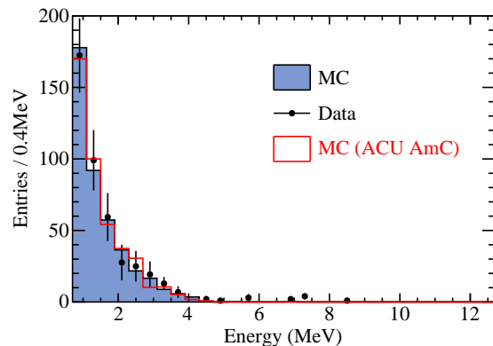
FIG. 29. (color online). The prompt reconstructed energy spectrum from correlated \bar{\nu}_e -like signal pairs induced by a \sim 59 Hz ^{241}\text{Am} - ^{13}\text{C} neutron source temporarily installed on the lid of EH3-AD5 (black points). Inelastic collisions of a neutron with nuclei present in stainless steel produced \gamma -rays which occasionally penetrated to the scintillating region of the detector, generating signals with a steeply-falling energy spectrum. A benchmarked Monte-Carlo simulation predicted a consistent spectrum (solid blue region). The prompt energy spectrum for correlated background from the regular \sim 0.7 Hz ^{241}\text{Am} - ^{13}\text{C} sources present in the automated calibration units (ACUs) was estimated to be identical, within the statistical precision of the simulation (red line).
