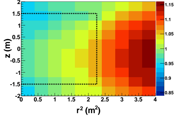
FIG. 8. (color online). Variation in light yield versus vertical ( z ) and radial ( r^2 ) position of neutron capture interactions within EH1-AD1 for reconstruction B. Each pixel shows the ratio of the observed light yield over the average for the entire GdLS region. The dashed lines indicate the boundary between the GdLS and LS regions. Neutrons which captured on Gd were used for the innermost GdLS region, while neutrons captured on hydrogen were used for the outermost LS region. Only slight differences ( <3.0\% ) in the nonuniformity were observed between the eight detectors.
