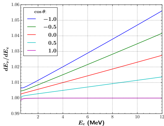
FIG. 44. (color online). The Jacobian dE_\nu/dE_{\text{true}} as a function of positron energy E_e for a range of values of the positron emission angle \cos \theta_e .
