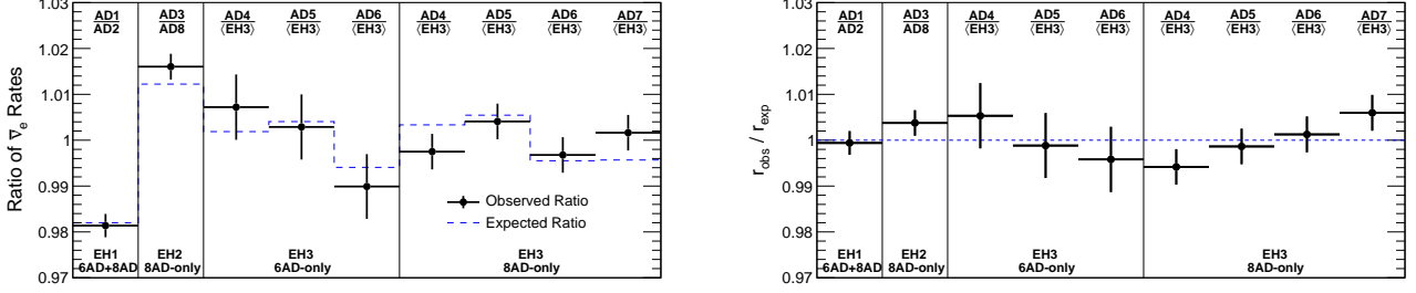
FIG. 33. (color online). ( Left ) Ratios of the \bar{\nu}_e interaction rates observed by detectors within the same experimental hall, r_{\text{obs}} (black points). The ratio of the rate in AD1 to that of AD2 is shown for EH1 for the entire data period. For the period following installation of AD8 in EH2, the ratio of AD3 to AD8 is provided. For EH3, the ratio of the rate in each detector relative to the site average is given separately for the period before and after installation of AD7. Slight differences in the distances of each detector relative to each reactor as well as small variations in detector target mass \Delta N_p predicted minor deviations in these ratios, r_{\text{exp}} (blue dashed line). The uncertainties are dominated by statistics and the estimated 0.13% variation in efficiency between detectors. The consistency of the side-by-side detector rates confirmed the stringent limits on this latter systematic uncertainty. ( Right ) The same figure, expressed as the double ratio r_{\text{obs}}/r_{\text{exp}} .
