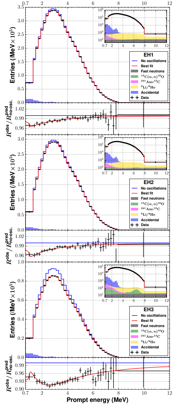
FIG. 38. (color online). Reconstructed positron energy spectra for the \bar{\nu}_e candidate interactions (black points). The spectra of the detectors in each experimental hall are combined: EH1 (top), EH2 (middle), and EH3 (bottom). The best-fit three-flavor neutrino oscillation model (red line) is determined from the difference in rate and spectrum observed at the far hall relative to the near halls. A prediction with no oscillation (blue line) is obtained from the best-fit model, but with \theta_{13} = 0 . The inset in semi-logarithmic scale shows the ratio of the background-subtracted spectra to prediction with no oscillation is shown in the panel beneath each energy spectrum.
