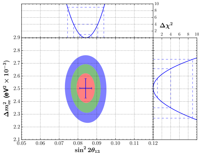
FIG. 41. (color online). Confidence regions of \sin^2 2\theta_{13} and |\Delta m_{ee}^2| from a combined analysis of the prompt positron spectra and rates. The 1\sigma , 2\sigma , and 3\sigma 2-D confidence regions are estimated using \Delta\chi^2 values of 2.30 (red), 6.18 (green), and 11.83 (blue) relative to the best fit. The upper panel provides the 1-D \Delta\chi^2 for \sin^2 2\theta_{13} obtained by profiling |\Delta m_{ee}^2| (blue line), and the dashed lines mark the corresponding 1\sigma , 2\sigma , and 3\sigma intervals. The right panel is the same, but for |\Delta m_{ee}^2| , with \sin^2 2\theta_{13} profiled. The point marks the best estimates, and the error bars display their 1-D 1\sigma confidence intervals.
