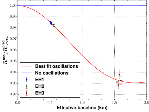
FIG. 37. (color online). Ratio of the detected \bar{\nu}_e signal to that expected assuming no oscillation versus the effective baseline for all eight antineutrino detectors. Oscillation due to \theta_{13} introduced a deficit in the far detectors relative to the near detectors, and the best-fit three-flavor oscillation model from the rate-only analysis is shown (red line). Extrapolation of the model to a baseline of zero determined the absolute normalization of the reactor \bar{\nu}_e flux, R^{\text{pred}}(L=0) . The points representing the near (far) detectors are displaced by \pm 6 m ( \pm 30 m) for clarity.
