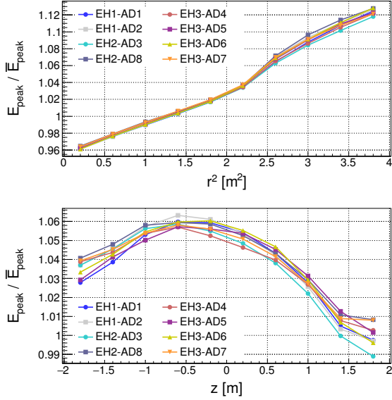
FIG. 9. (color online). Variation in light yield versus radial ( top ) and vertical ( bottom ) position of neutron capture interactions for reconstruction B. Each point shows the ratio of the observed light yield over the average for the entire the GdLS region. The variation was primarily due to the optical acceptance versus position, and was reproduced by optical simulation. Only slight differences ( <3.0\% ) in the nonuniformity were observed between the eight detectors.
