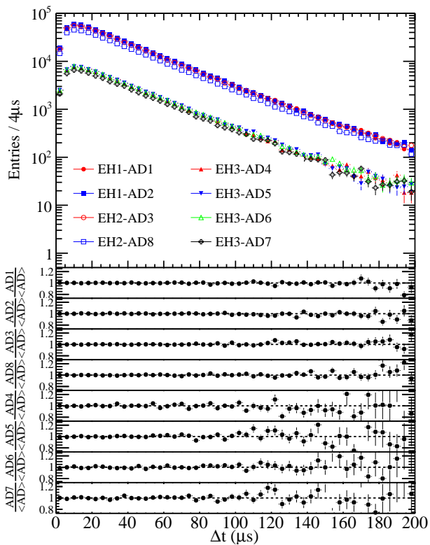
FIG. 17. (color online). (Top) Distribution of the time separation between prompt and delayed \bar{\nu}_e inverse beta decay interaction candidates for each detector. (Bottom) Ratio of the observed distribution to the normalized average for all eight detectors. The consistency of these distributions constrained potential systematic variation in the fraction of IBD neutrons which captured on Gd among the eight detectors.
