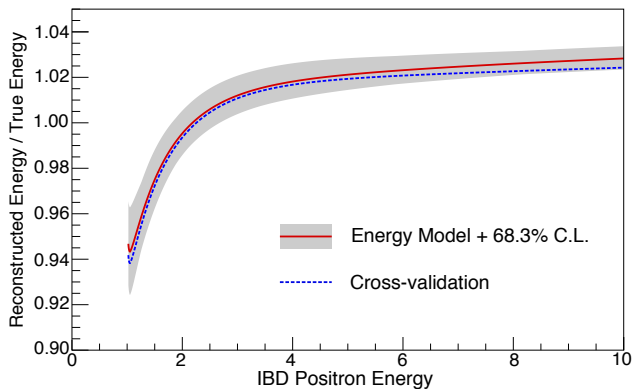
FIG. 15. (color online). Estimated ratio of reconstructed over true energy, E_{\text{rec}}/E_{\text{true}} , for positron interactions totally contained within the antineutrino detector target (red solid line). The two 0.511-MeV \gamma -rays from positron annihilation were included in the energy. The resulting 68% C.L. region (gray shaded band) constrains this ratio to better than 1% over most of the energy range of interest. An independent estimate, which relied on the \beta+\gamma spectra from bismuth and thallium decay as well as the Michel electron spectrum endpoint, produced a consistent model (blue dotted line).
