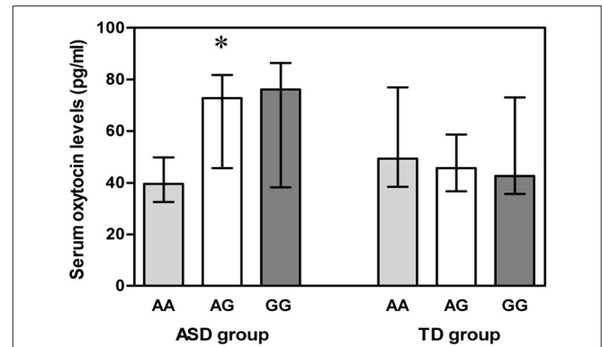
FIGURE 2 | Vertical bar charts of serum oxytocin levels for the three OXTR SNP rs2254298 genotypes in both ASD and TD groups are presented as median (IQR). Error bars show interquartile range (IQR). ASD group: n = 9 AA, n = 21 AG, and n = 25 GG. TD group: n = 9 AA, n = 52 AG, and n = 49 GG. The ASD subjects exhibited a significant association between serum oxytocin levels and three OXTR SNP rs2254298 genotypes, and serum oxytocin levels were low in ASD subjects with an AA genotype. p < 0.05 . ASD, autism spectrum disorders; IQR, interquartile range; OXTR, oxytocin receptor; SNP, single-nucleotide polymorphism; TD, typically developing.
