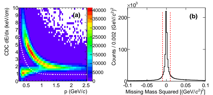
FIG. 2. (color online) (a) Energy loss dE/dx versus positively charged track momentum and (b) the spectrum of missing mass squared for the reaction \tilde{\gamma}p \rightarrow p\gamma\gamma .
