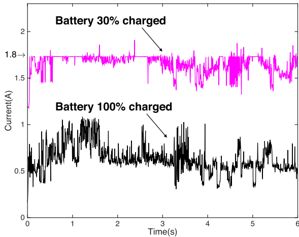
Fig. 4. Power traces obtained while loading the same webpage (yahoo.com) with 30% and 100% battery level. The figure shows that the trace corresponding to 100% battery level exhibits a relatively higher dynamic range, because it is not capped by the 1.8 A limit which is often reached by the trace corresponding to 30% battery level.
