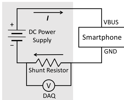
Fig. 1. Overview of the setup used to collect power traces.
