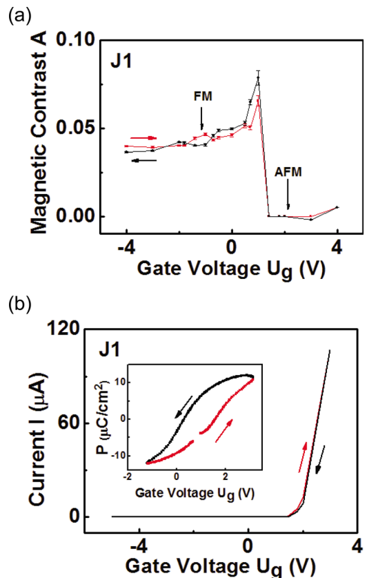
FIG. 2. (Color online) (a) MSHG magnetic contrast A as a function of gate voltage U_g from BTO/LCMO/LSMO heterostructure (J1). (b) I-V curve measured from sample J1 at 78 K. Decreasing (increasing) gate voltages are labeled in black (red). The inset shows the ferroelectric polarization ( P ) in BTO as a function of U_g measured at 78 K. The direction of positive P is defined as pointing away from LSMO electrode.
