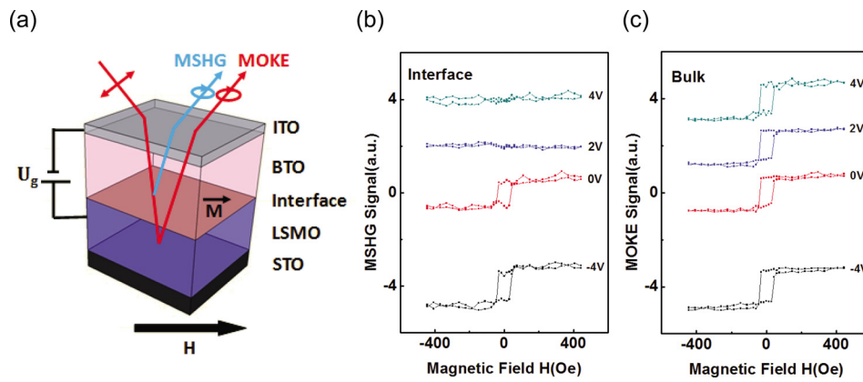
FIG. 1. (Color online) (a) Schematic depiction of MSHG and MOKE measurement—MOKE measures the bulk magnetization of the LSMO film, while MSHG selectively probes the interface magnetization only. (b) Interface and (c) bulk magnetic hysteresis loops from BTO/LCMO/LSMO heterostructure (J1) for different external gate voltages U_g measured with MSHG and MOKE techniques at 78 K, respectively.
