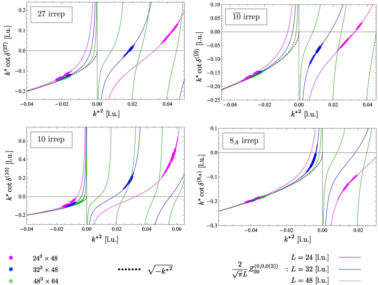
FIG. 8. k^* \cot \delta values in the two-baryon channels belonging to the four irreps 27, \overline{10} , 10 and 8_A , obtained by solving Eq. (2) at the corresponding values of the square of the CM momentum of the two baryons, k^{*2} . The functions on the left-hand side of this equation for l = m = 0 , i.e., \frac{2}{\sqrt{\pi}L} \mathcal{Z}_{00}^d[1; (k^*L/2\pi)^2] , are also shown at the corresponding volumes and CM boost momenta. The thick points cover the statistical uncertainty in the results, while the thin points cover the statistical and systematic uncertainties combined in quadrature. Quantities are expressed in lattice units (l.u.).
