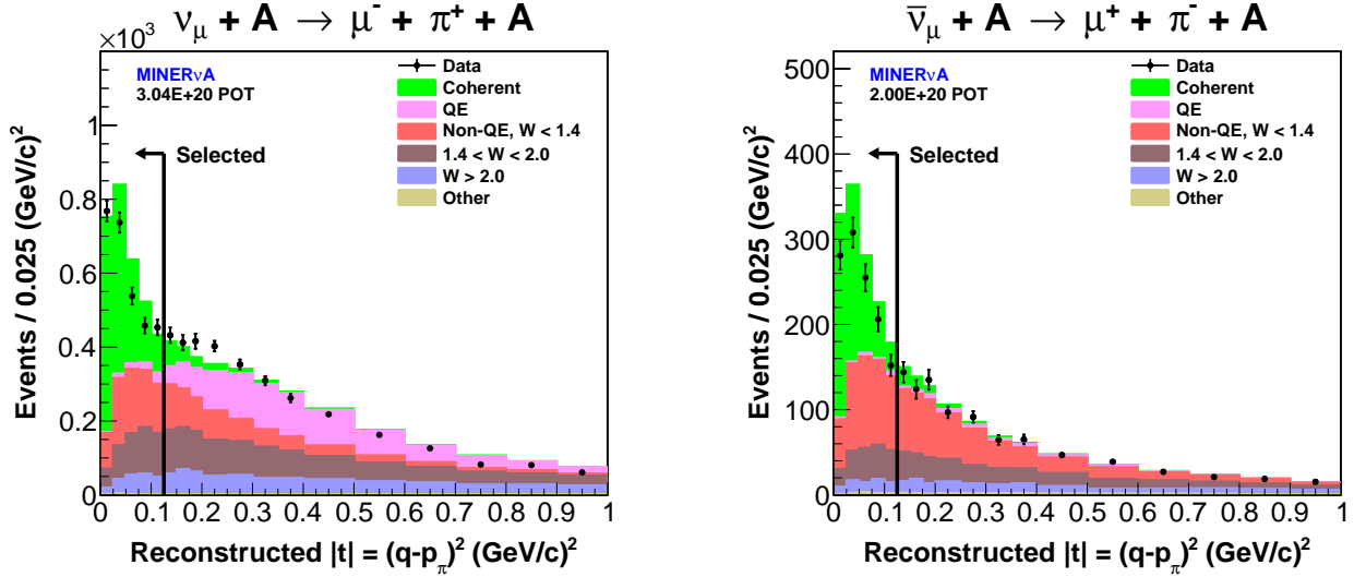
FIG. 15. The \nu_\mu (left) and \bar{\nu}_\mu (right) |t| distributions, after background tuning, for events passing all cuts up through the E_{vtx} cut. Events with |t| < 0.125 ( \text{GeV}/c ) 2 are selected.
