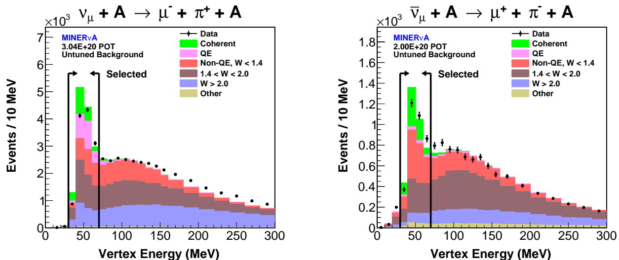
FIG. 14. The left (right) plot shows the E_{vtx} distribution for events in the \nu_\mu ( \bar{\nu}_\mu ) sample that pass all selection cuts up through the proton score ( E_\nu ) cut. Events in the range 30 < E_{vtx} < 70 MeV are selected.
