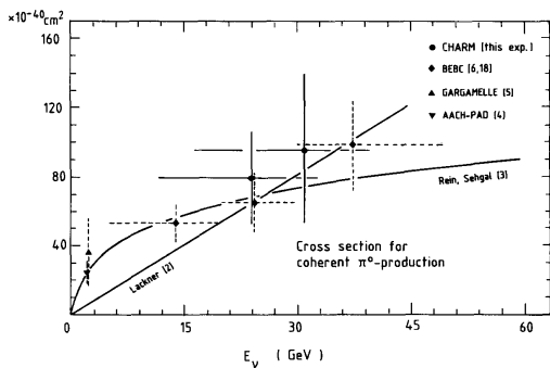
FIG. 3. Early measurements of the NC coherent pion production cross section. The horizontal error bars represent the range of neutrino energies sampled by the measurement. The figure is from [18].
