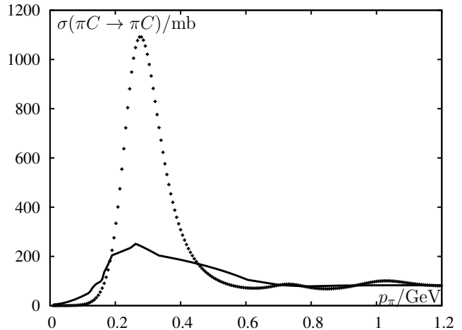
FIG. 2. The Rein-Sehgal (dashed line) and Berger-Sehgal (solid line) pion-carbon elastic scattering cross sections as a function of the pion momentum in the laboratory frame. From [12].
