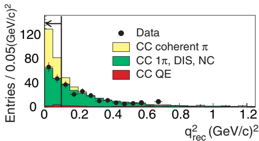
FIG. 5. The data and simulated Q^2 distributions for \nu_\mu CC coherent pion production candidates at K2K. The figure is from [31].
