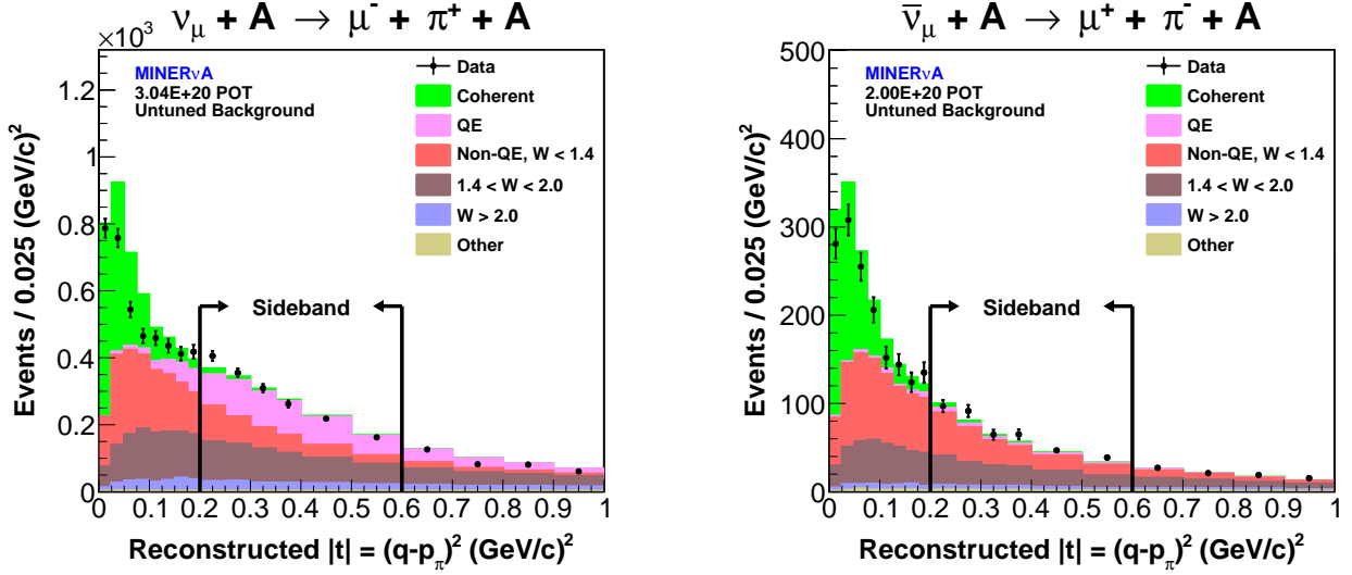
FIG. 16. The \nu_\mu (left) and \bar{\nu}_\mu (right) |t| distributions, before background tuning, for events that pass all selection cuts through the vertex energy and proton score cuts. The sideband used for the background tuning are events with 0.2 < |t| < 0.6 ( \text{GeV}/c ) 2 .
