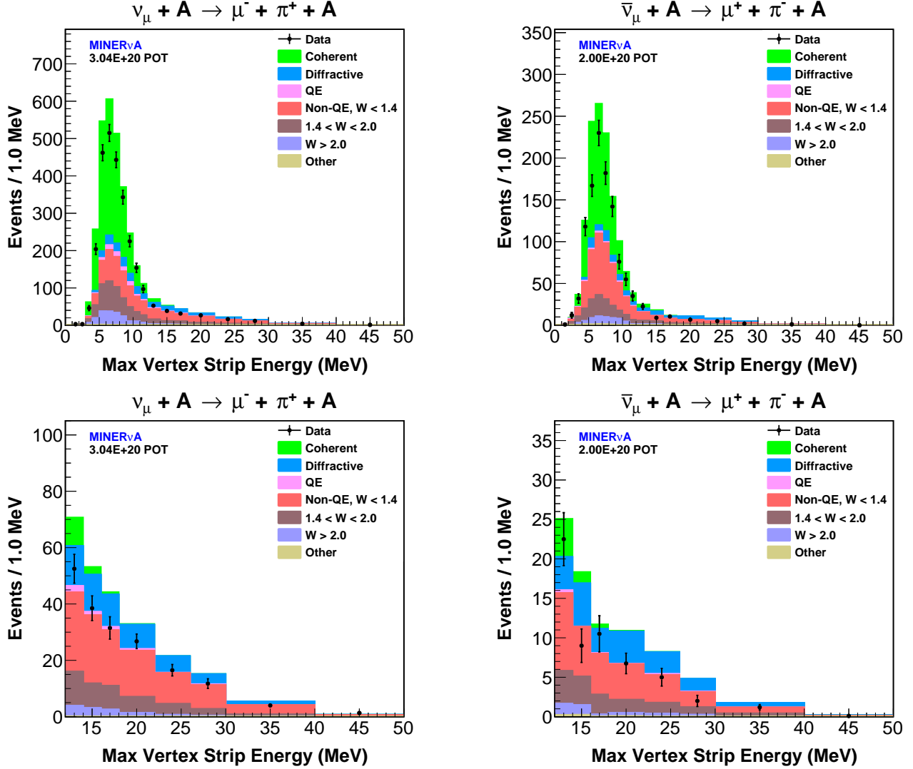
FIG. 34. The MVSE distribution for the \nu_\mu (left) and \bar{\nu}_\mu (right) selected coherent-like samples. The bottom plots show the high-MVSE region examined for the presence of diffractive scattering. The non-diffractive background normalizations are tuned. The added diffractive MC sample shown is for 0.2 relative diffractive-to-coherent normalization, which is clearly inconsistent with the data. The fitted \nu_\mu ( \bar{\nu}_\mu ) relative diffractive-to-coherent normalization is +0.01 \pm 0.08 ( -0.03 \pm 0.09 ).
