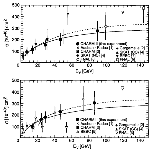
FIG. 4. Early measurements of the \nu_\mu (top) and \bar{\nu}_\mu (bottom) CC coherent pion production cross sections. The solid line is the Rein-Sehgal model prediction. The figure is from [30].
