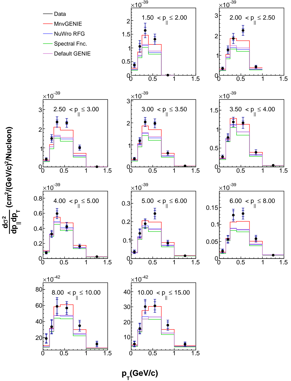
FIG. 22: Double-differential QE-like cross section vs. muon transverse momentum, in bins of muon longitudinal momentum compared to the MINERvA-tuned GENIE (red curve), NuWro and GENIE RFG implementations (blue and purple) and the NuWro Spectral Function model (green curve). Inner error bars show statistical uncertainties; outer error bars show total (statistical and systematic) uncertainty.
