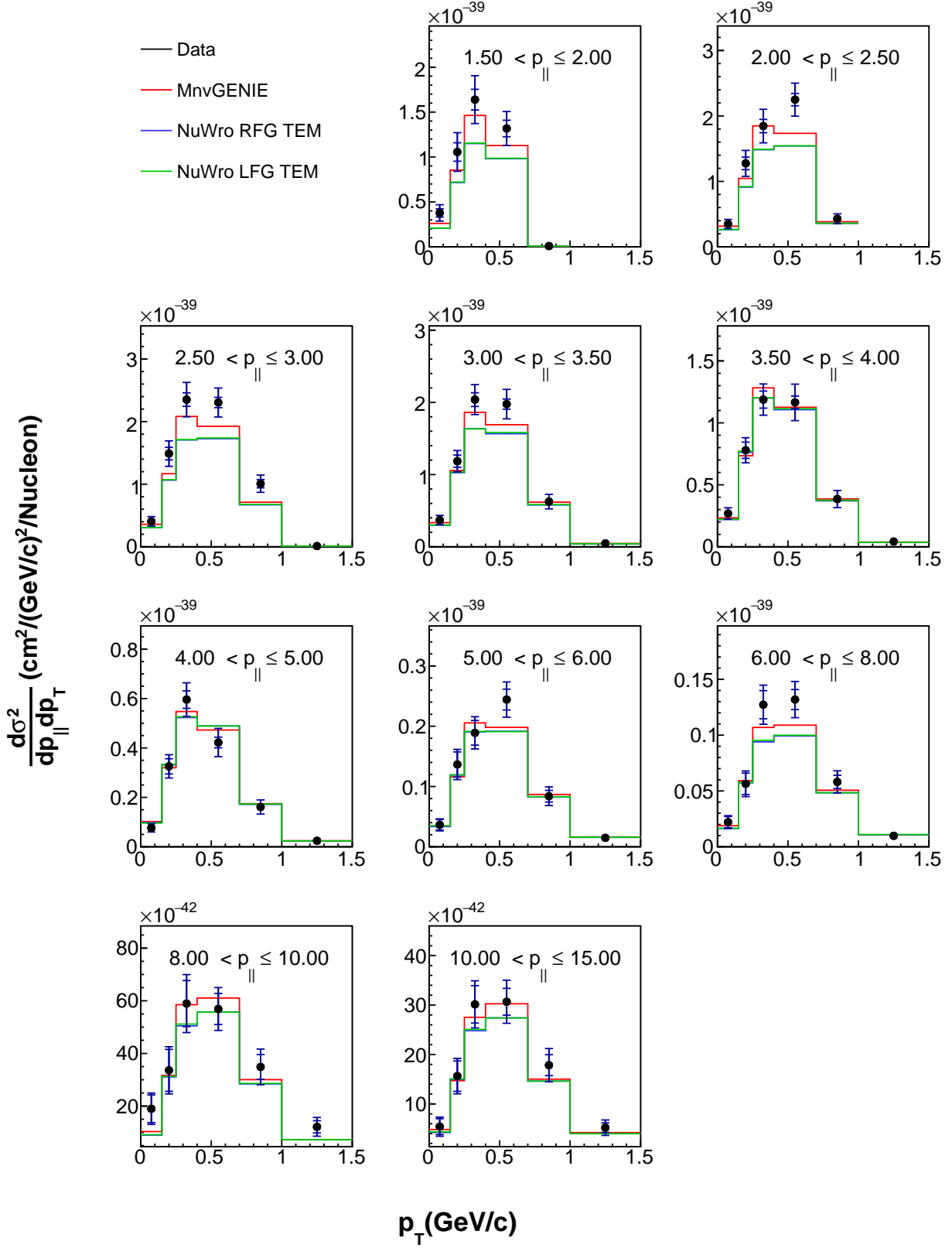
FIG. 21: Double-differential QE-like cross section vs. muon transverse momentum, in bins of muon longitudinal momentum compared to the MINERvA-tuned GENIE (red curve) and the NuWro Relativistic (RFG) Fermi Gas model with Transverse Enhancement (RFG+TEM, blue curve) and the NuWro Local Fermi Gas (LFG) model with Transverse Enhancement (LFG+TEM, green curve). Inner error bars show statistical uncertainties; outer error bars show total (statistical and systematic) uncertainty.
