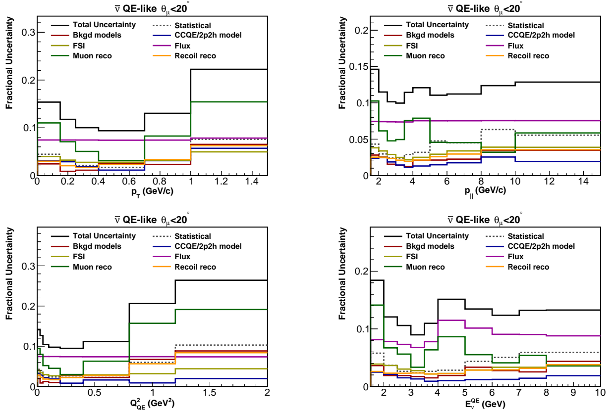
FIG. 26: Summary of fractional uncertainties on the single-differential projections of the double-differential QE-like cross section measurements in data. The cross sections themselves are shown in Fig. 18.
