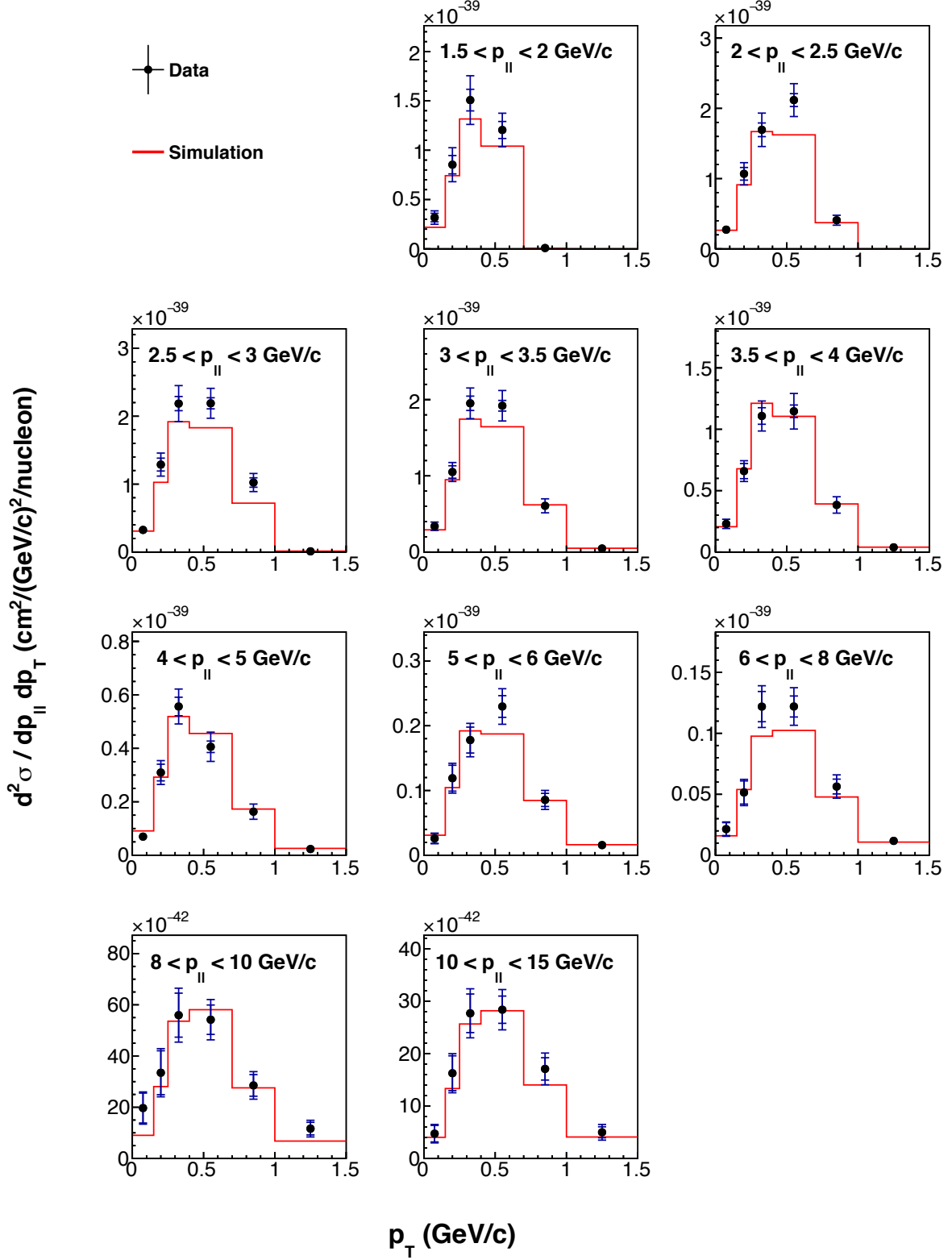
FIG. 30: Double-differential flux-integrated true CCQE cross section d^2\sigma/dp_T dp_{\parallel} vs. muon transverse momentum, in bins of muon longitudinal momentum. Inner error bars show statistical uncertainties; outer error bars show total (statistical and systematic) uncertainty. These results are tabulated in Tables XXII–XXIV.
