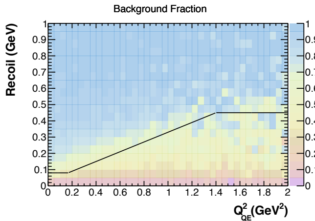
FIG. 4: Simulated QE-like background fraction before the recoil cut, in bins of Q^2 and recoil energy. The line shows the Q^2 dependent recoil energy selection used to optimize efficiency and purity.
