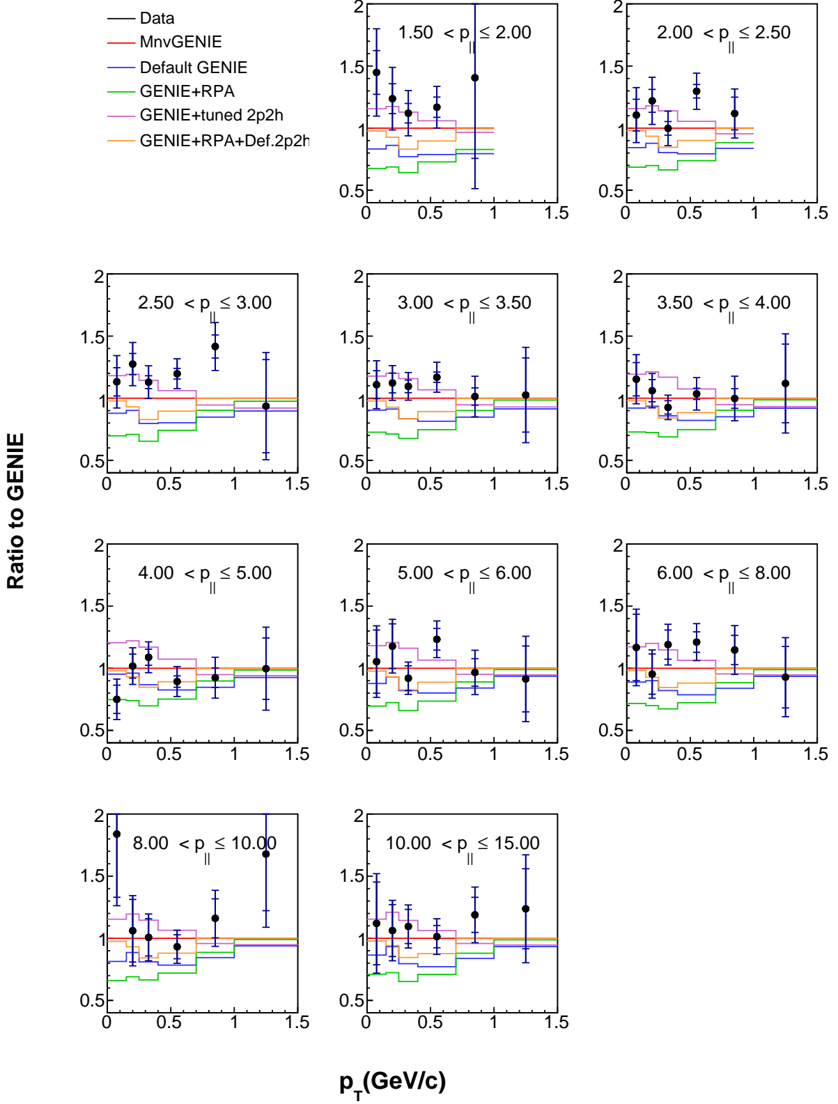
FIG. 19: Ratio of the double-differential QE-like cross sections vs. muon transverse momentum shown in the previous figure, in bins of muon longitudinal momentum. In all cases, the denominator for the ratio is MINERvA-tuned GENIE (includes RPA and MINERvA-tuned 2p2h); the numerators are our measured cross section (black circles), MINERvA-tuned GENIE (red), GENIE without any modifications (blue), GENIE with the RPA weight but no 2p2h component (green), GENIE with MINERvA-tuned 2p2h but no RPA (violet), and GENIE with RPA and untuned 2p2h (orange). Inner error bars show statistical uncertainties; outer error bars show total (statistical and systematic) uncertainty.
