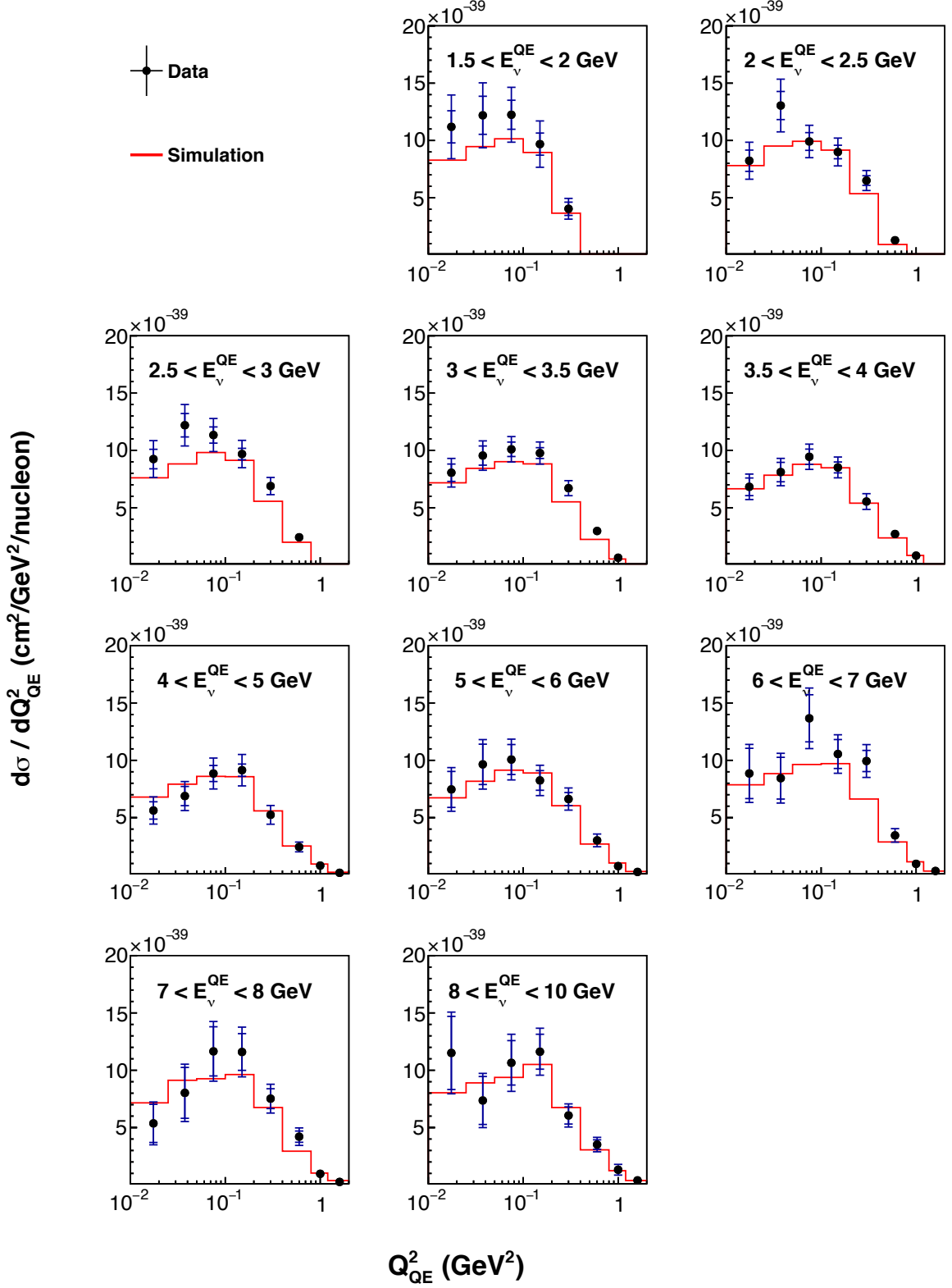
FIG. 14: Differential QE-like cross section d\sigma(E_{\nu}^{\text{QE}})/dQ_{\text{QE}}^2 , in bins of E_{\nu}^{\text{QE}} . Inner error bars show statistical uncertainties; outer error bars show total (statistical and systematic) uncertainty. The red histogram shows the MINERvA-tuned GENIE model used to estimate smearing and acceptance. These results are tabulated in Tables XII–XIV.
