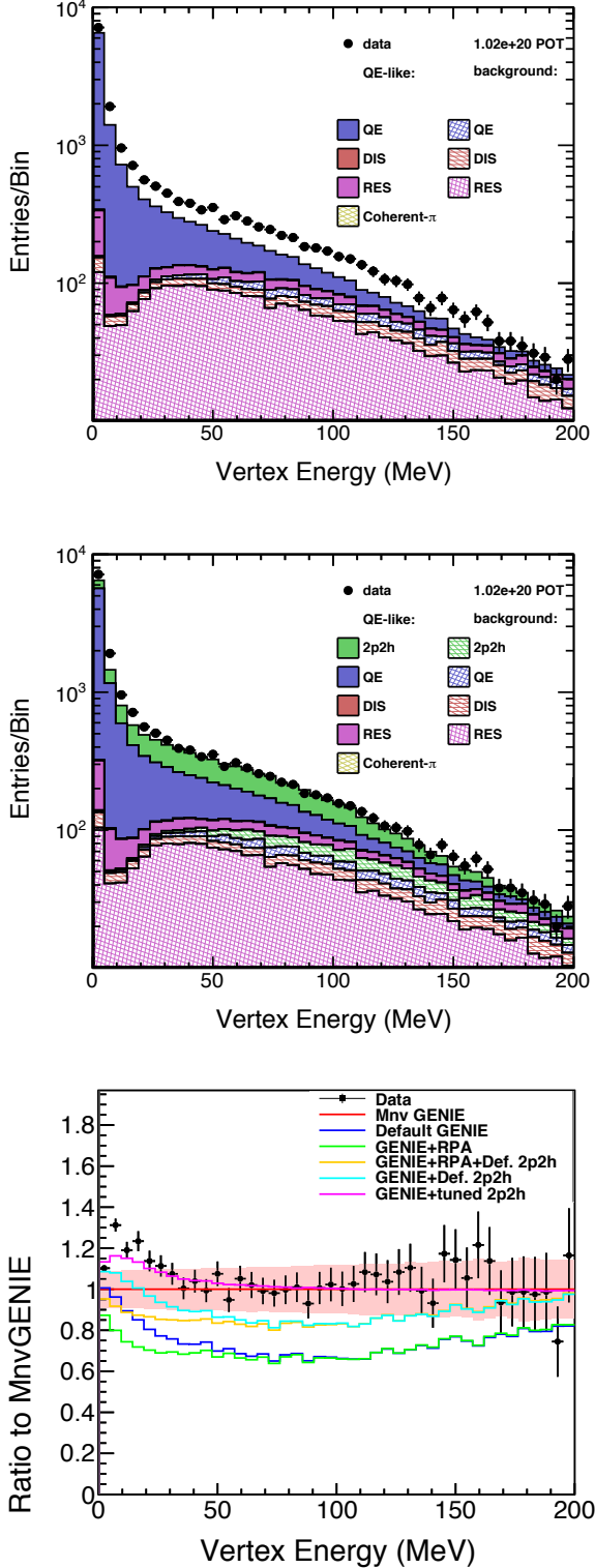
FIG. 25: Reconstructed energy within 100 mm of the neutrino interaction vertex. The black points show MINERvA data. In the top plot, the stacked histograms show the predictions of various models using default GENIE 2.8.4. In the middle plot, the stacked histograms are for the MINERvA-tuned GENIE 2.8.4, which includes RPA and MINERvA-tuned 2p2h. The bottom plot shows the ratio of the data and various models to MINERvA-tuned GENIE. Statistical uncertainties only.
