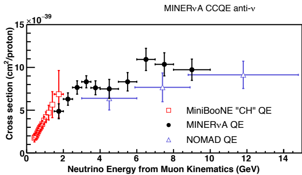
FIG. 23: MINERvA true CCQE cross section as a function of E_{\nu}^{QE} compared to data from the MiniBooNE and NOMAD experiments. Error bars show total (statistical and systematic) uncertainty.
