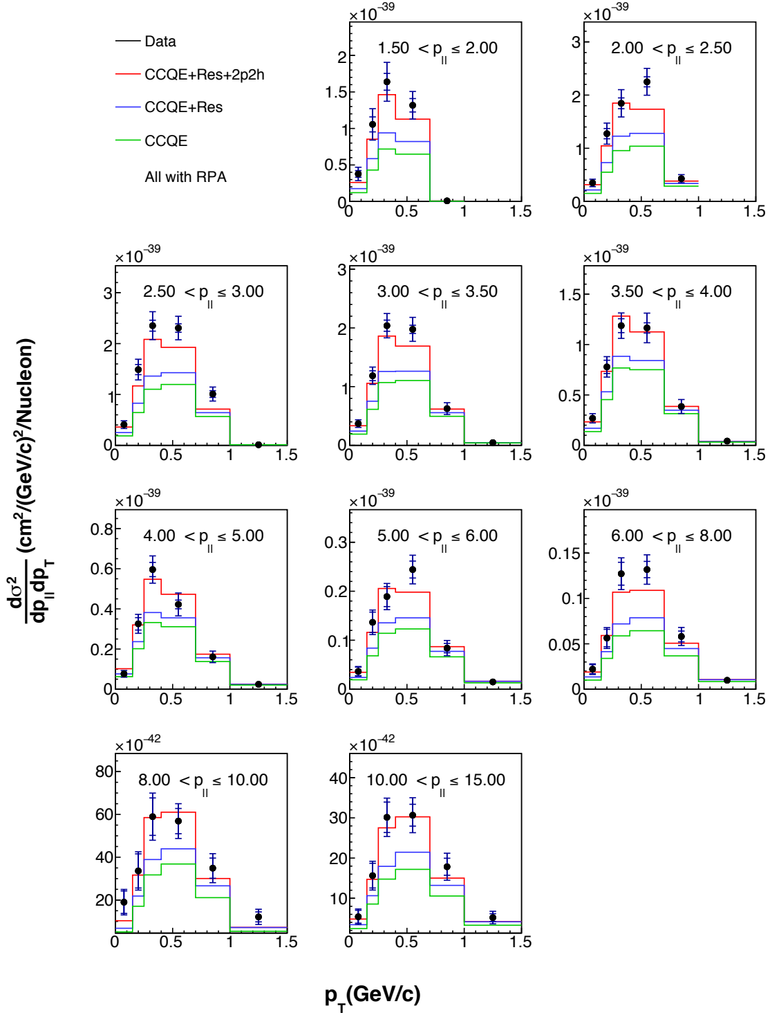
FIG. 16: Double-differential QE-like cross section vs. muon transverse momentum, in bins of muon longitudinal momentum. Inner error bars show statistical uncertainties; outer error bars show total (statistical and systematic) uncertainty. The red histogram shows the MINERvA-tuned GENIE 2.8.4 model used to estimate smearing and acceptance which is CCQE + resonant + 2p2h. The green histogram shows events produced as CCQE, the blue curve shows default GENIE which is CCQE + resonant. These results are tabulated in Tables VII–IX and the models are included in the supplementary material.
