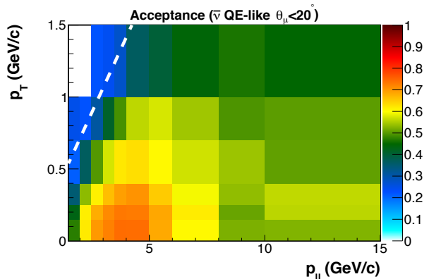
FIG. 11: Efficiency \times acceptance versus generated p_T and p_{||} , for QE-like events in the simulation. The dashed white line illustrates the 20 degree limit imposed on reconstructed muon angles.
