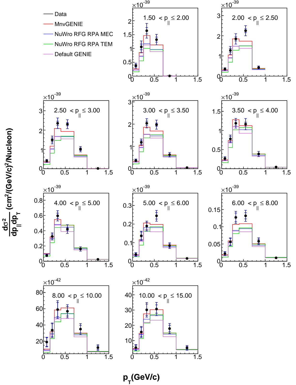
FIG. 20: Double-differential QE-like cross section vs. muon transverse momentum, in bins of muon longitudinal momentum compared to the MINERvA-tuned GENIE (red curve), the NuWro Nieves RFG model with Random Phase Approximation and Meson Exchange current (MEC) (blue curve) and the NuWro Relativistic Fermi Gas RFG model with RPA and Transverse Enhancement added (green curve). Inner error bars show statistical uncertainties; outer error bars show total (statistical and systematic) uncertainty.
