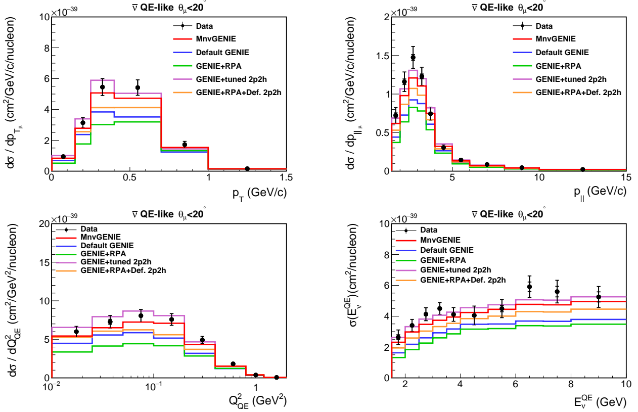
FIG. 32: Single-differential projections of the double-differential true CCQE cross section measurements in data, compared to MINERvA-tuned GENIE (red curve, includes RPA and MINERvA-tuned 2p2h), GENIE without any modifications except the single non-resonant pion correction discussed in section IV (blue), GENIE with the RPA weight but no 2p2h component (green), GENIE with MINERvA-tuned 2p2h but no RPA (violet), and GENIE with RPA and untuned 2p2h (orange). Inner error bars show statistical uncertainties; outer error bars show total (statistical and systematic) uncertainty. These results are tabulated in Tables XXV, XXVI, XXX and XXXI.
