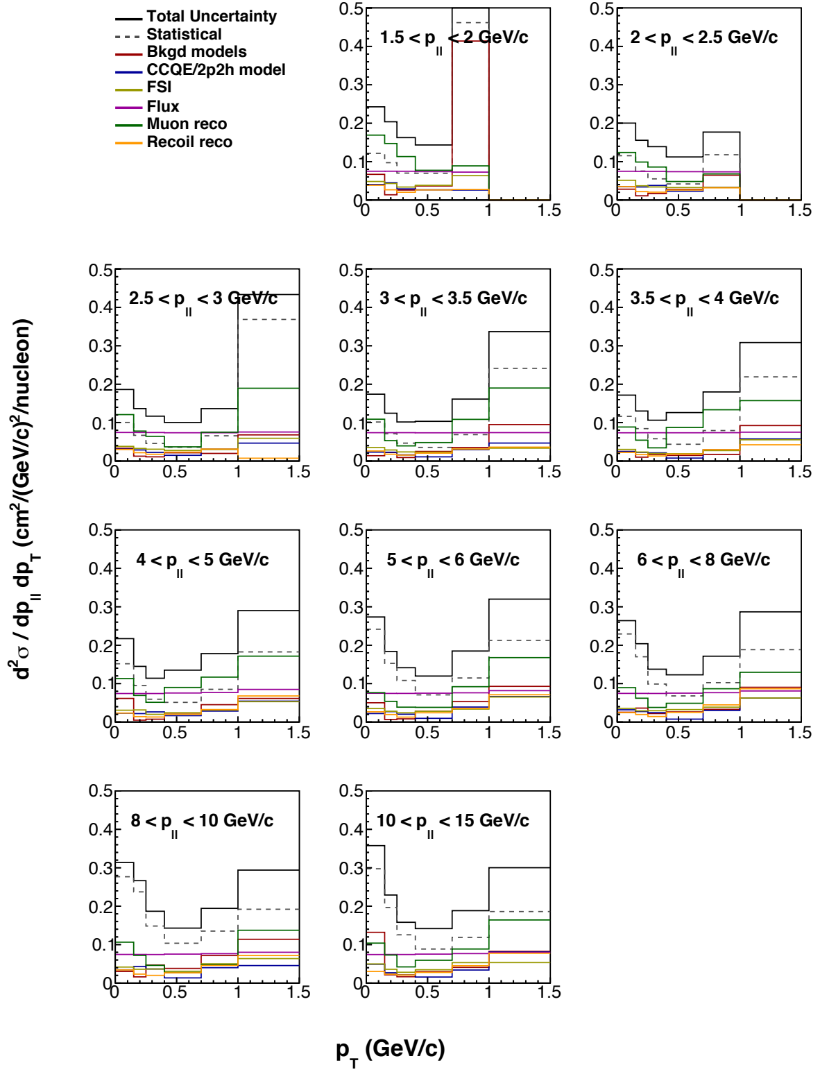
FIG. 27: Absolute fractional uncertainties on the double-differential QE-like cross section vs. muon transverse momentum, in bins of muon longitudinal momentum.
