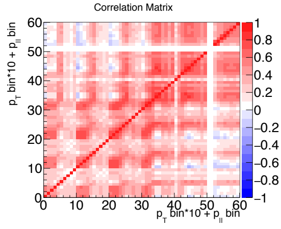
FIG. 29: Correlation matrix for the 6 \times 10 p_T and p_{||} bins. As in the migration matrix, the larger blocks are p_T bins with the smaller scale bins p_{||} bins.
