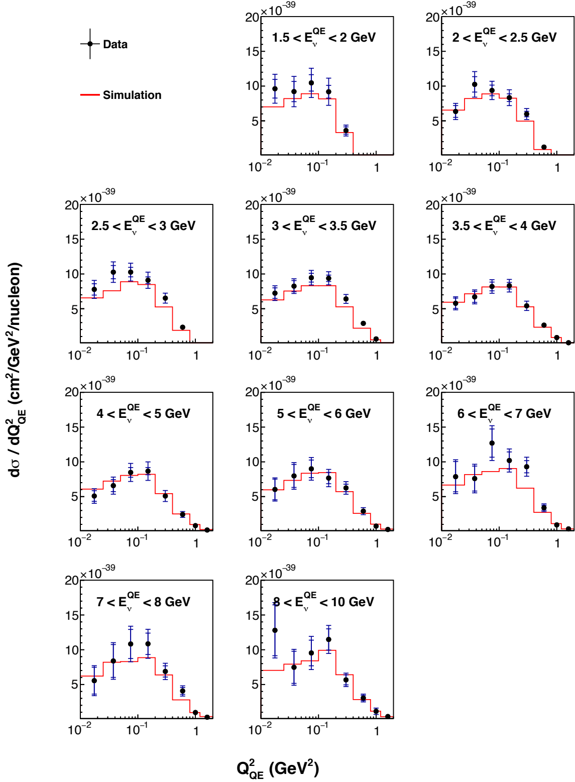
FIG. 31: True CCQE cross section d\sigma(E_{\nu}^{\text{QE}})/dQ_{\text{QE}}^2 , in bins of E_{\nu}^{\text{QE}} . Inner error bars show statistical uncertainties; outer error bars show total (statistical and systematic) uncertainty. These results are tabulated in Tables XXVII–XXIX.
