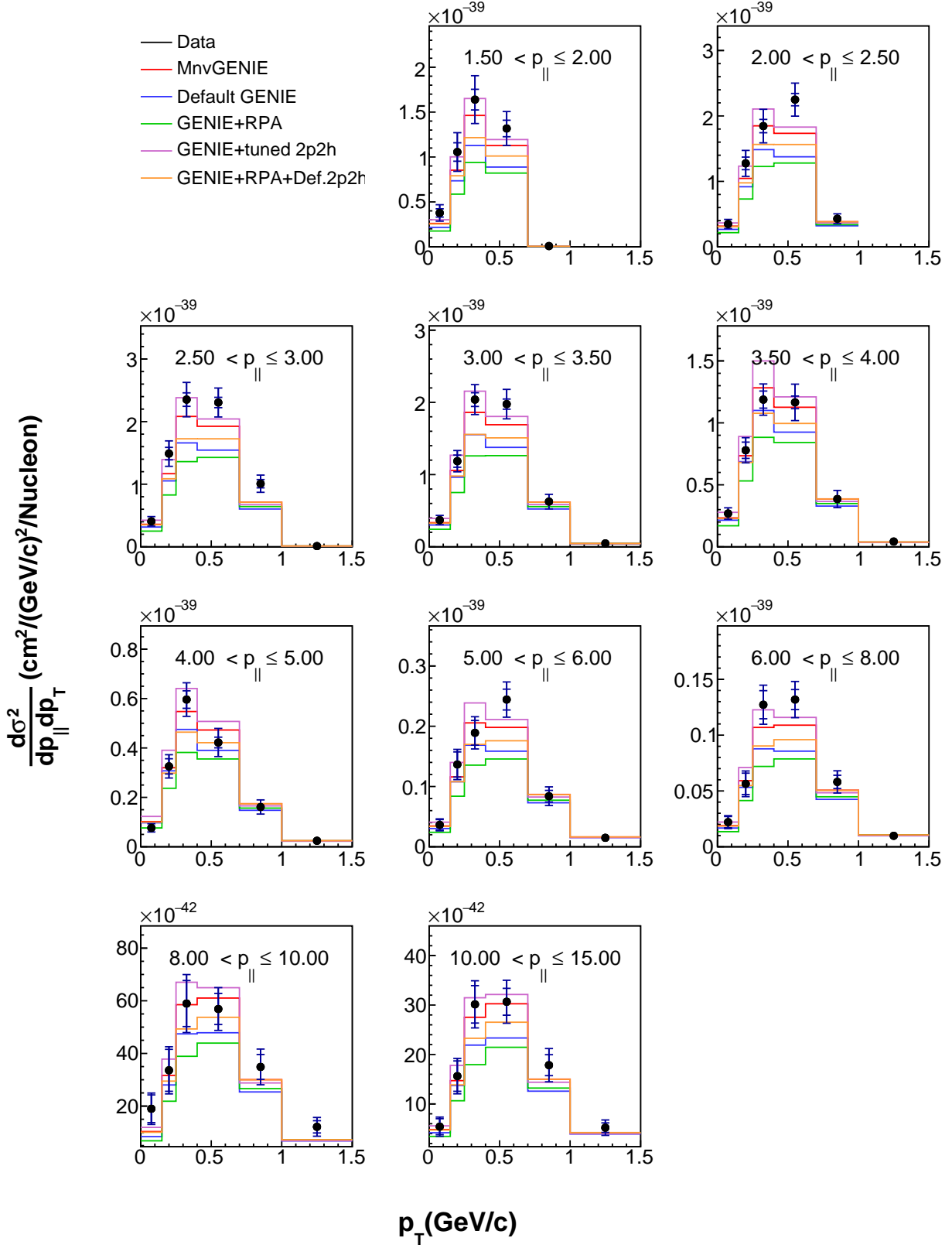
FIG. 17: Double-differential QE-like cross section vs. muon transverse momentum, in bins of muon longitudinal momentum (black circles) compared to MINERvA-tuned GENIE (red curve, includes RPA and MINERvA-tuned 2p2h), GENIE without any modifications except the single non-resonant pion correction discussed in section IV (blue), GENIE with the RPA weight but no 2p2h component (green), GENIE with MINERvA-tuned 2p2h but no RPA (violet), and GENIE with RPA and untuned 2p2h (orange). Inner error bars show statistical uncertainties; outer error bars show total (statistical and systematic) uncertainty.
