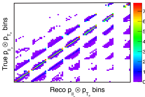
FIG. 10: Migration matrix for the p_{||} \otimes p_T distribution. The x axis corresponds to reconstructed bins, the y to true. The large cells correspond to p_T bins while the small cells are the p_{||} bins within a p_T bin. The high p_T overflow bin is included.
