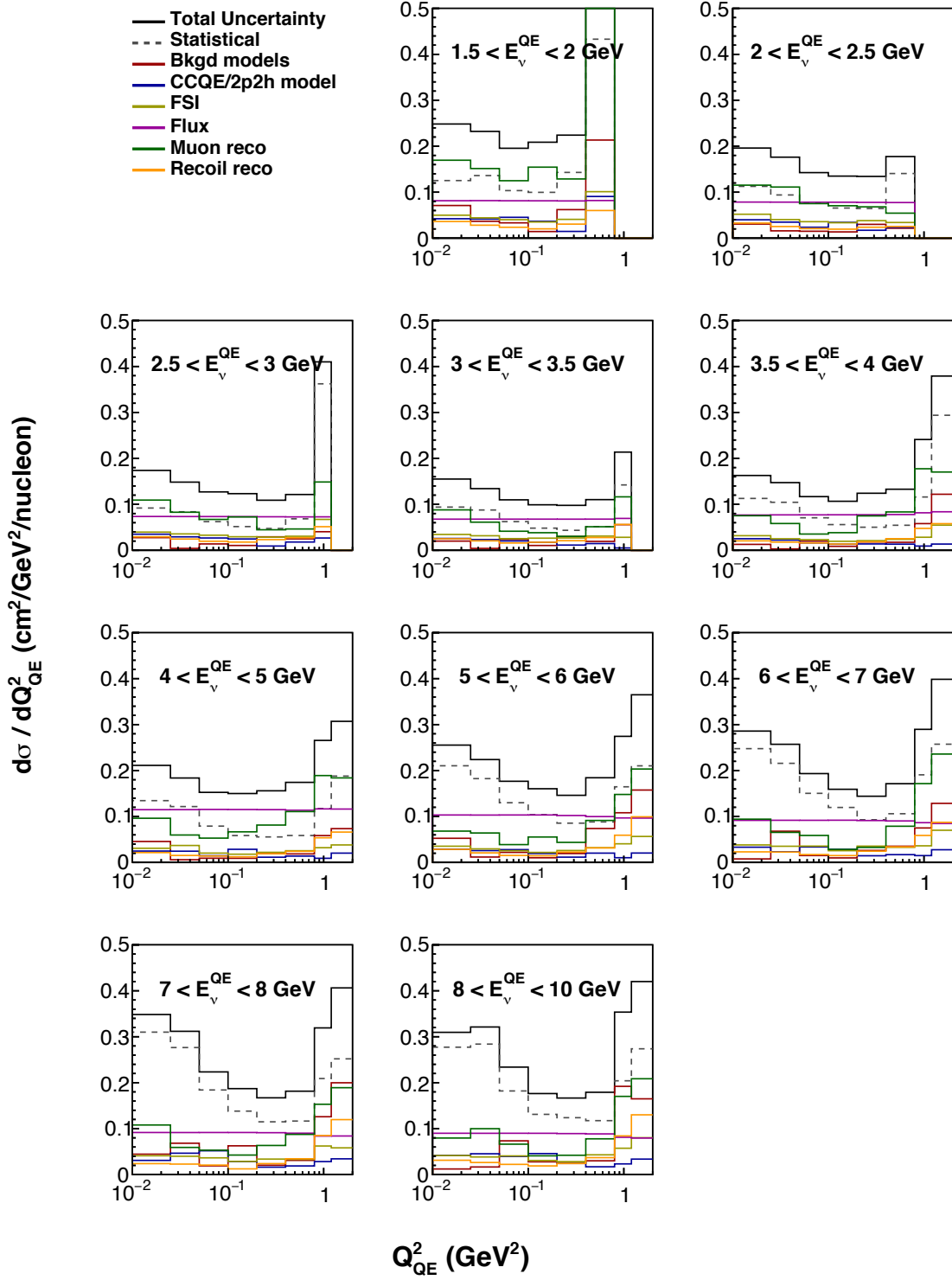
FIG. 28: Absolute fractional uncertainties on the cross section vs. Q^2 , in bins of E_{\nu}^{\text{QE}} .
