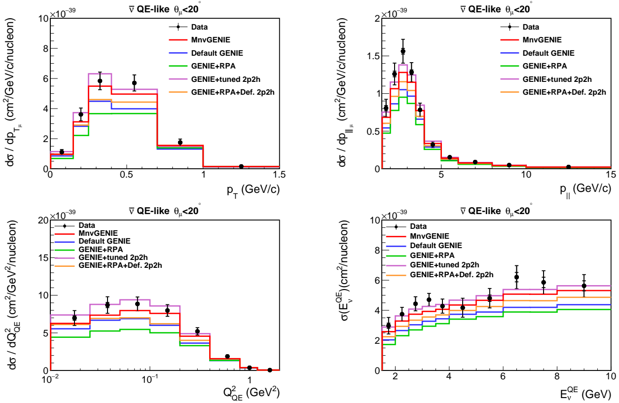
FIG. 18: Single-differential projections of the double-differential QE-like cross section measurements compared to MINERvA-tuned GENIE (red curve, includes RPA and MINERvA-tuned 2p2h), GENIE without any modifications except the single non-resonant pion correction discussed in section IV (blue), GENIE with the RPA weight but no 2p2h component (green), GENIE with MINERvA-tuned 2p2h but no RPA (violet), and GENIE with RPA and untuned 2p2h (orange). Inner error bars show statistical uncertainties; outer error bars show total (statistical and systematic) uncertainty. These results are tabulated in Tables X, XI, XV and XVI.
