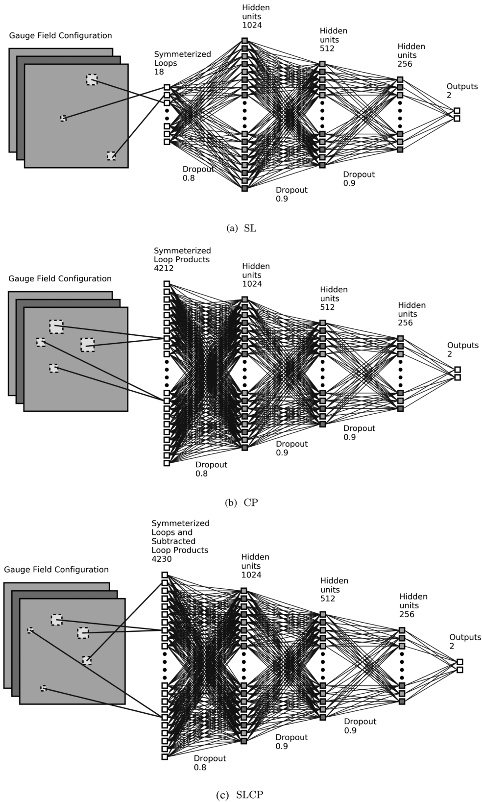
FIG. 13. Diagrams of the neural network structure used. In the first layer, SL , CP , or SLCP structures are formed, e.g., in the CP case, products of the 18 different types of loops separated by lattice distance R < 13 (averaged in integer space bins of R ) are allowed, for a total of 18 \times 18 \times 13 = 4212 loop products. The first layer is followed by 3 fully connected hidden layers with 1024, 512, and 256 nodes. Each hidden layer uses a \tanh activation function, with dropouts between layers.
